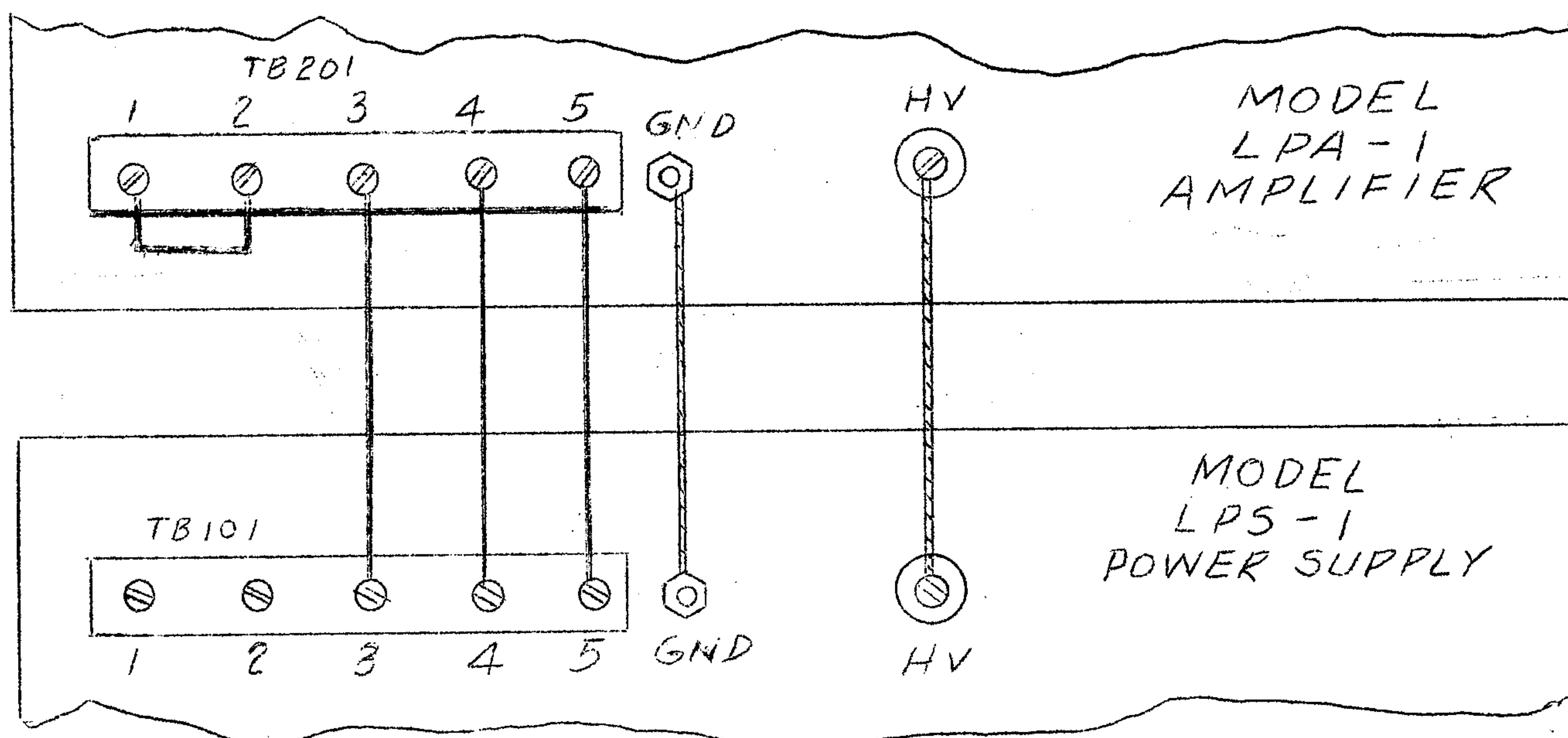
FIGURE 5A. CONNECTION OF LPA-1 TO LPS-1
