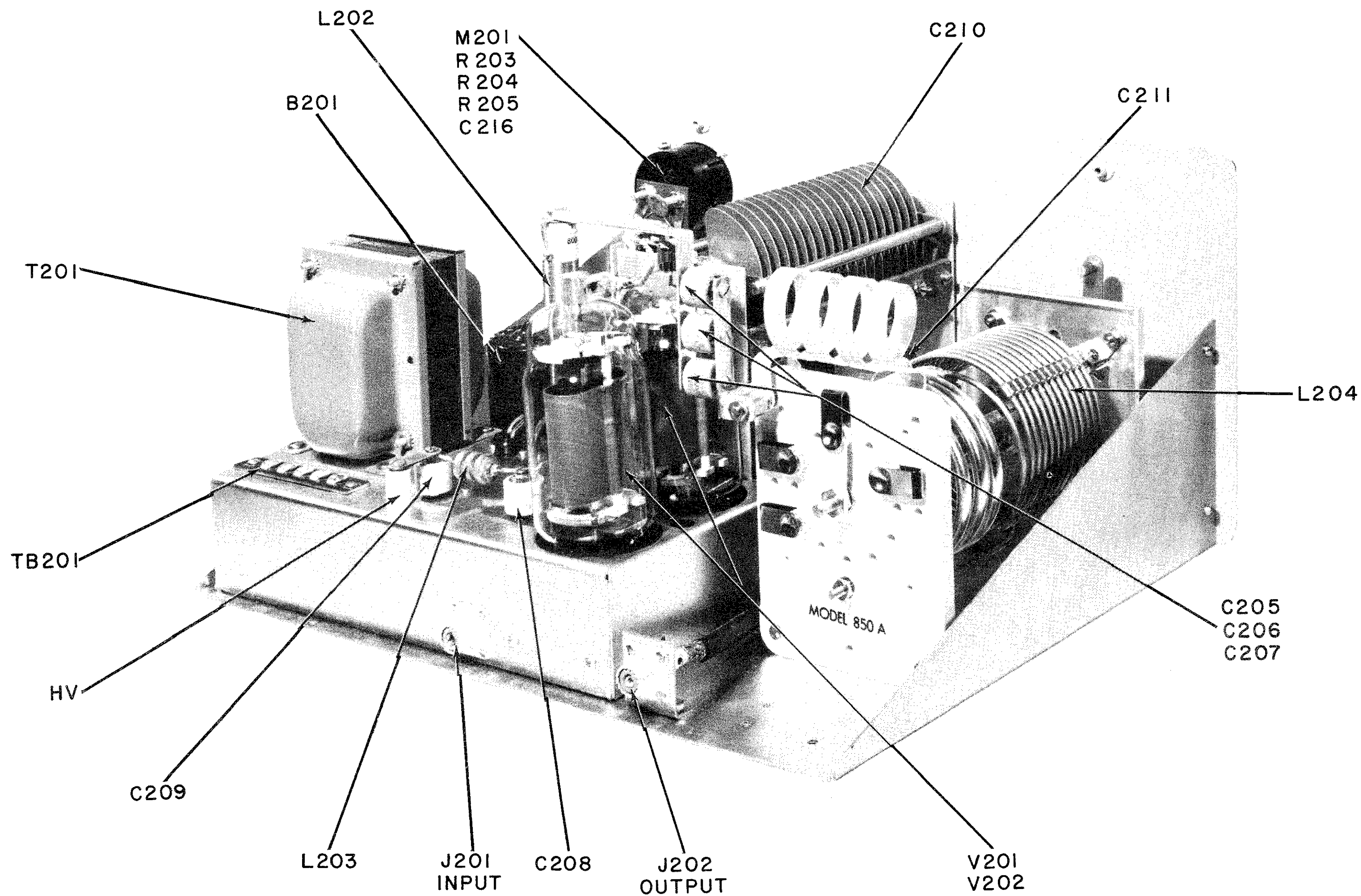
FIGURE 2. MODEL LPA-1 LINEAR POWER AMPLIFIER, TOP OF CHASSIS
