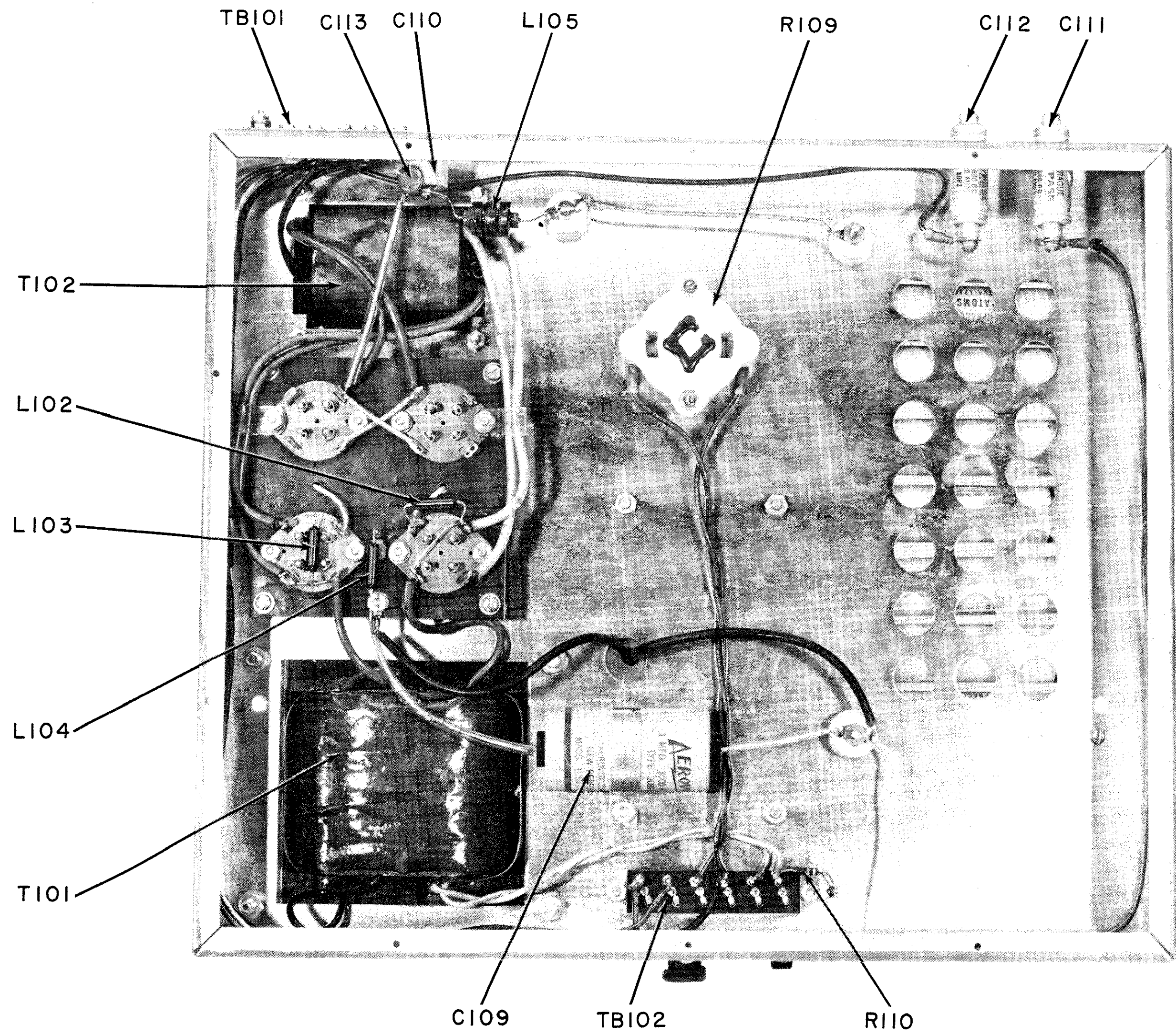
FIGURE 4. MODEL LPS-I POWER SUPPLY, BOTTOM OF CHASSIS
