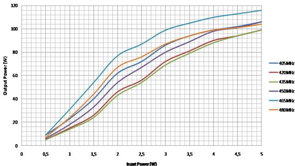
MUA100 UHF Wideband Amplifier
