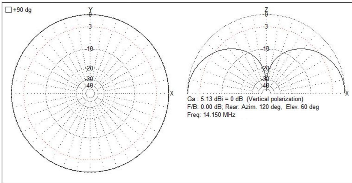
Figure 11. Portable Vertical Far Field Plot 14 MHz.
