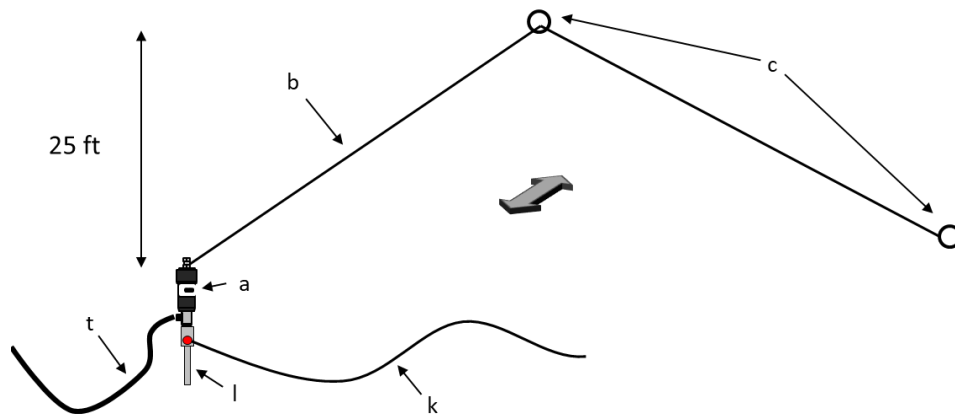
1. Select a site to deploy the CHA MPAS End-Fed Inverted “V” configuration. The site must have one center support, around 25 feet high and with 27 feet on each side for the ends of the antenna. If the right supports are unavailable, any convenient objects, such as fence posts or the tops of vehicles, may be used as a field expedient supports with reduced performance.
