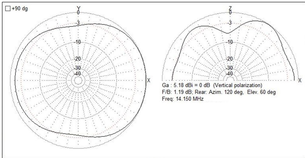
Figure 13. Sloping Wire Far Field Plot 14 MHz.
