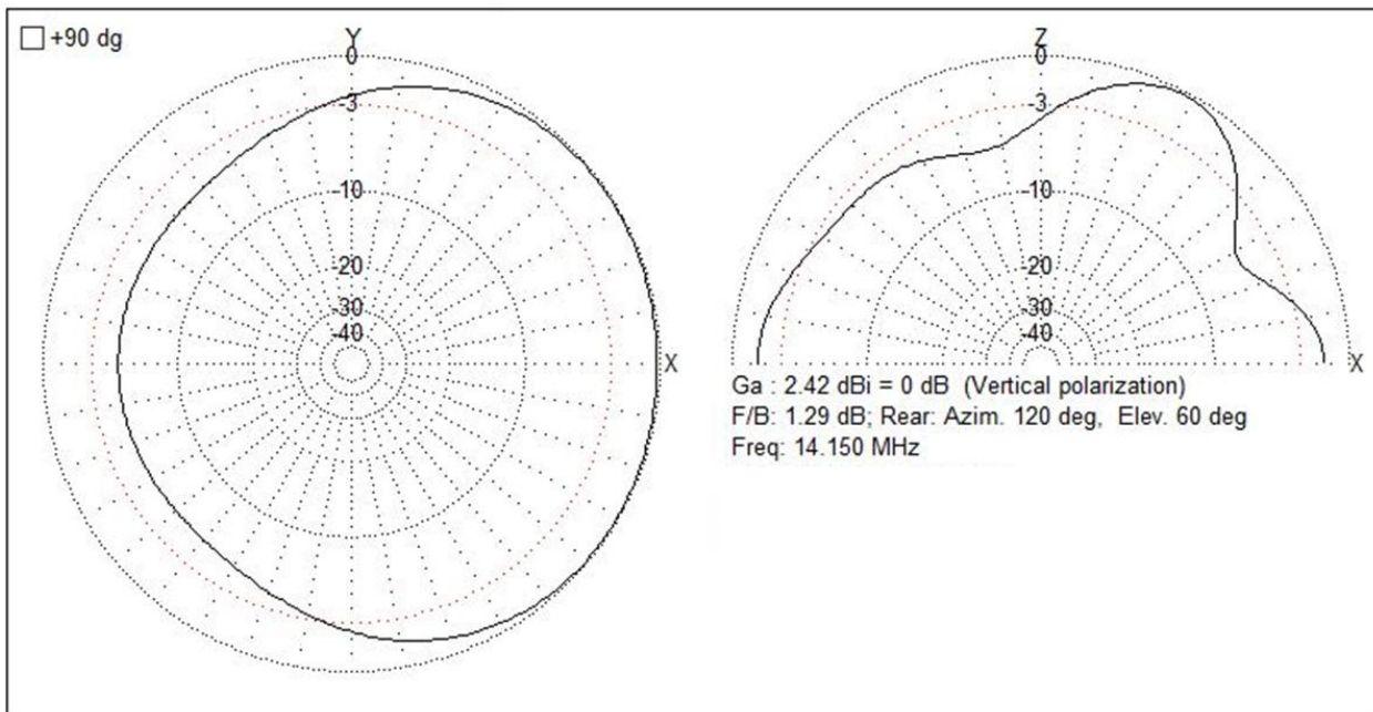
Figure 14. Inverted "L" Far Field Plot 14 MHz.
