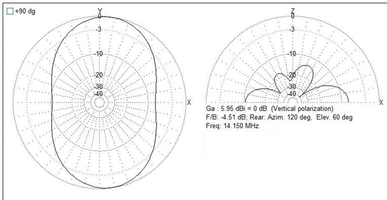
Figure 15. End-Fed Inverted "V" Far Field Plot 14 MHz.
