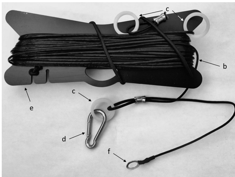
Plate 3. Antenna Wire Assembly.
