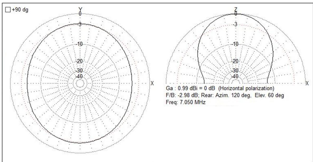
Figure 12. Horizontal NVIS Far Field Plot 7 MHz.
