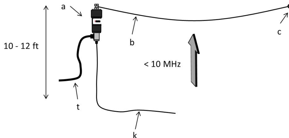
Figure 3. Horizontal NVIS Configuration.
