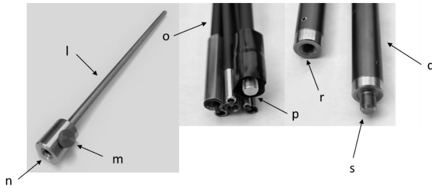
Plate 4. Whip Antenna and Spike Mount Connections.
