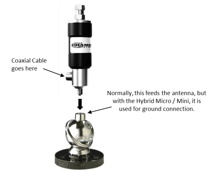
Plate (7). Hybrid Micro / Mini Electrical and Mechanical Connections.
