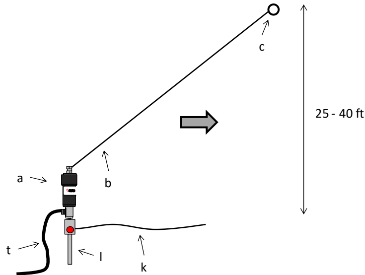
Figure 4. Sloping Wire Configuration.
