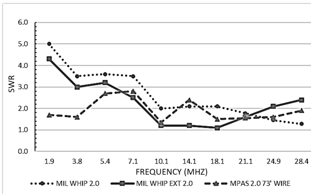
Figure 9. SWR by Frequency Graph.
