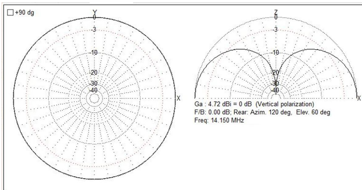
Figure 10. Manpack Vertical Far Field Plot 14 MHz.
