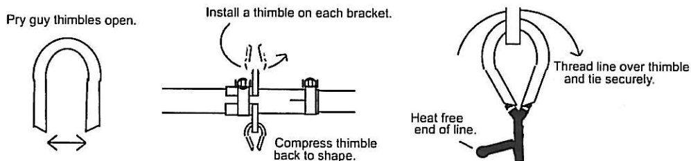
FIG-7B: Installing Thimbles and Guys
