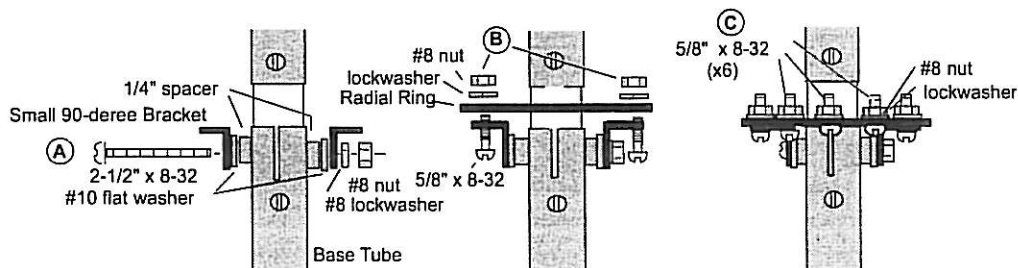
FIG-2: Ground Radial Ring Assembly
