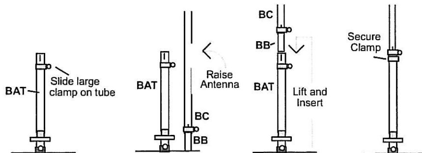
FIG-12A: Installing Antenna Radiator
