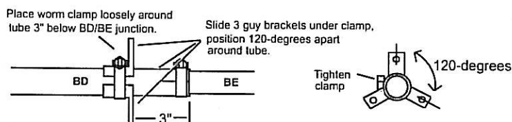
FIG-7A: Installation of Guy Brackets
