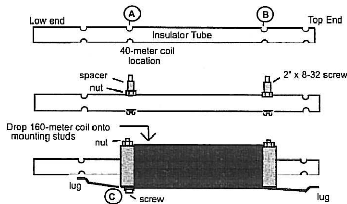
FIG-4: Mounting Loading Coil
