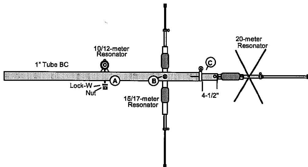
FIG 8: Mounting Resonators
