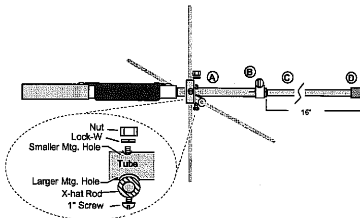
FIG 6: 20-Meter Resonator Assembly
