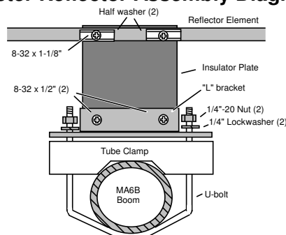
Six-Meter Reflector Assembly Diagram
