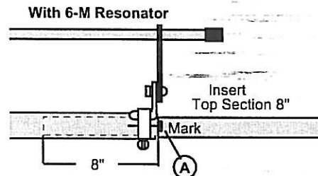
FIG 11: Joining antenna sections
