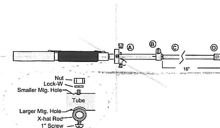
FIG 6: 20-Meter Resonator Assembly
