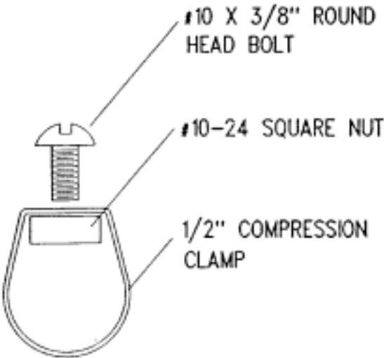
Figure 3 One-Half Inch Compression Clamp Detail
