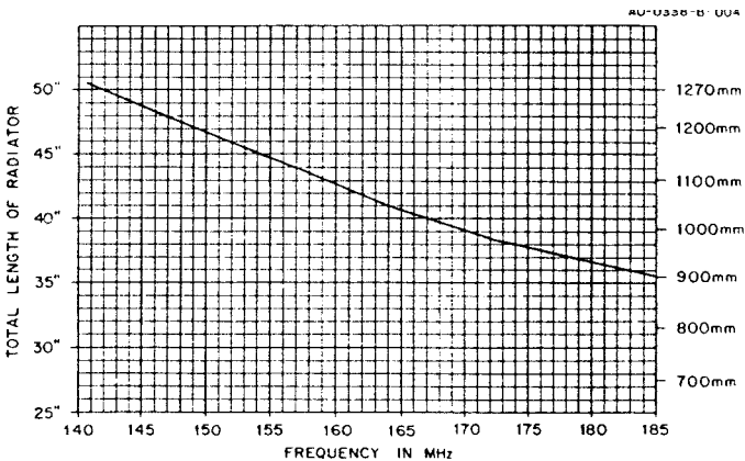
Figure 4 Frequency Adjustment Chart
