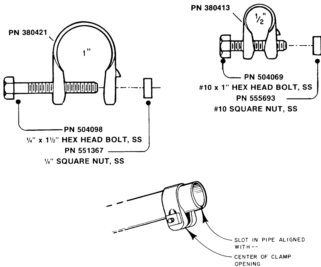
Figure 3 Compression Clamps
