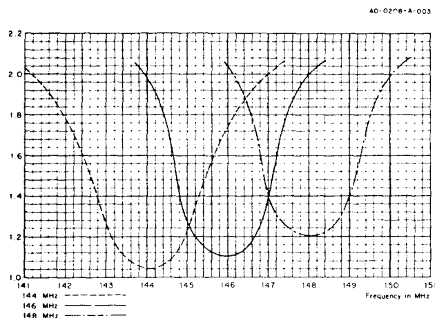
Figure 3A VSWR for Horizontal Polarization Only
