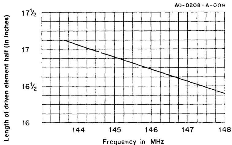
Figure 3B Driven Element Cutting Chart
