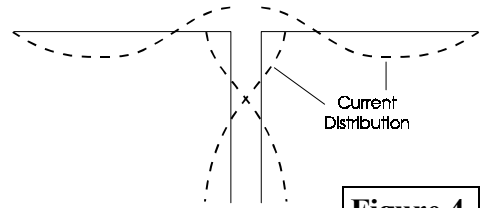
Current Distribution 14MHz
