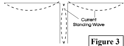
Current Distribution 10MHz
