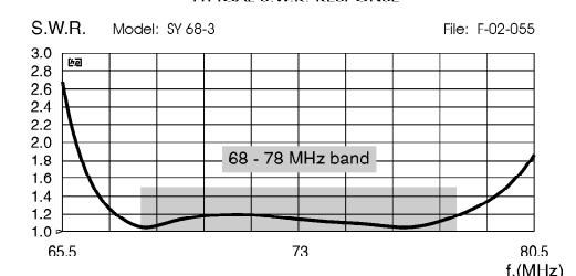
TYPICAL S.W.R. RESPONSE File: F-02-055
