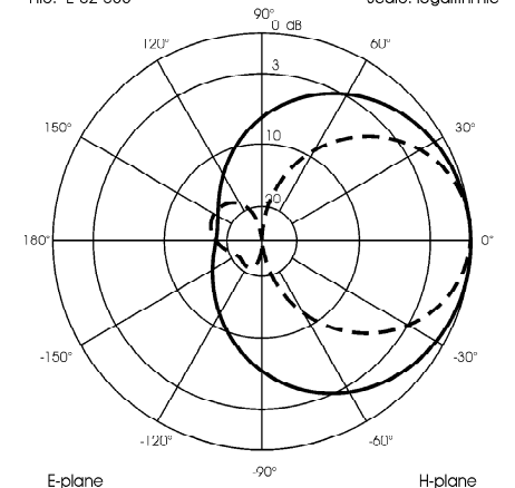
TYPICAL RADIATION PATTERN at 73 MHz File: E-02-055 Scale: logarithmic
