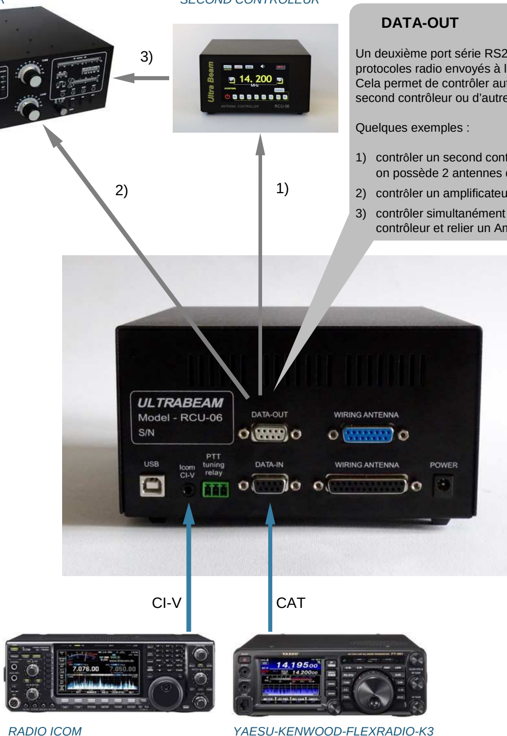
RADIO ICOM
