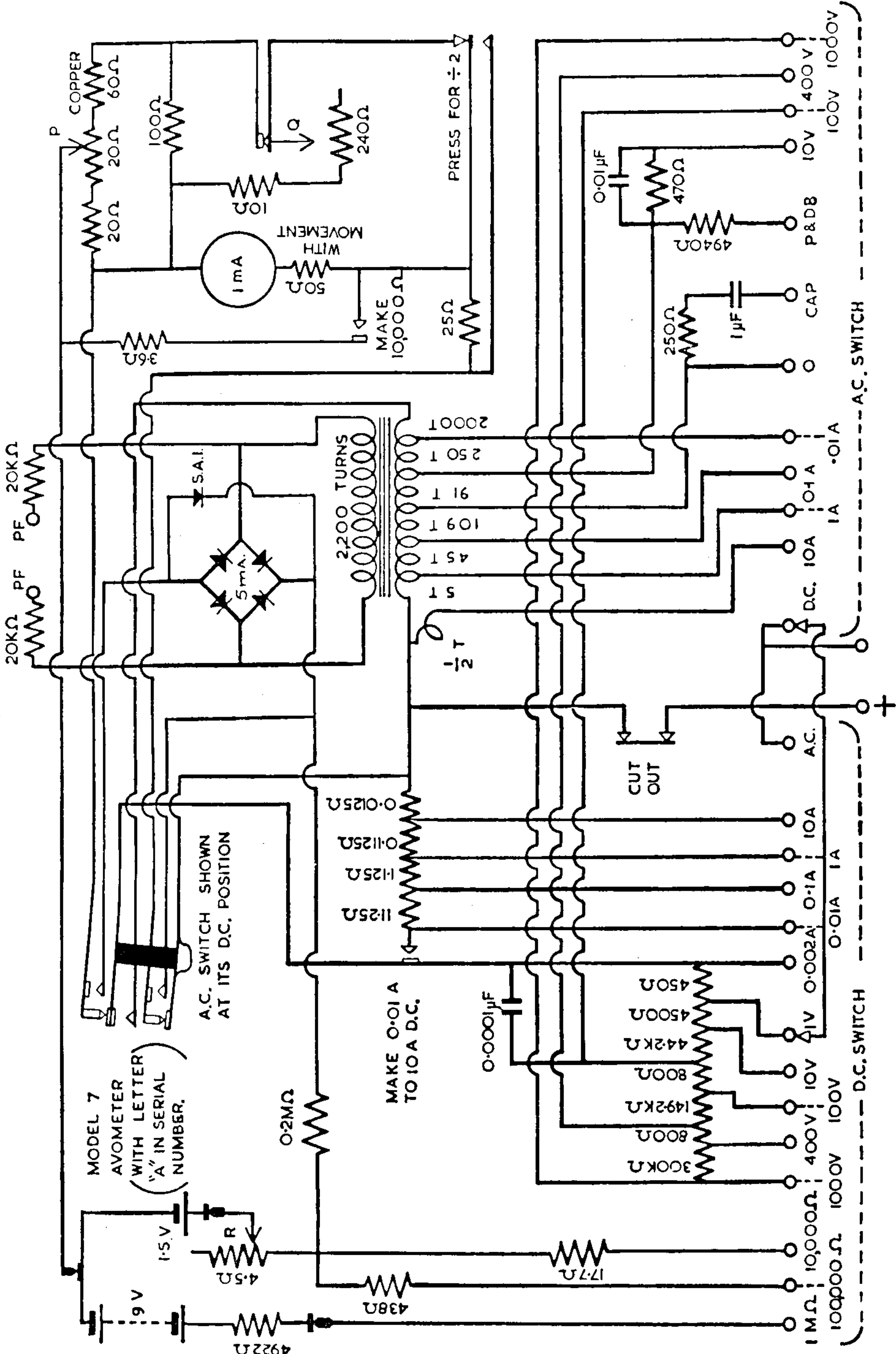
CIRCUIT DIAGRAM OF THE MODEL 7 AVOMETER MK. II
