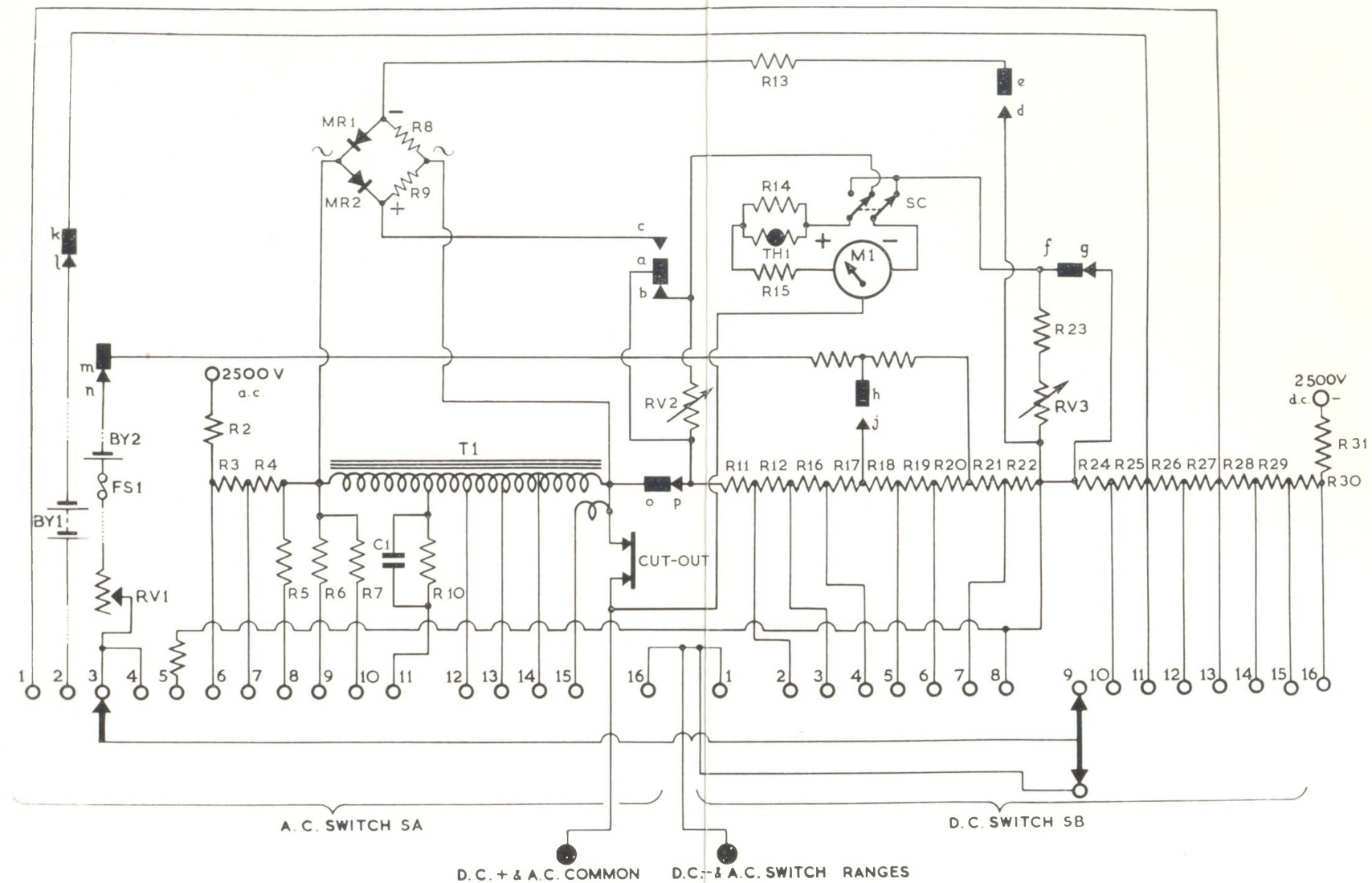
CIRCUIT DIAGRAM OF THE MODEL 8 MK. III AVOMETER
