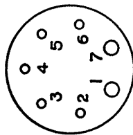
AMERICAN SMALL SEVEN PIN (SM7)
