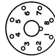
MAZDA OCTAL (MO8)
