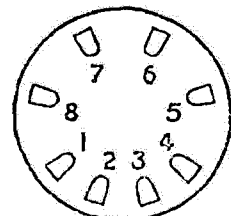
'P' TYPE BASE (8SC)
