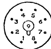
AMERICAN OCTAL (B8B or B8G)
