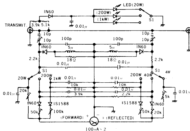
CN-620A Schematic Diagram
