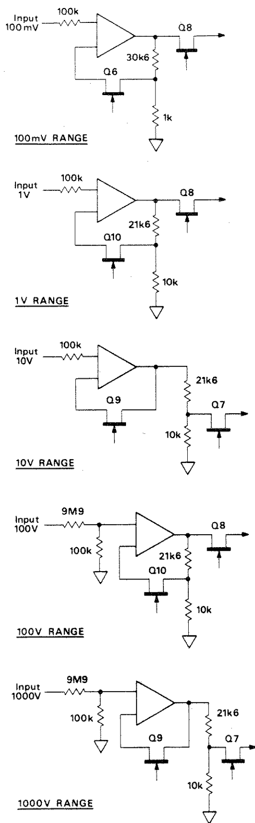
FIG. 3.9 PREAMPLIFIER GAIN CIRCUITS
