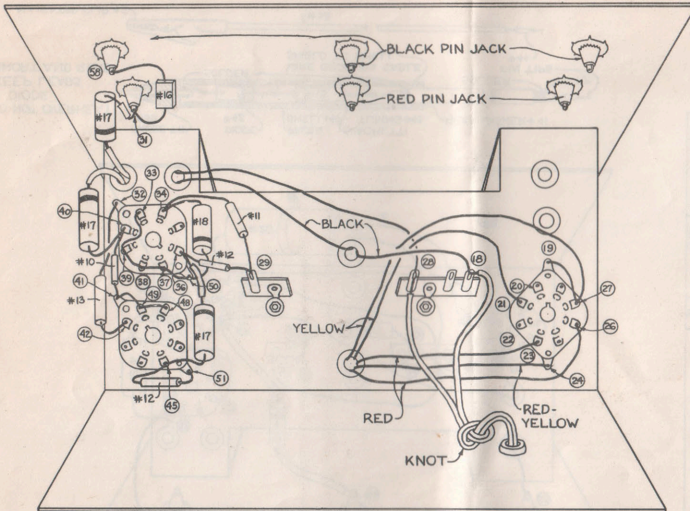
BOTTOM VIEW OF CHASSIS ASSEMBLY PRINT No.2
