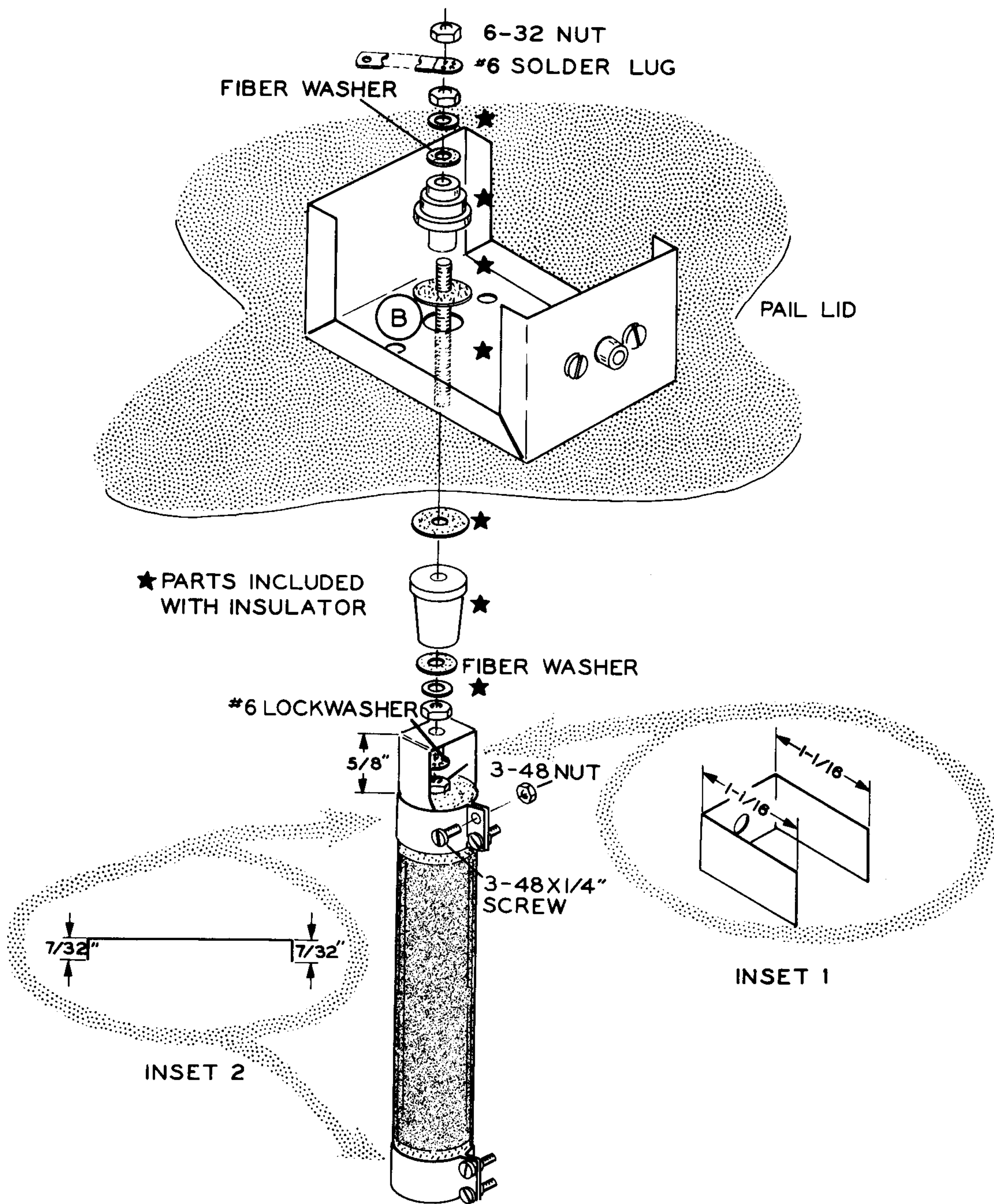
Pictorial 3
