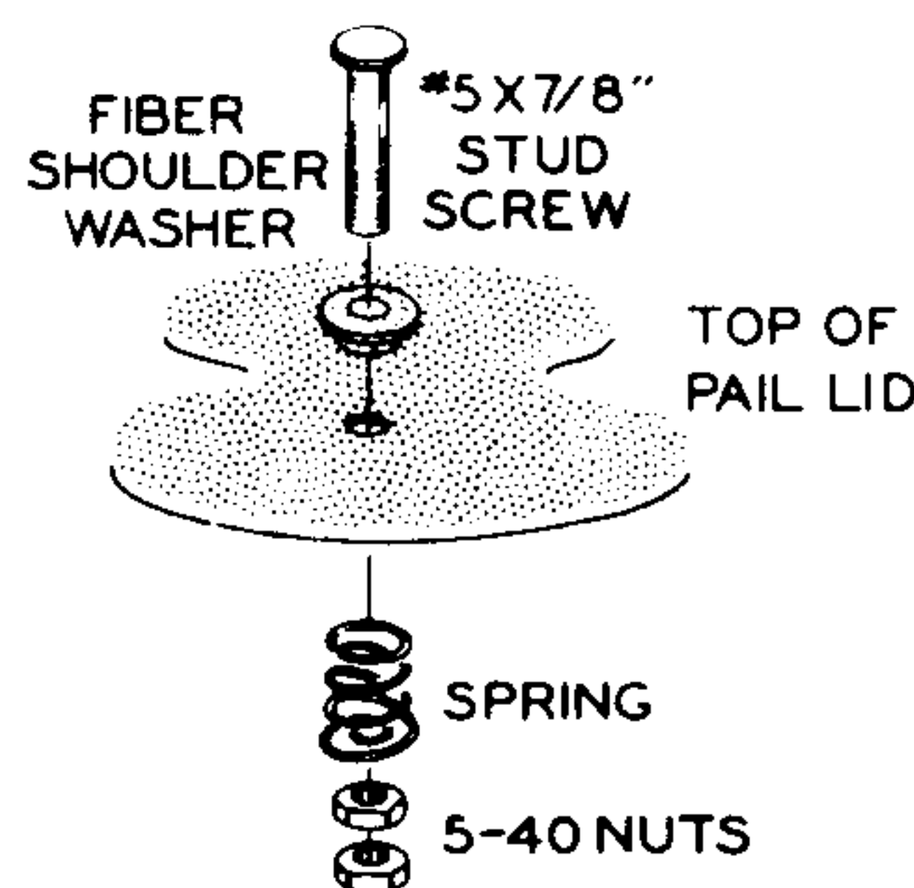
Detail 1D
