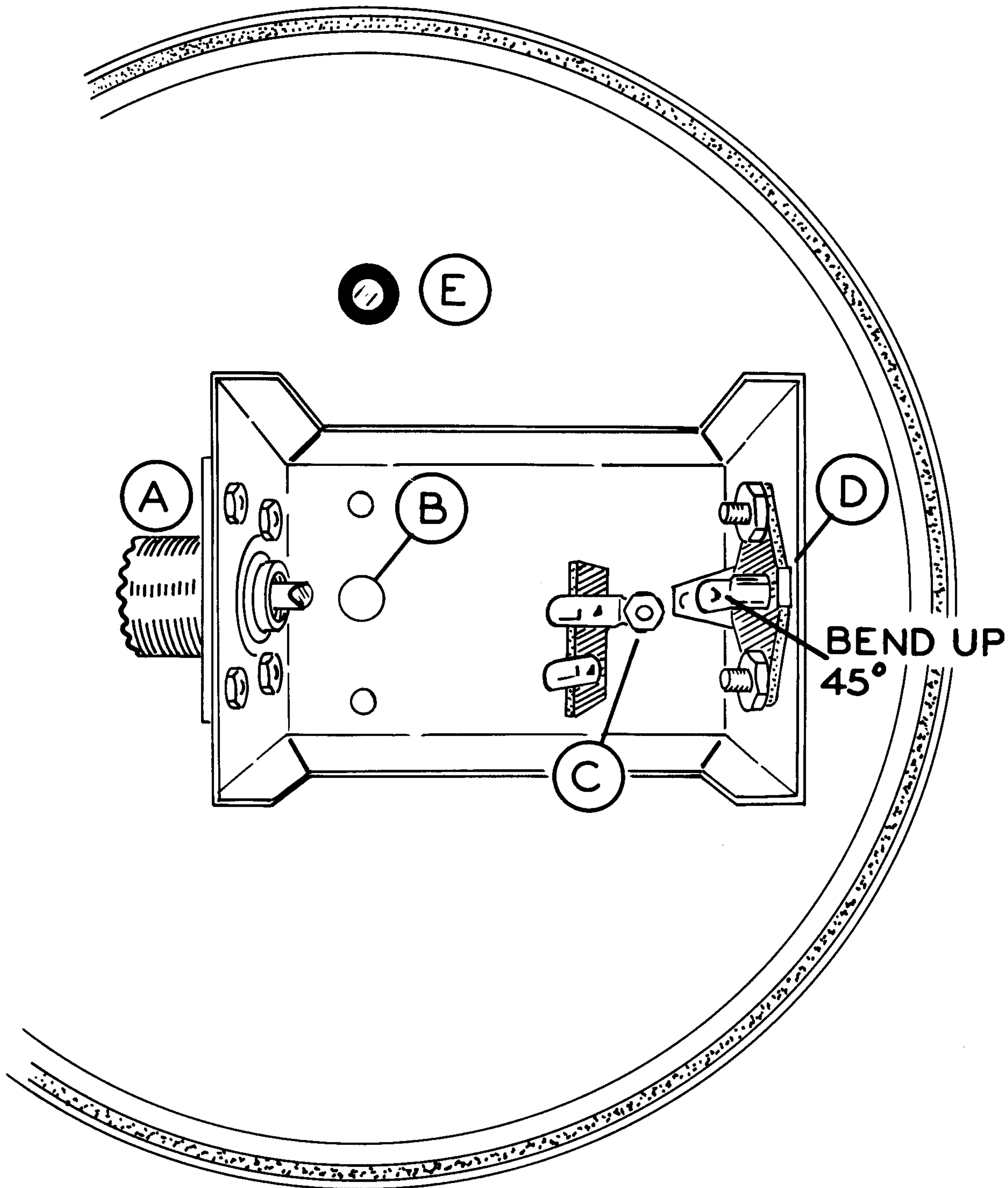
Pictorial 1
