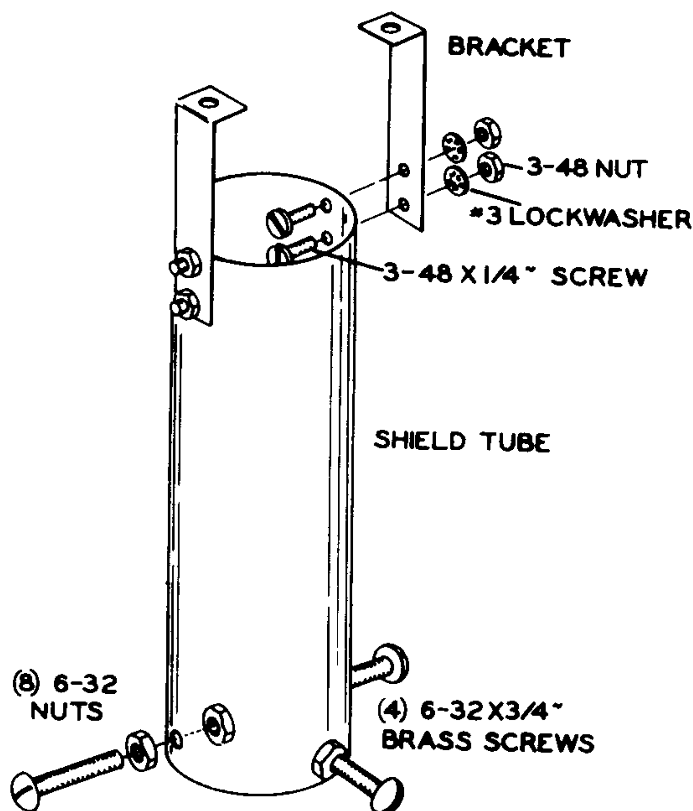
Pictorial 2
