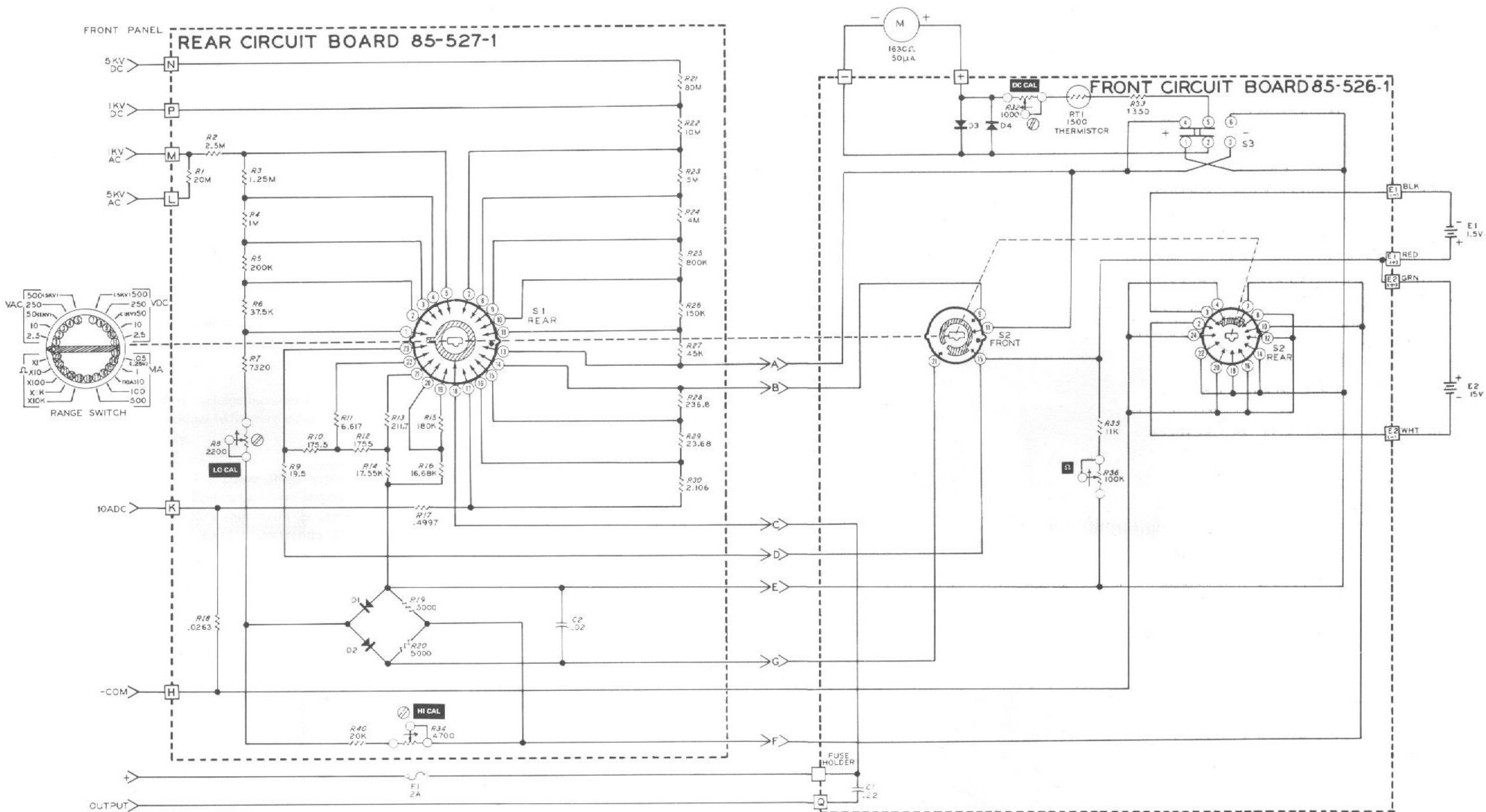
SCHEMATIC OF THE HEATHKIT® VOLT-OHM-MILLIAMMETER MODEL IM-105
