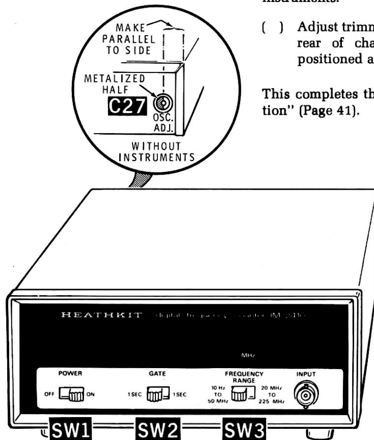
PICTORIAL 7-1
