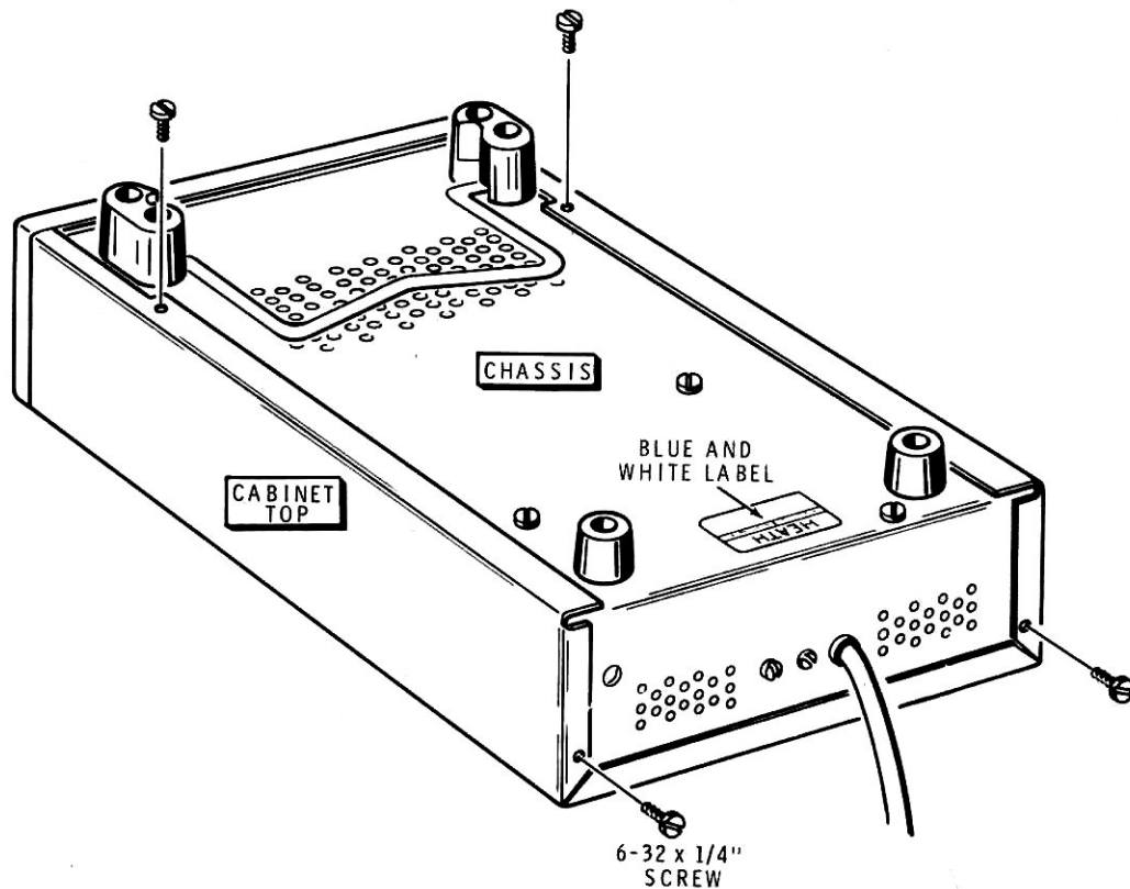
PICTORIAL 6-1
