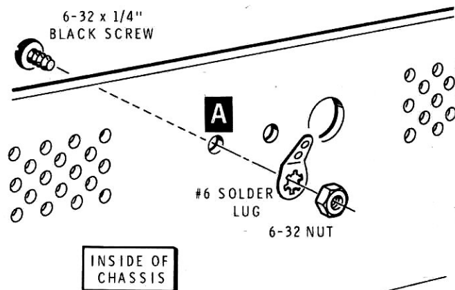
Detail 4-1B
