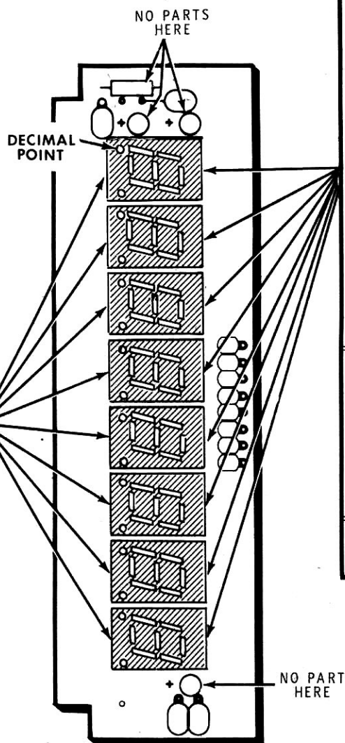
PICTORIAL 2-1
