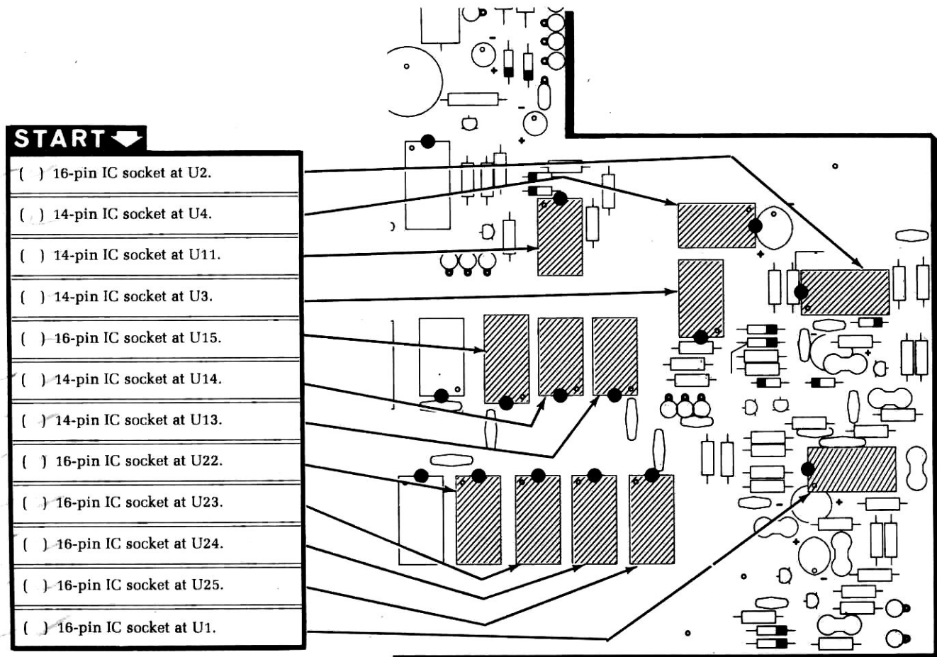
PICTORIAL 1-6
