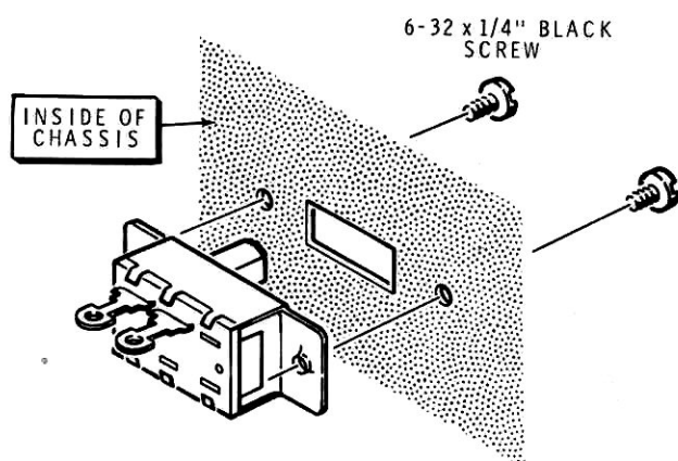
Detail 4-1A
