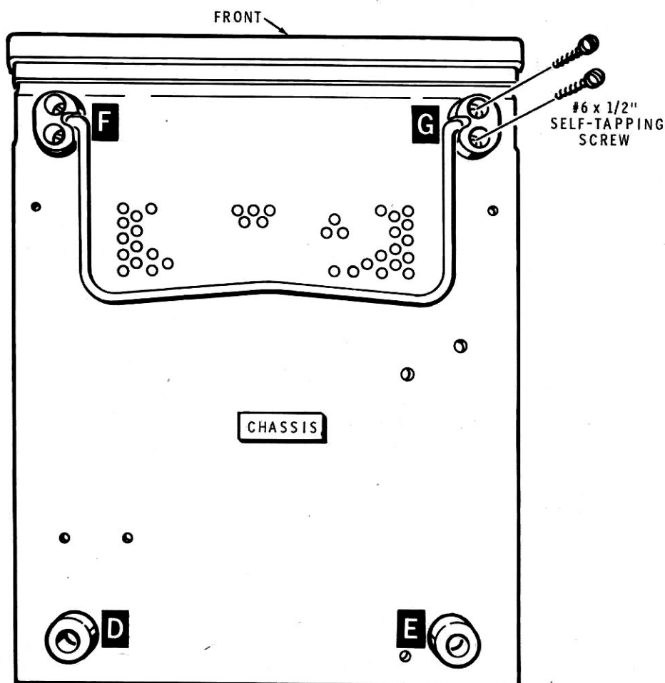
Detail 4-1D
