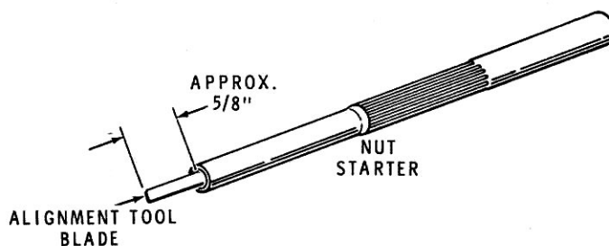
Detail 7-1A
