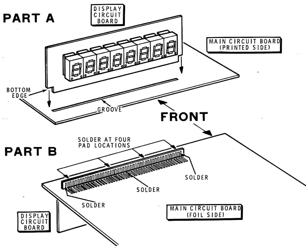
PICTORIAL 3-1
