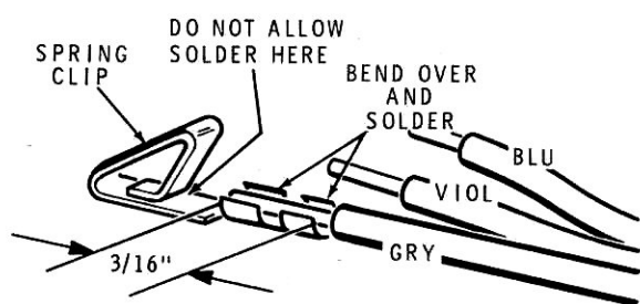
Detail 3-2C
