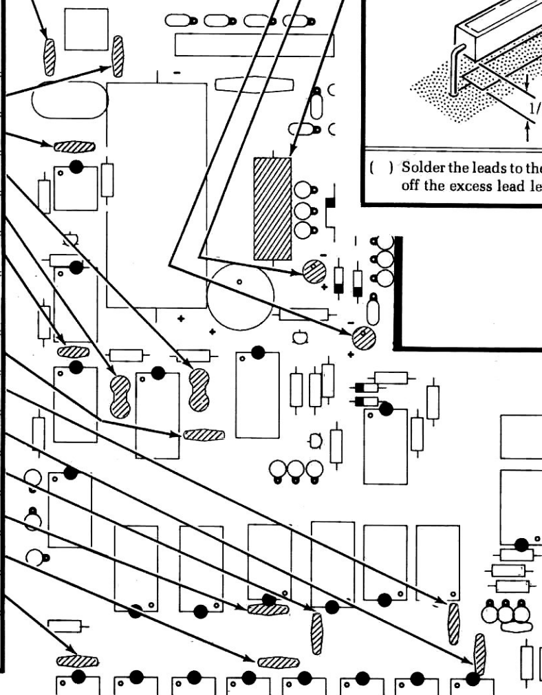
PICTORIAL 1-8
