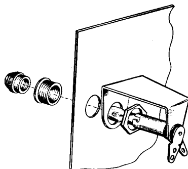
Detail 1D
