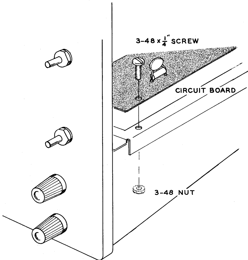
Detail 5A
