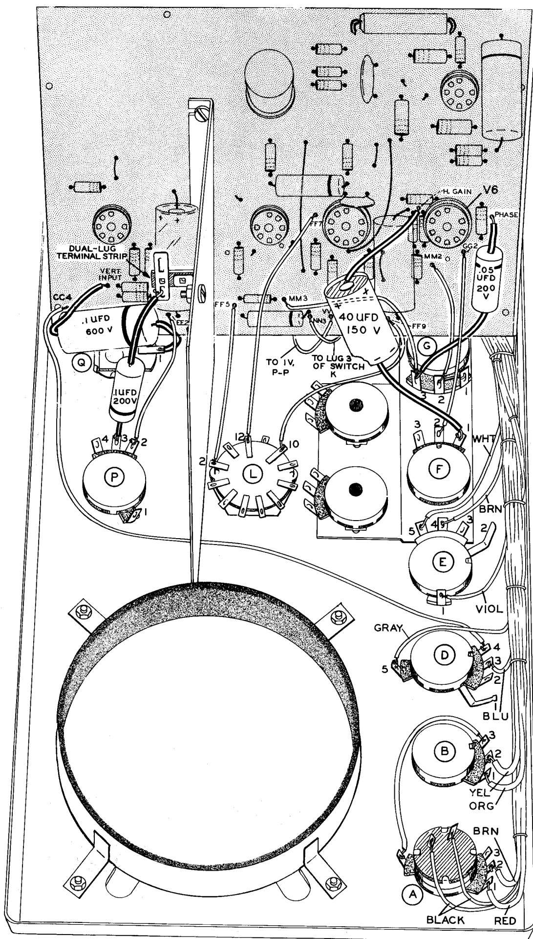
Pictorial 7
