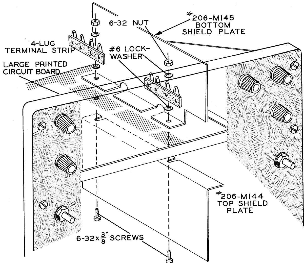
Detail 6A
