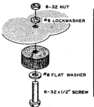
Detail 11A
