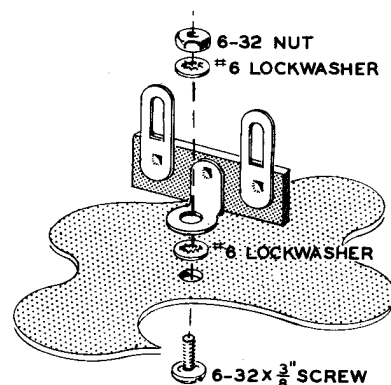
Detail 5B
