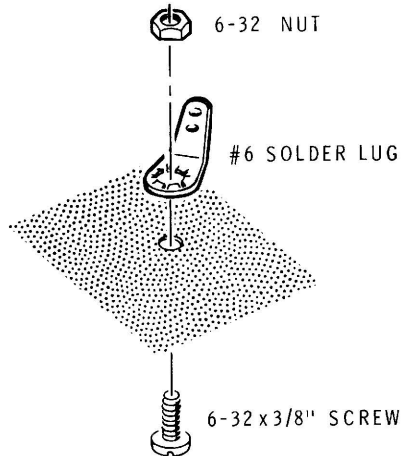
Detail 2-2F
