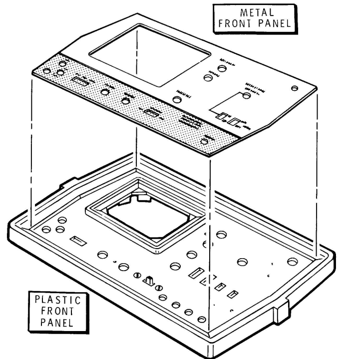
Detail 3-1B
