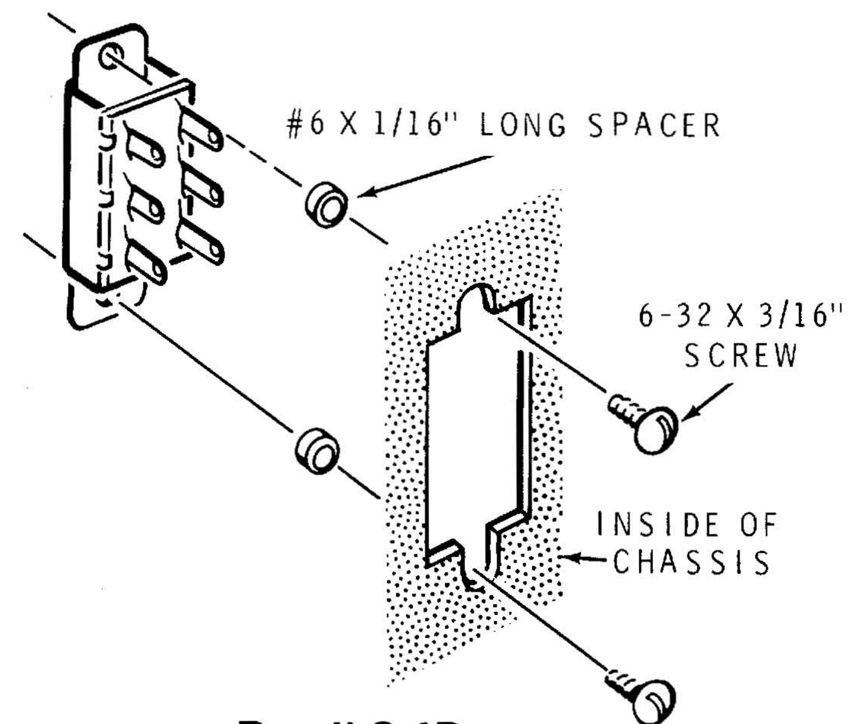
Detail 2-1B
