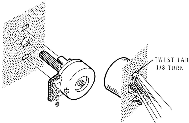
Detail 2-1D
