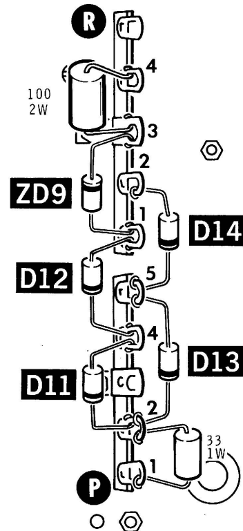
PICTORIAL 5-4
