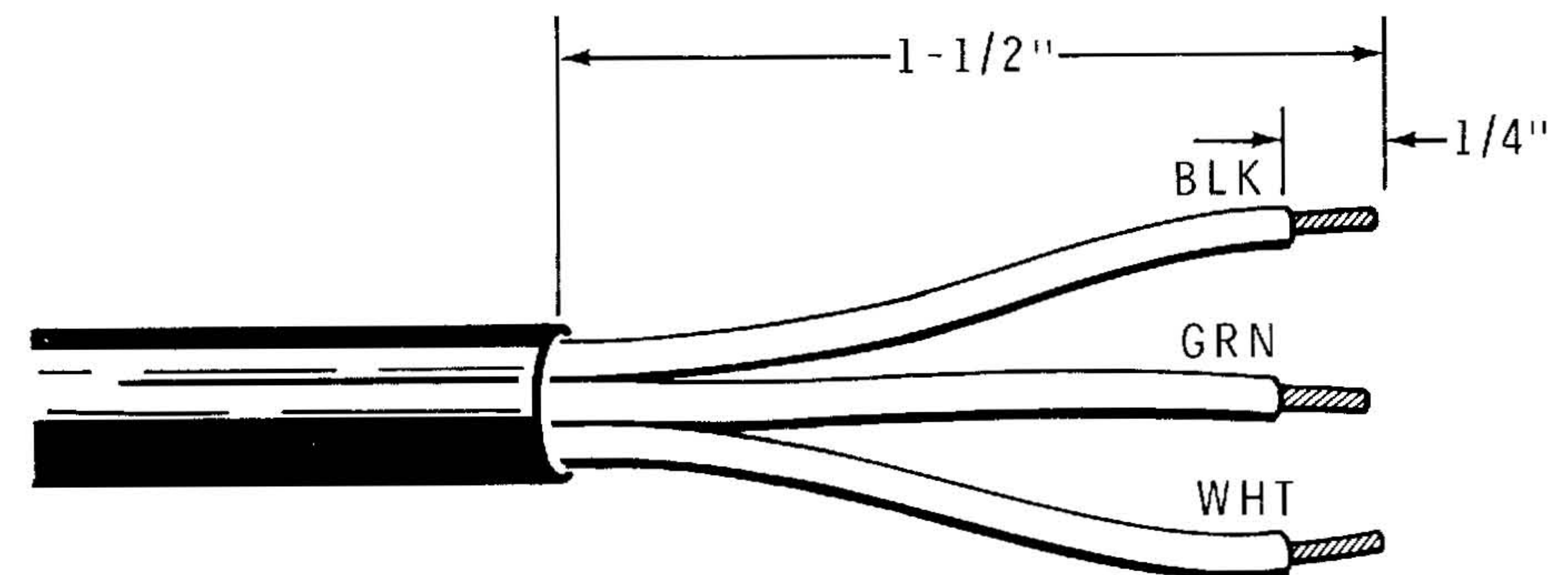
Detail 5-6A
