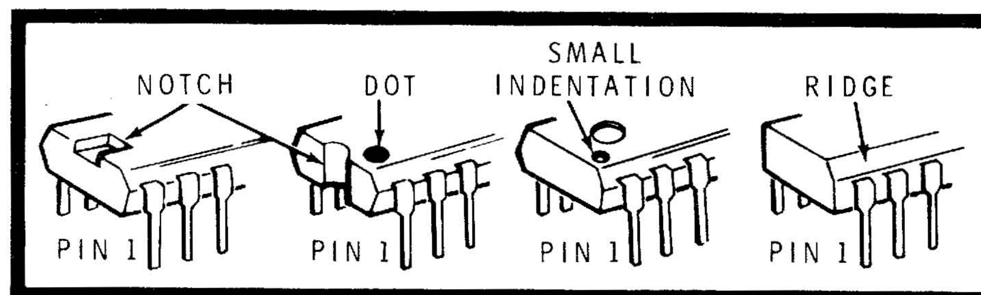
Detail 1-3A
