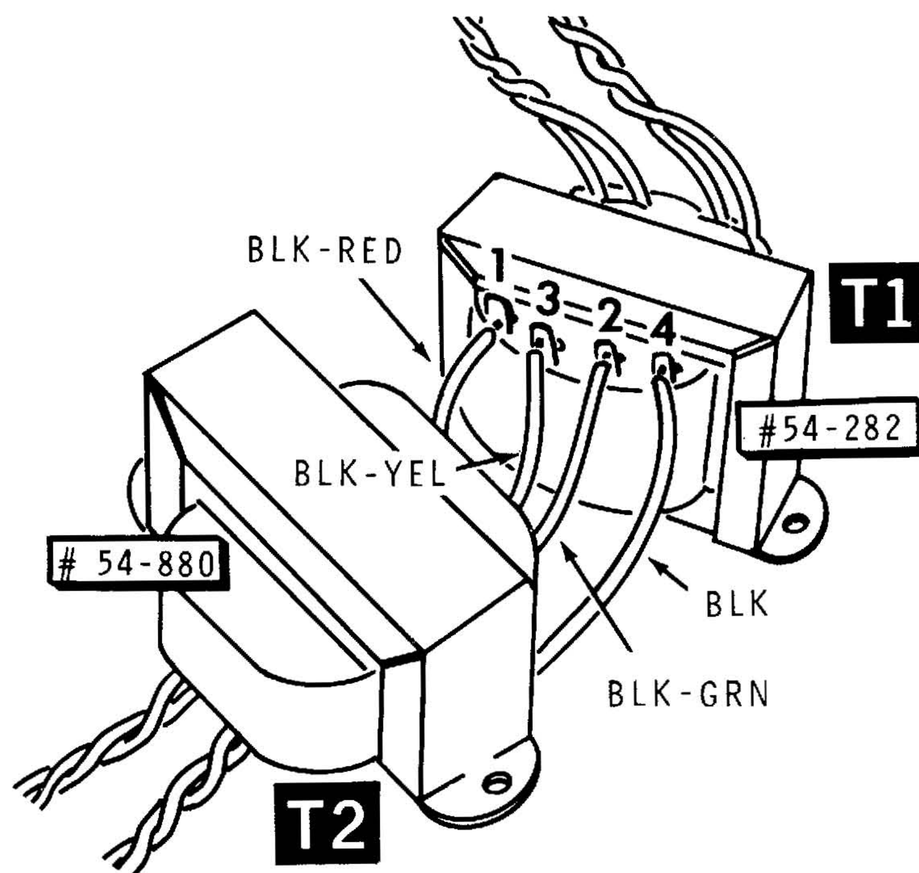
PICTORIAL 4-16
