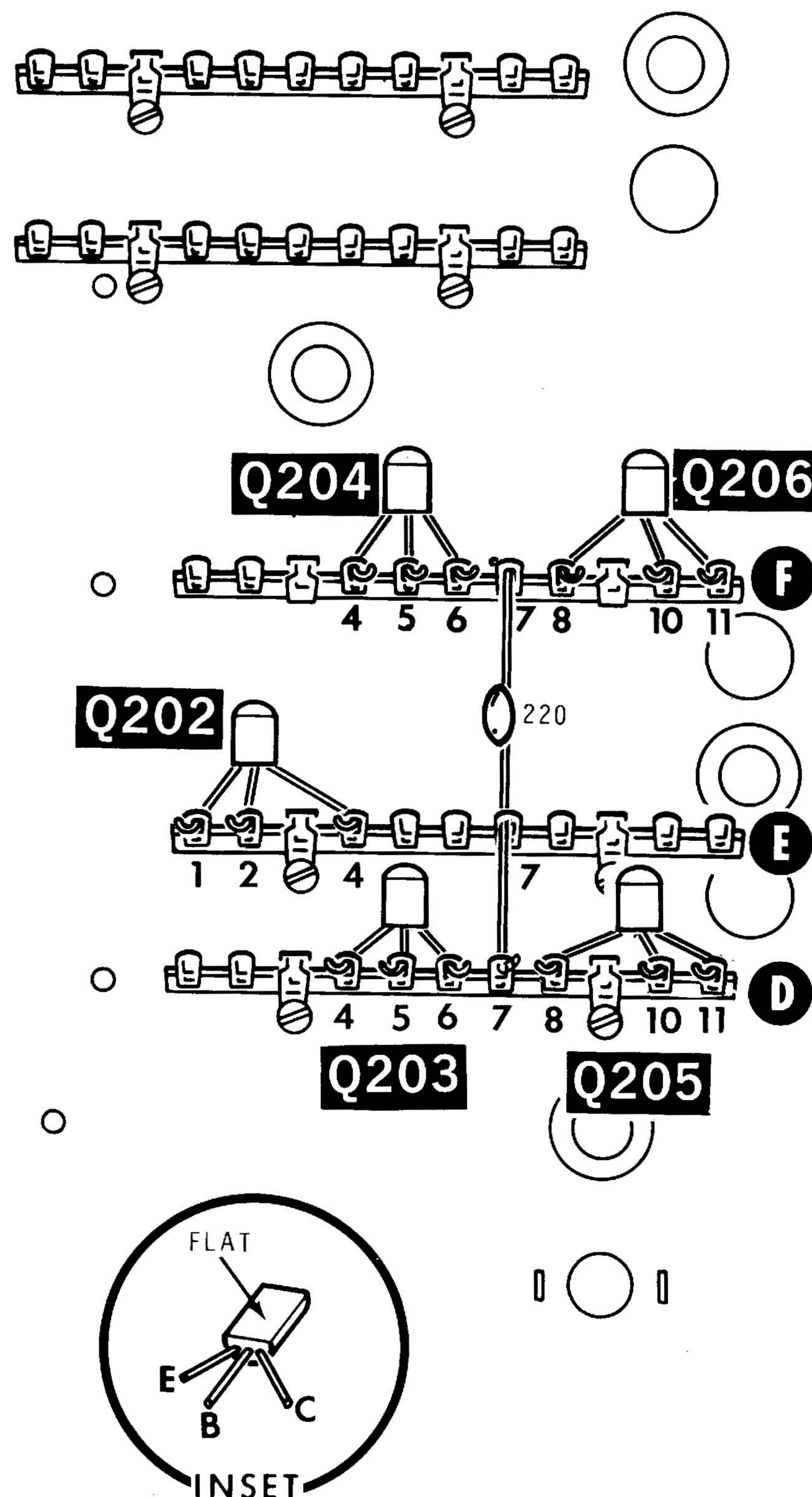
PICTORIAL 4-7
