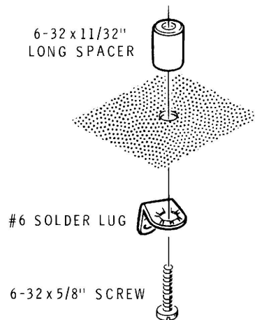
Detail 3-2C
