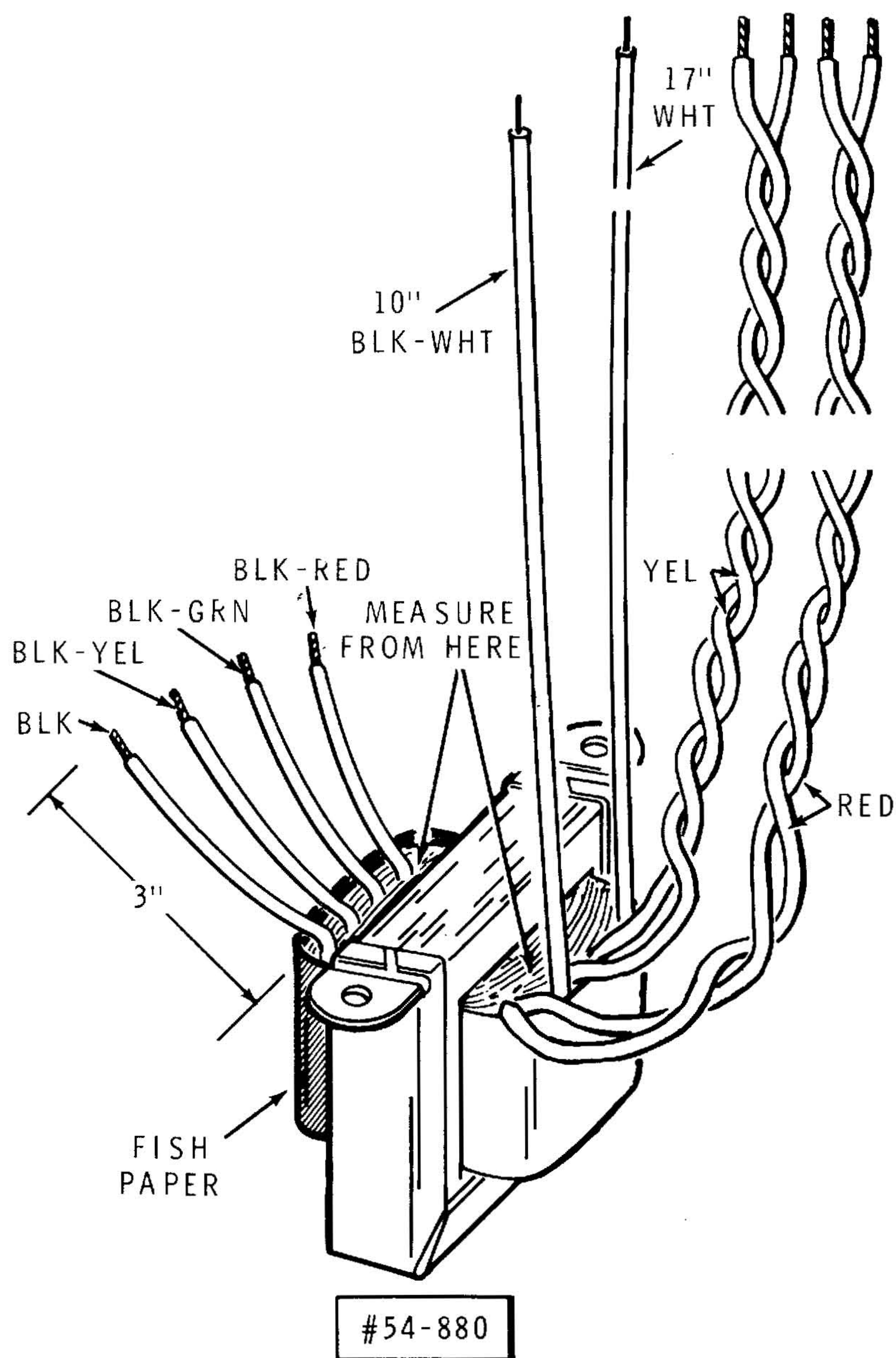
PICTORIAL 4-14
