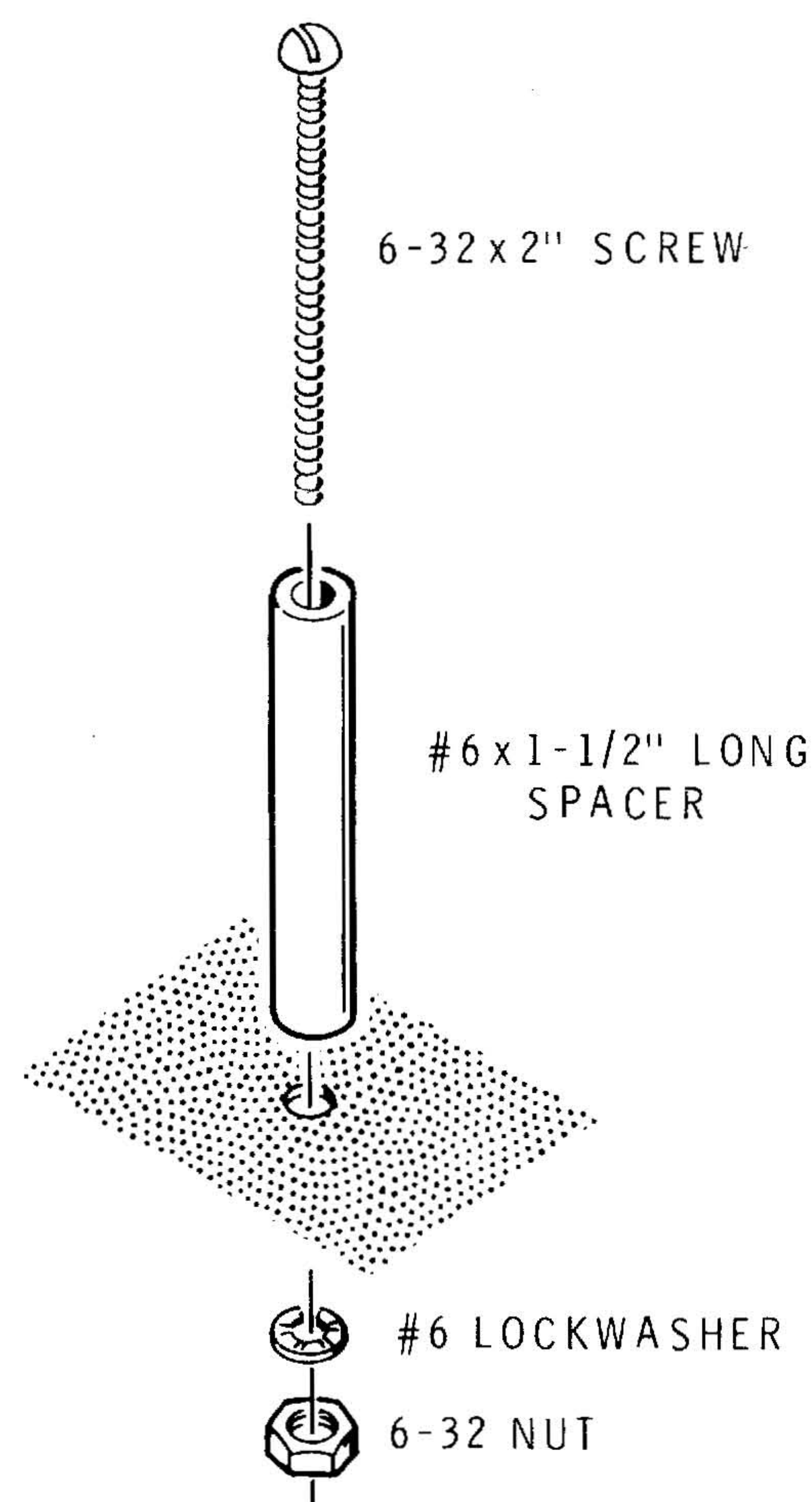
Detail 2-2D
