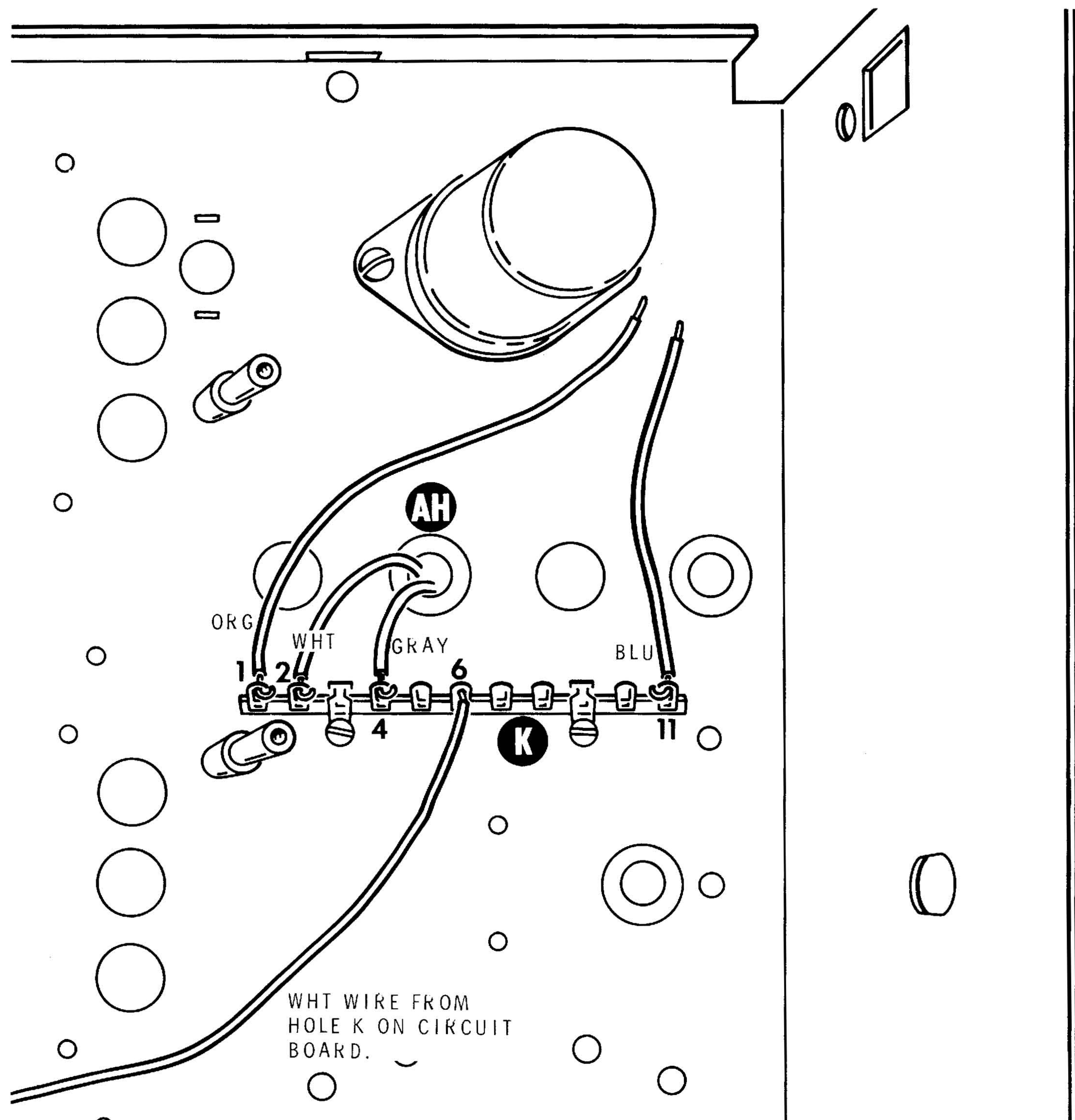
PICTORIAL 4-11
