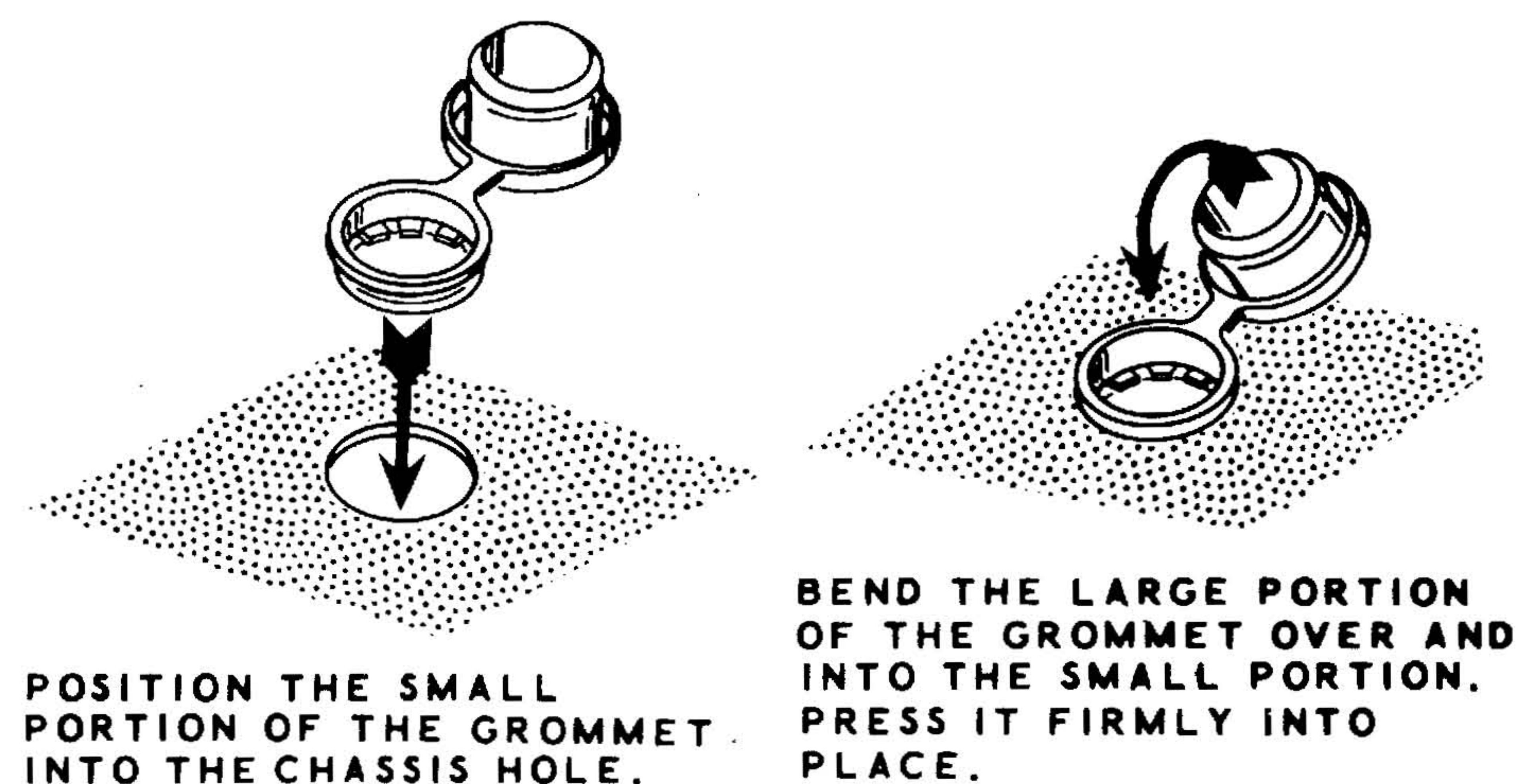
Detail 4-19A
