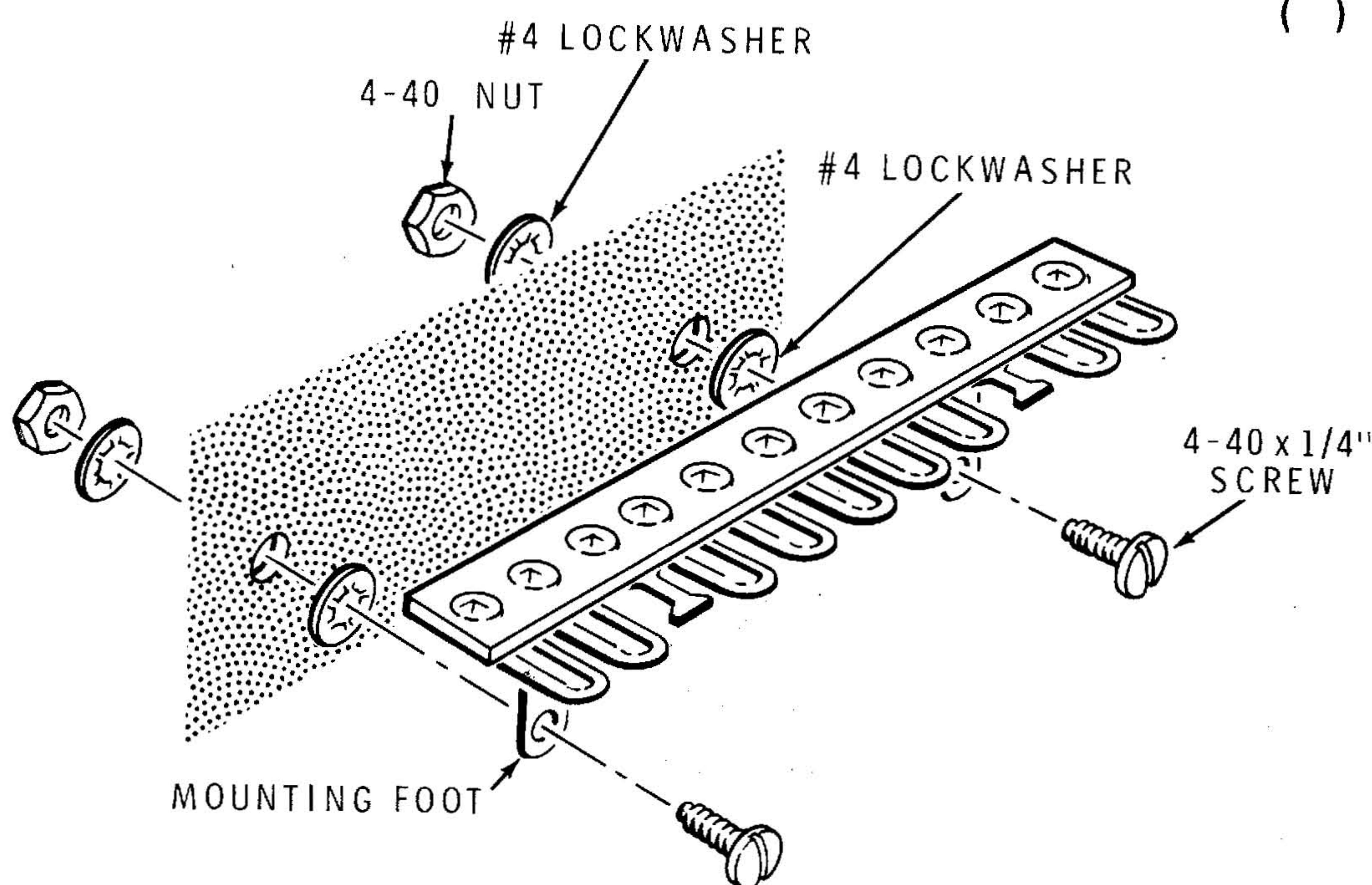
Detail 2-1A
