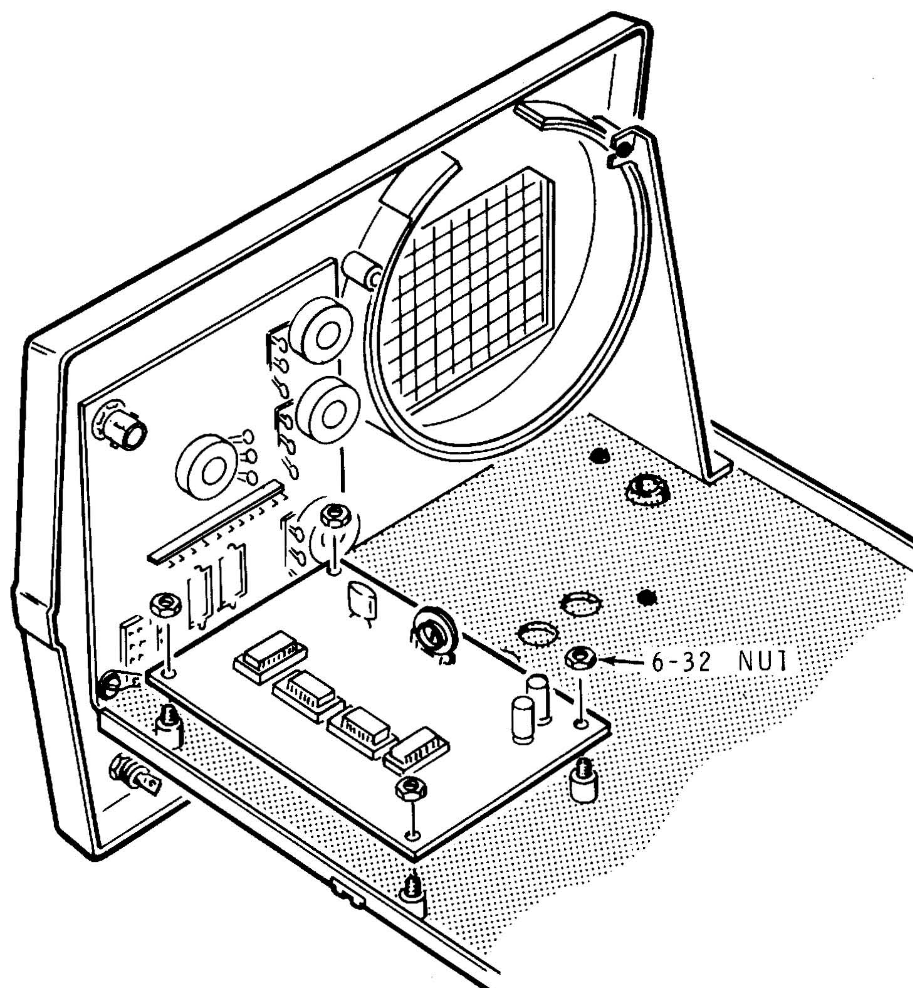
Detail 4-4A
