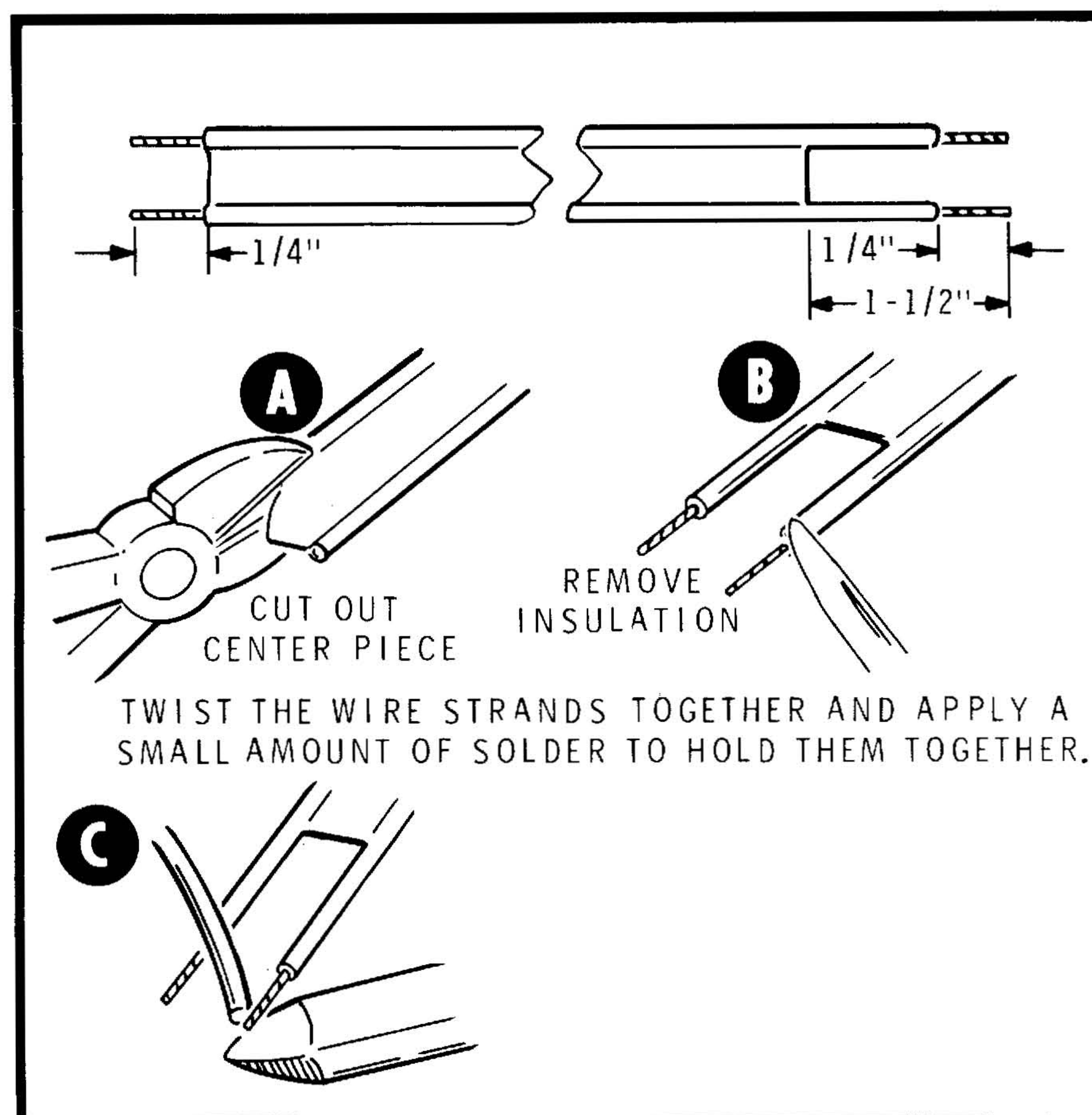
Detail 4-5A
