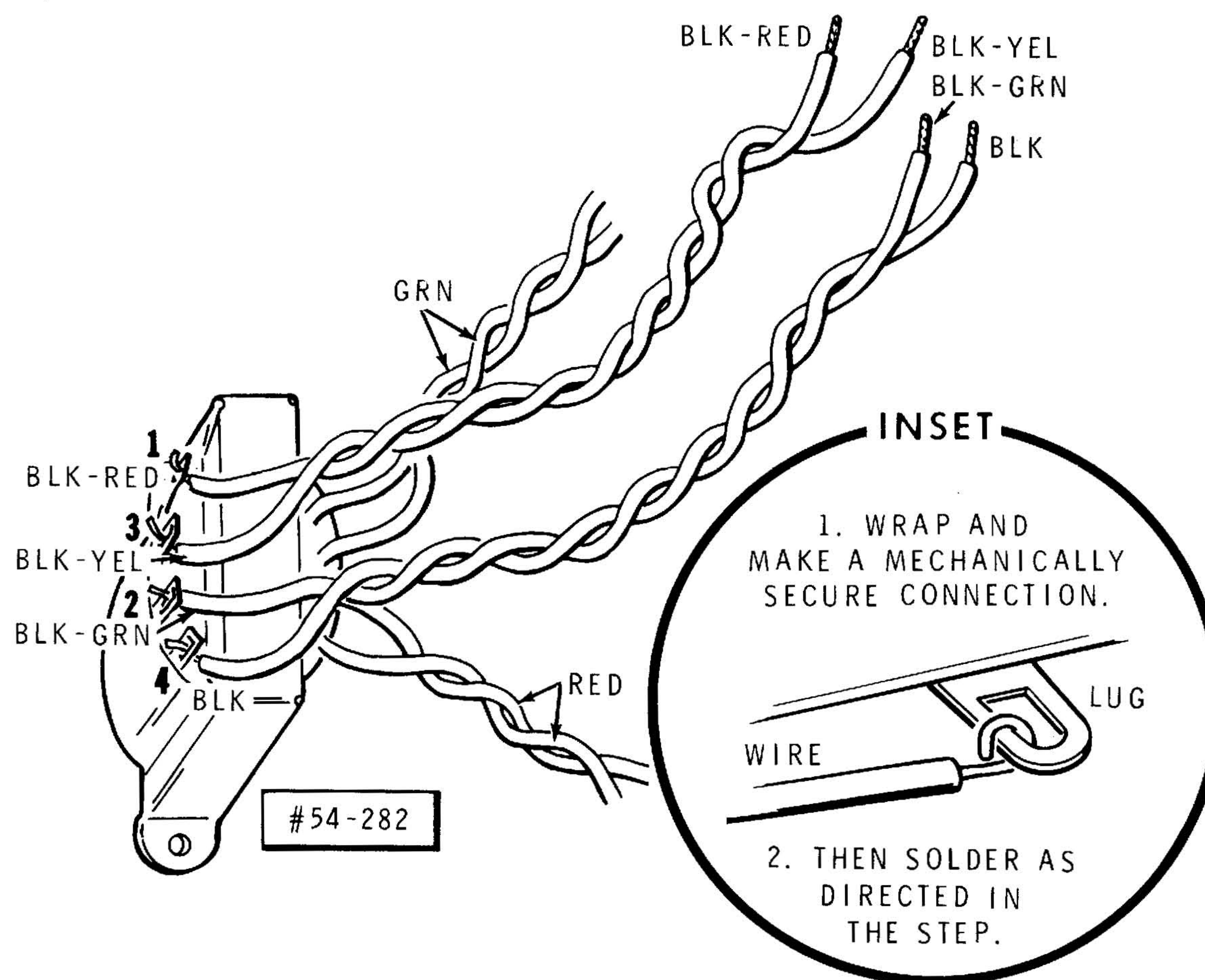
PICTORIAL 4-15
