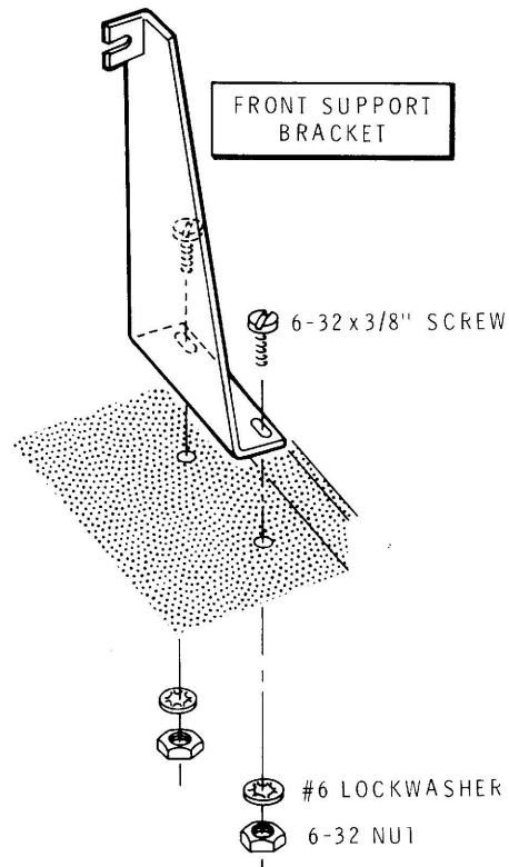
Detail 2-1F
