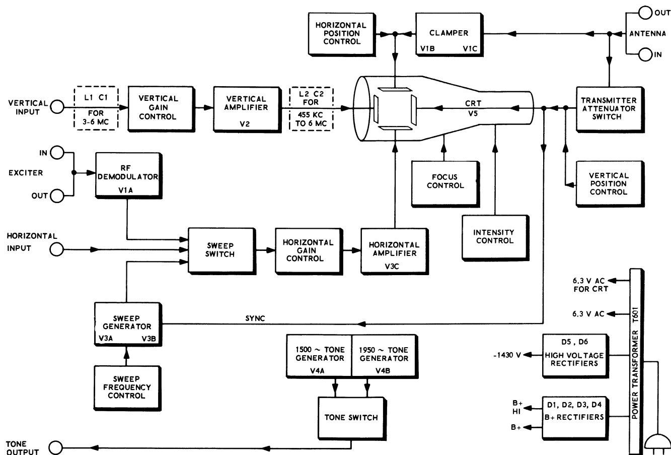
BLOCK DIAGRAM
