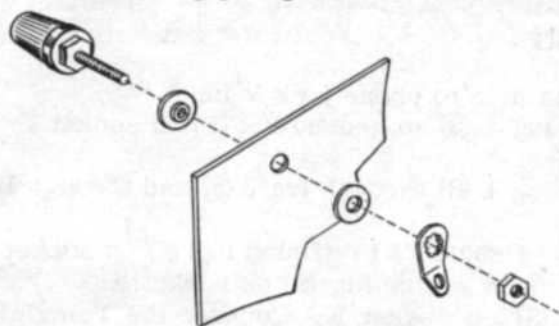
BINDING POST ASSEMBLY
