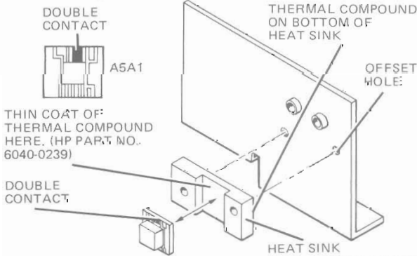
Figure 8-6. A5A1 Removal
