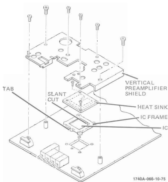
Figure 8-7. A3A1 Removal
