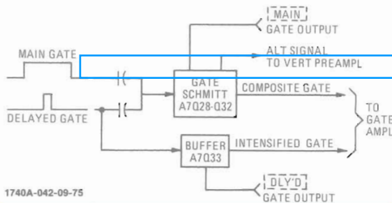
Figure 4-3. Gate Schmitt Simplified Block Diagram
