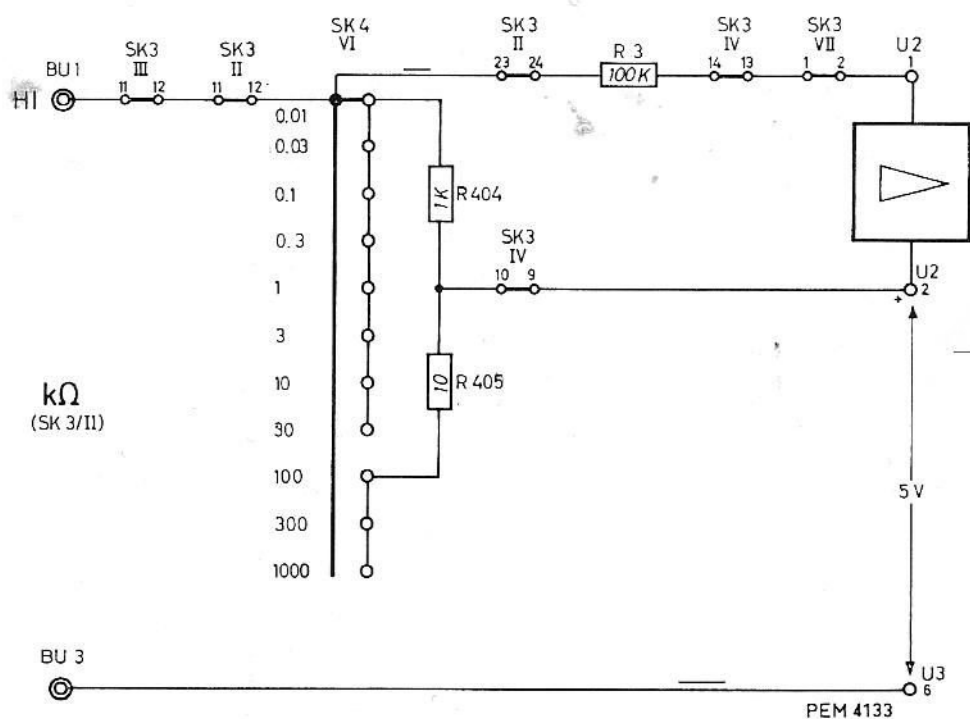
Fig. 12. Input circuit for k\Omega and M\Omega ranges
