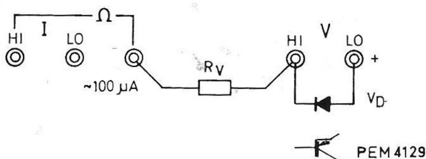
Fig. 9. Measuring the threshold voltage or breakdown voltage of semi-conductors
