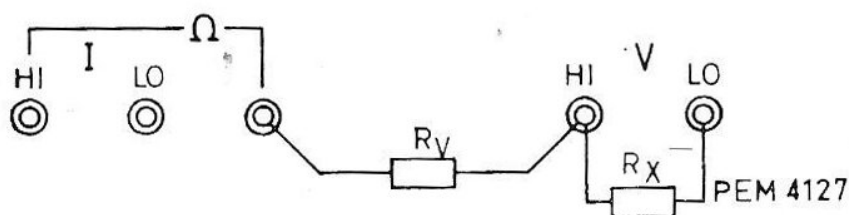
Fig. 7. Measuring resistance values lower than 5\text{ k}\Omega
