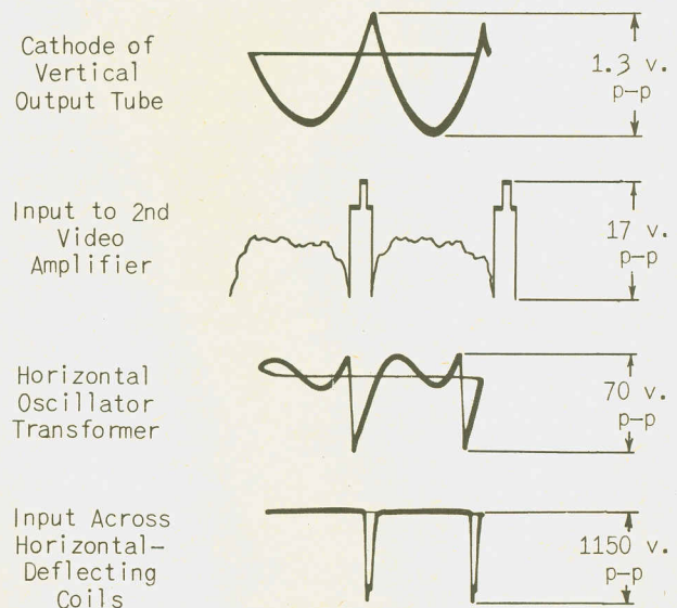
Figure 7. Typical television voltage waveforms
