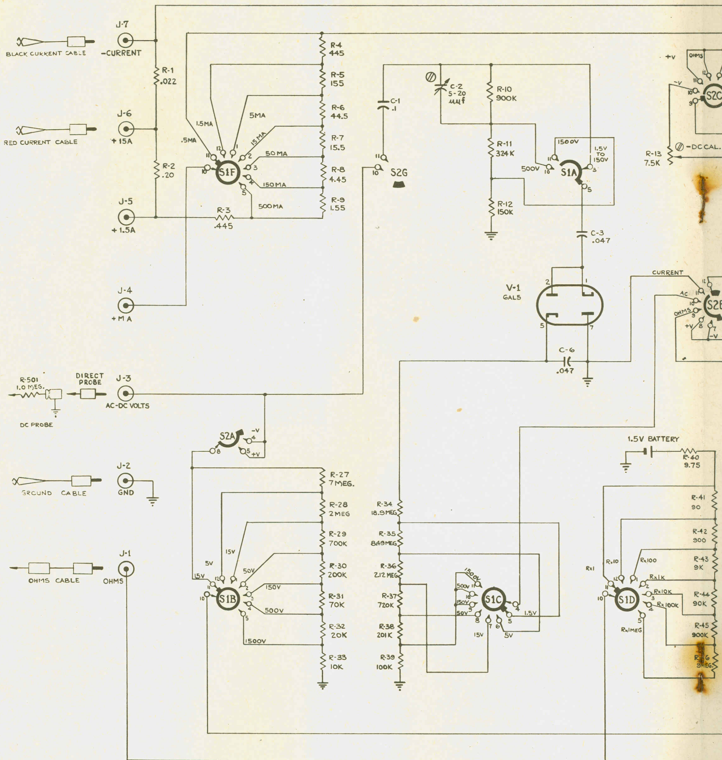
Figure 6. Schematic diag
