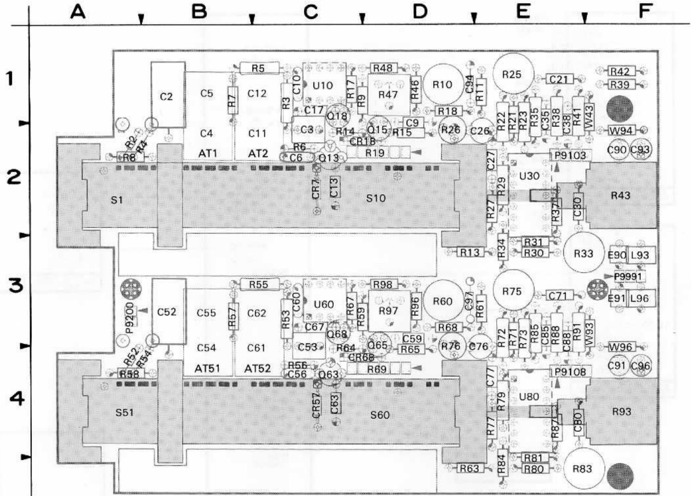
Figure 9-6. A2—Attenuator board.
