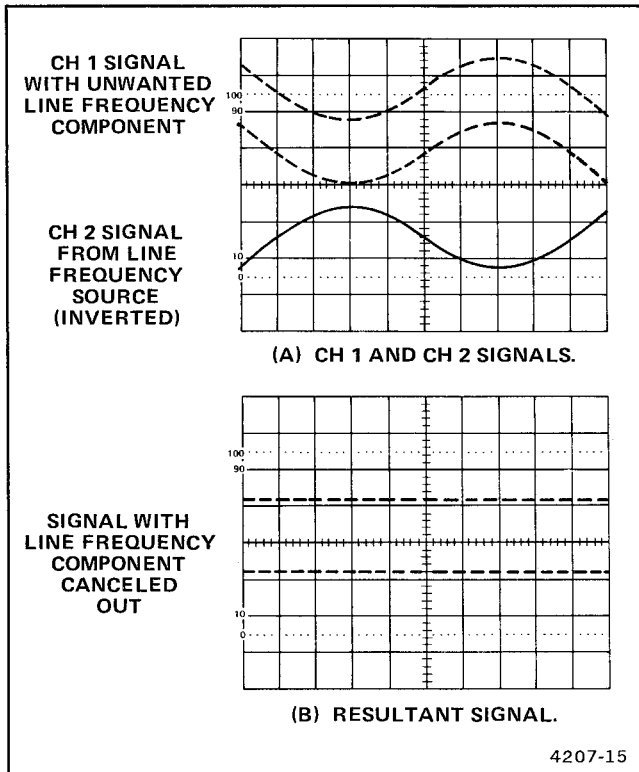
Figure 4-5. Common-mode rejection.
