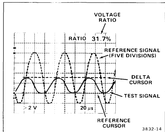
Figure 6-2. Voltage ratios.
