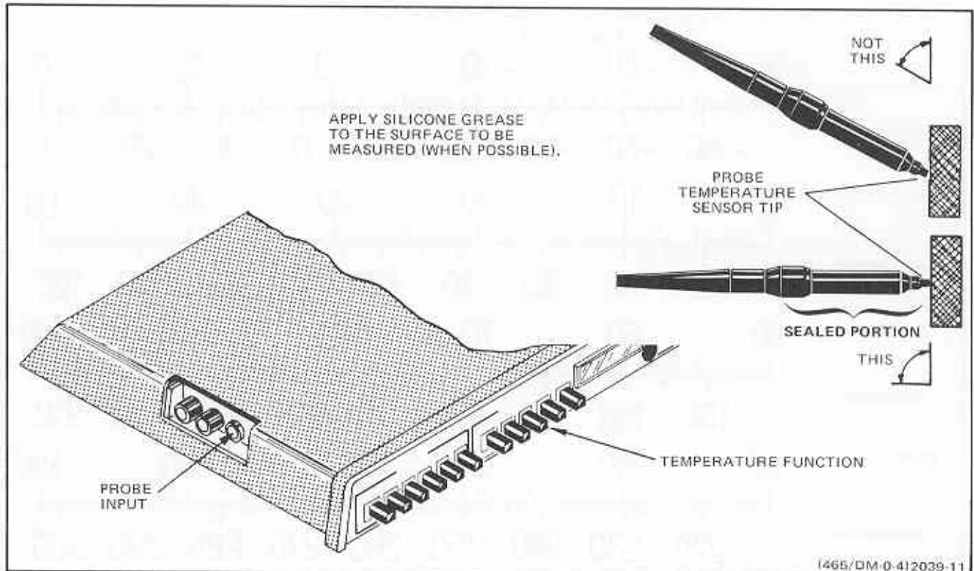
Fig. 10. Temperature.
