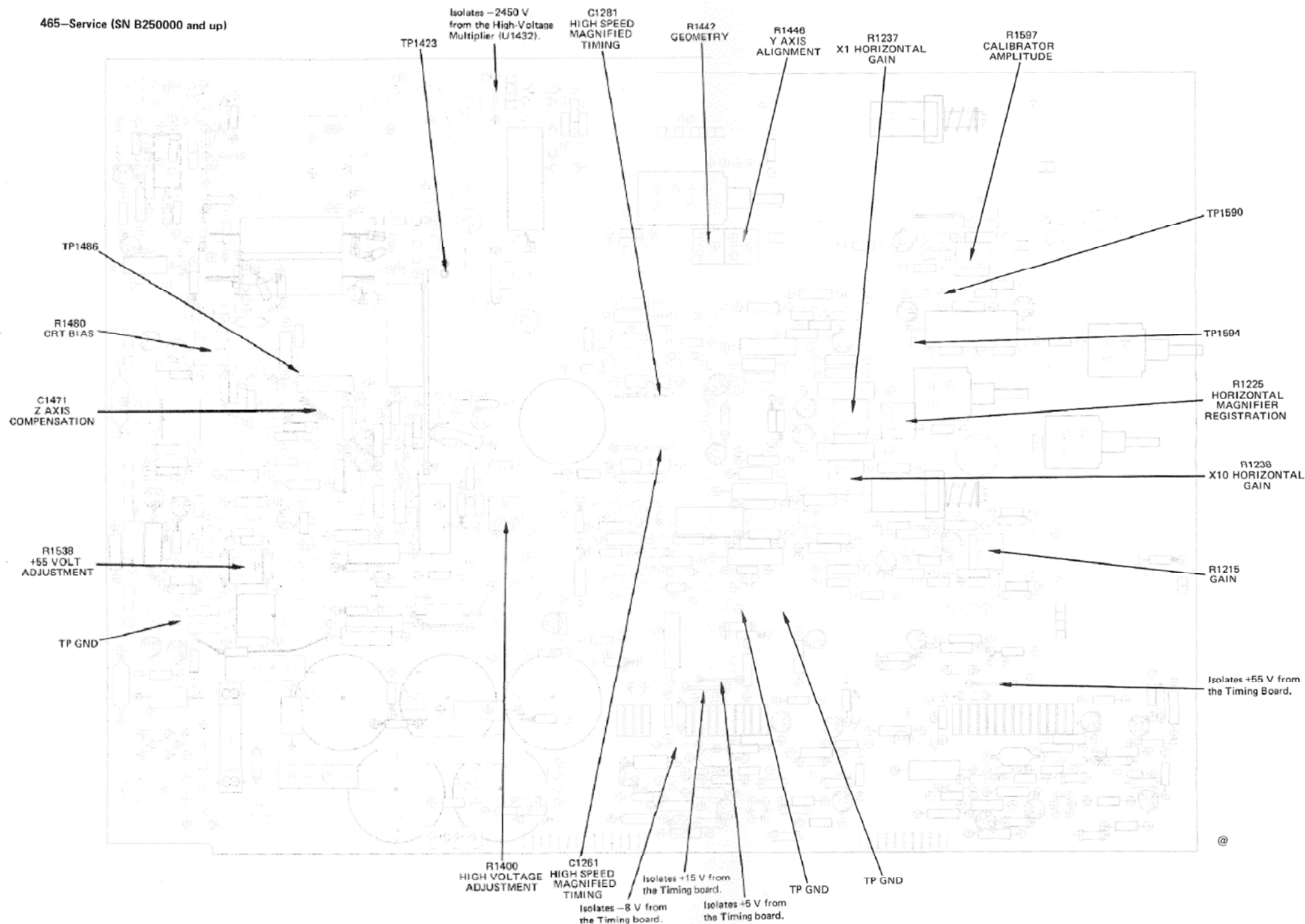
Fig. 8-19. Interface circuit board adjustment locations.
