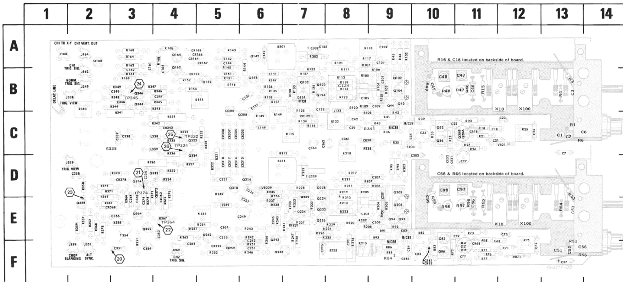
Fig. 8-6. A1 &amp; A2—Attenuators and A3—Vertical Preamp circuit boards.
