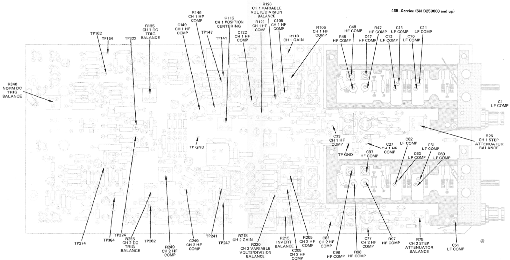
Fig. 8-20. Vertical Preamplifier and Attenuator circuit board adjustment locations.
