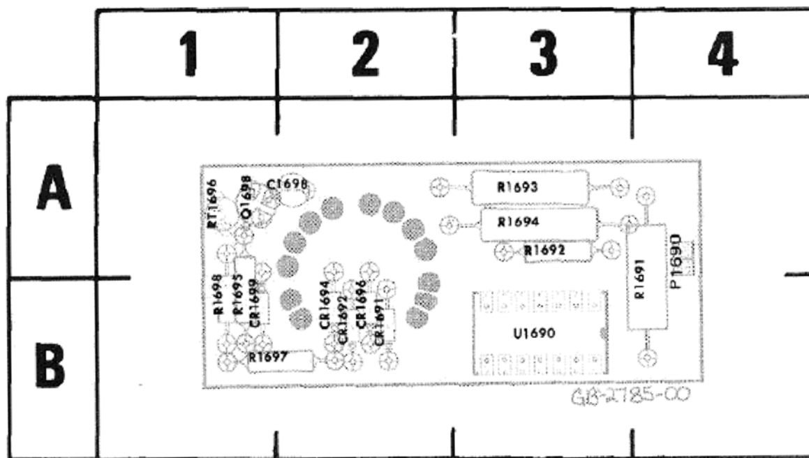
Fig. 8-15. A6-Fan circuit board.
