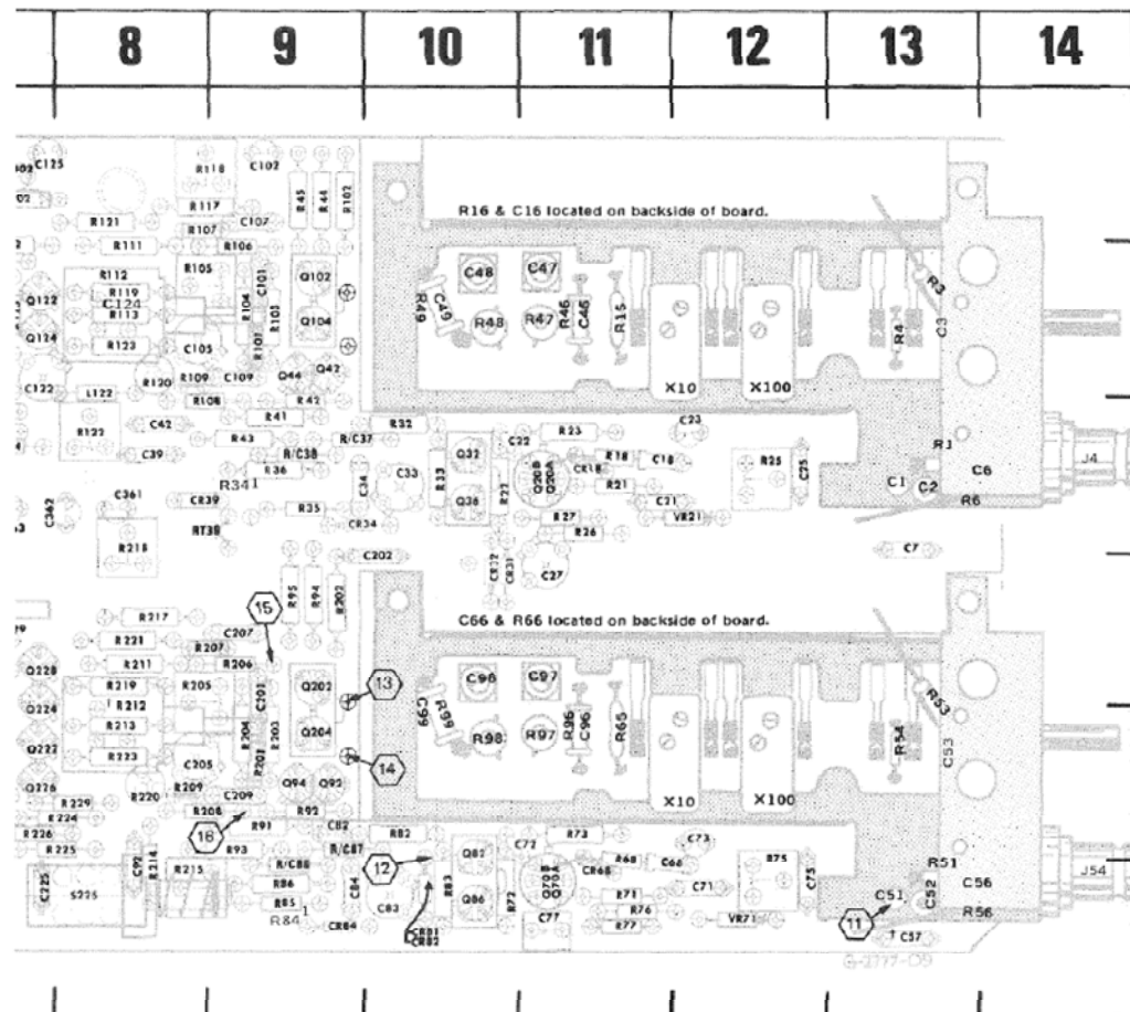
8rs and A3—Vertical Preamp circuit boards.
