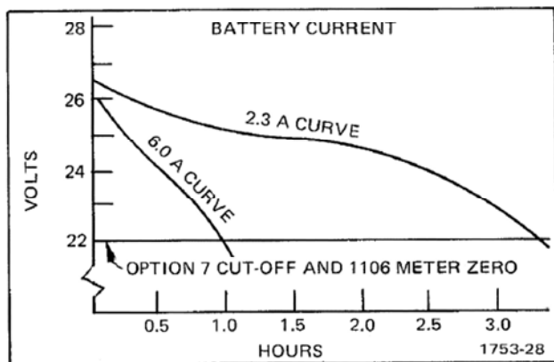
Fig. Option 7-4. Typical battery pack discharge curves.
