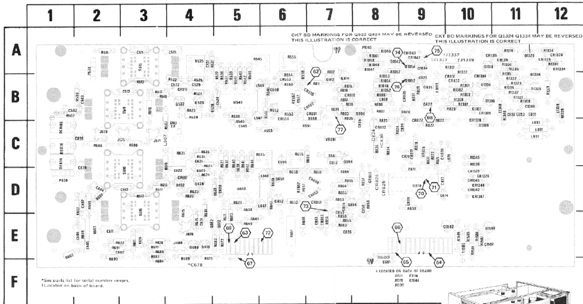
Fig. 8-12. A8—Trigger Generator and Sweep Logic circuit board.
