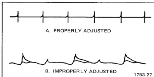
Fig. Option 7-5. Inverter Balance.
