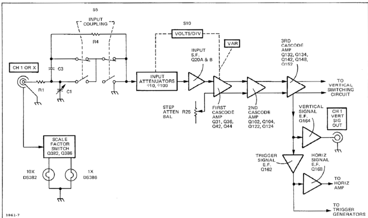
Fig. 3-2. Detailed block diagram of the Channel 1 Preampifier.
