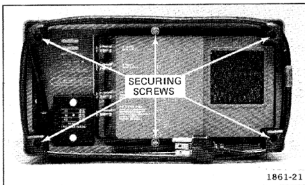
Fig. 4-1. Removing the wrap around cabinet.
