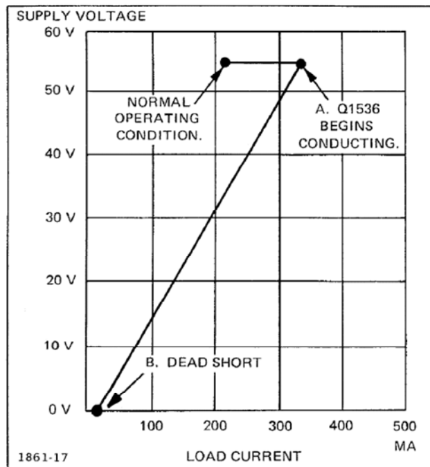
Fig. 3-12. Foldover circuit action.
