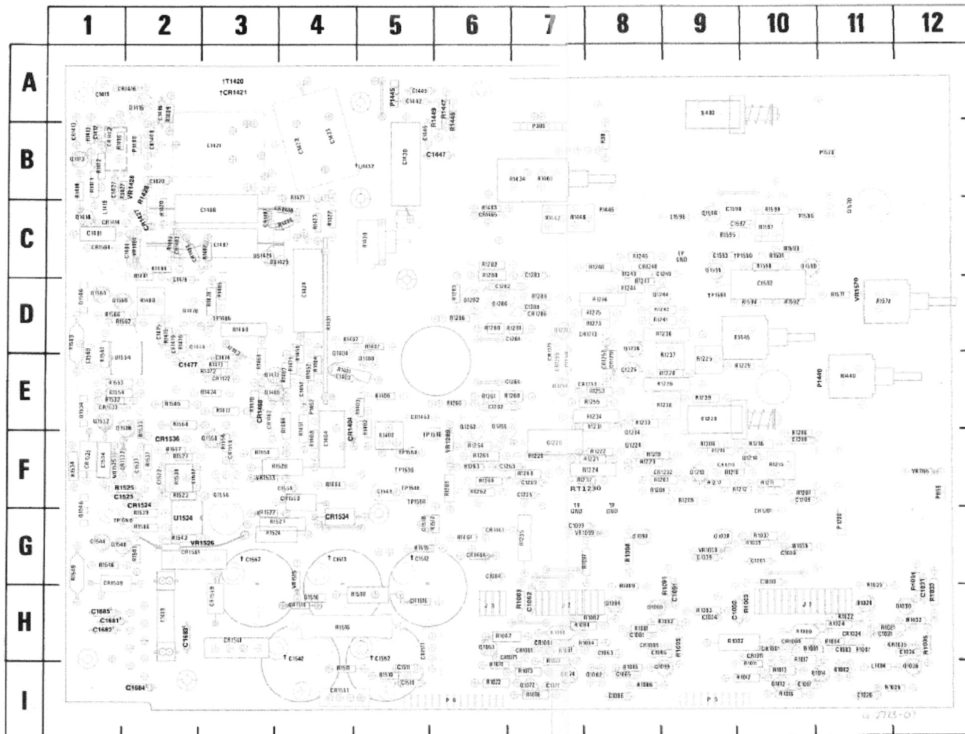
Fig. 8-18. A9—Interface circuit board.
