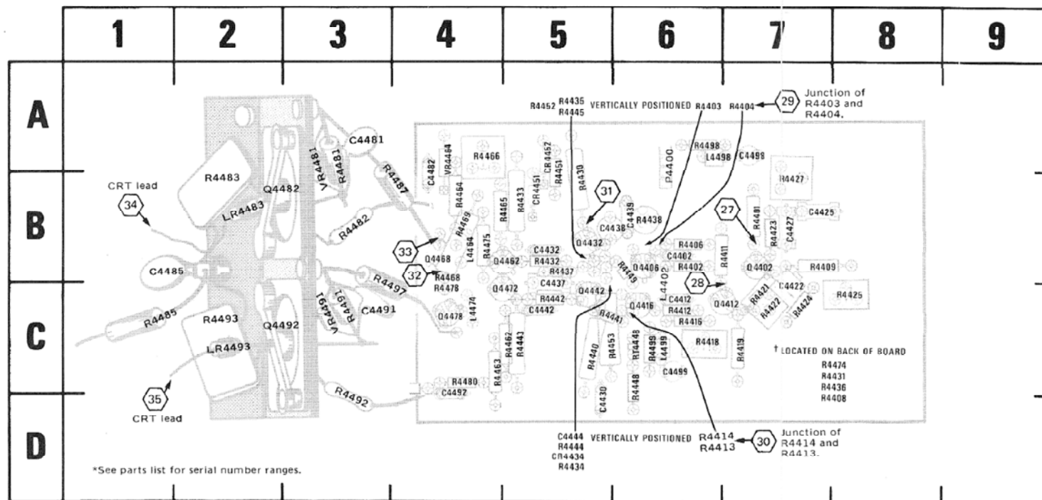
Fig. 8-7. A5a—Vertical Output Amplifier circuit board (discrete version).
