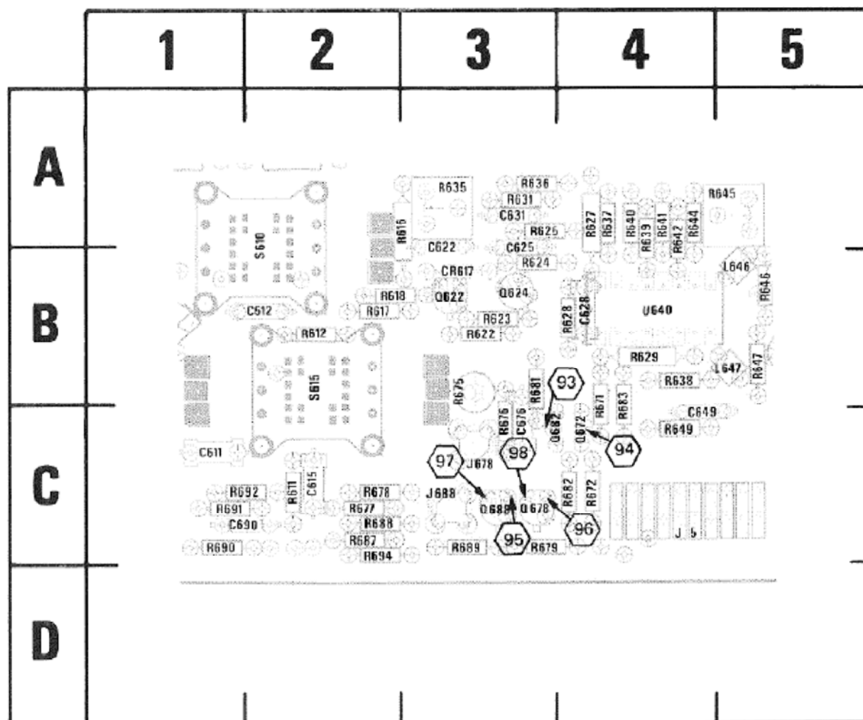
Fig. B-16. Partial A8-Trigger Generator and Sweep Logic circuit boards.
