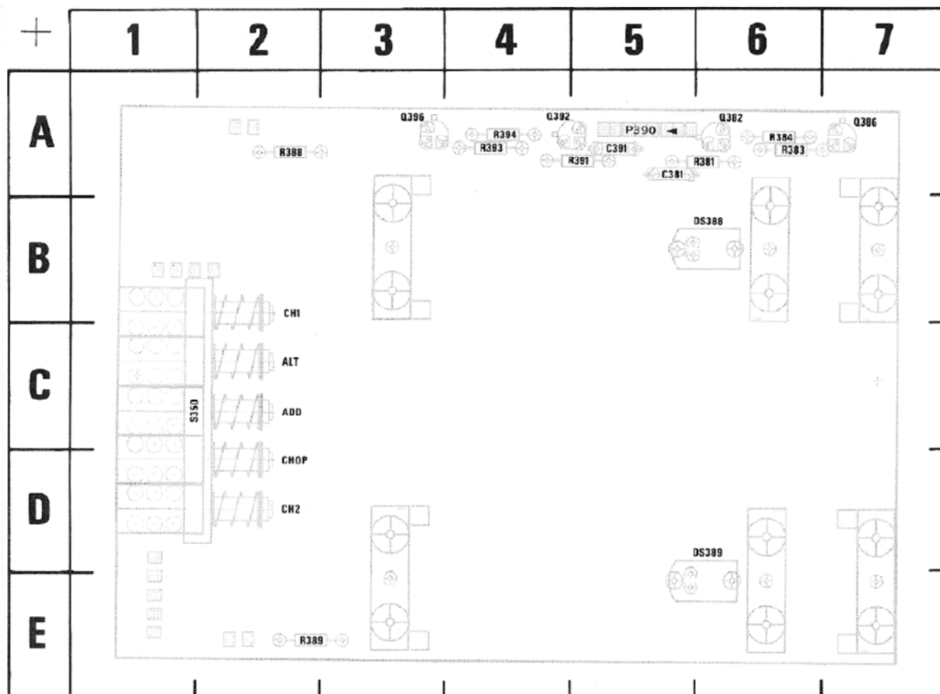
Fig. 8-3. A4-Vertical Mode Switch circuit board.
