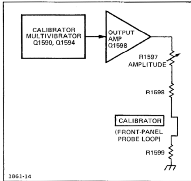
Fig. 3-9. Detailed block diagram of the Calibrator circuit.
