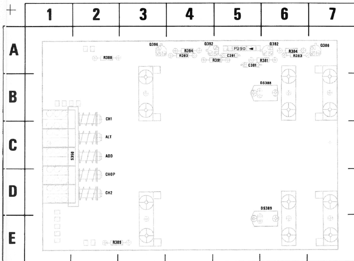
Fig. 8-5. A4—Vertical Mode Switch circuit board.
