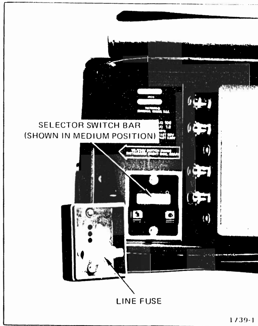
Fig. 1. Regulating range selector and line fuse.
