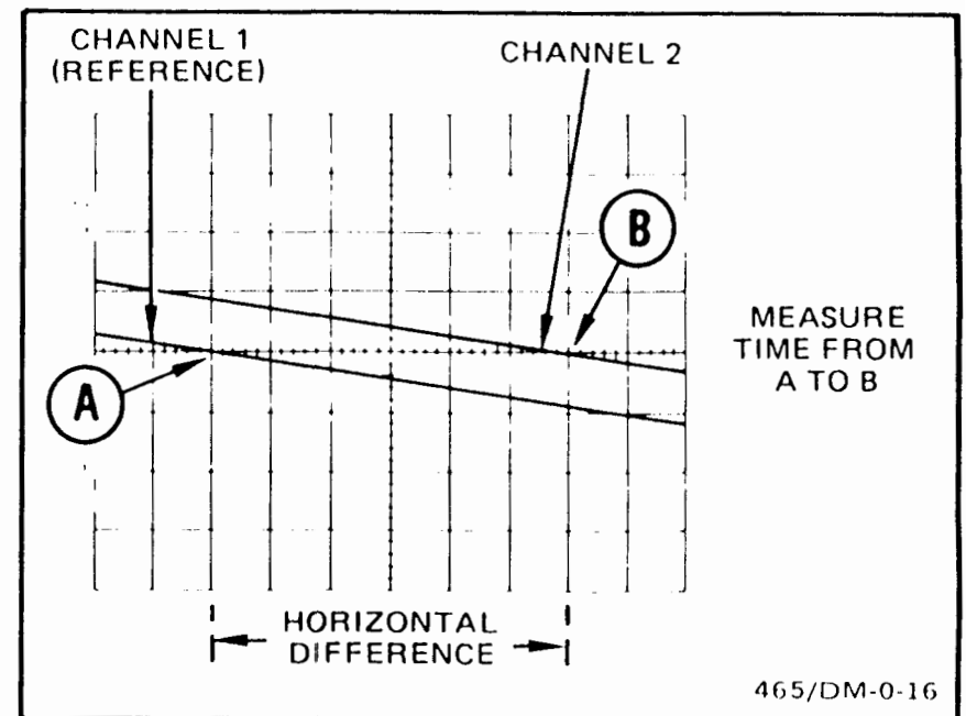
Fig. 22. High-resolution phase difference.
