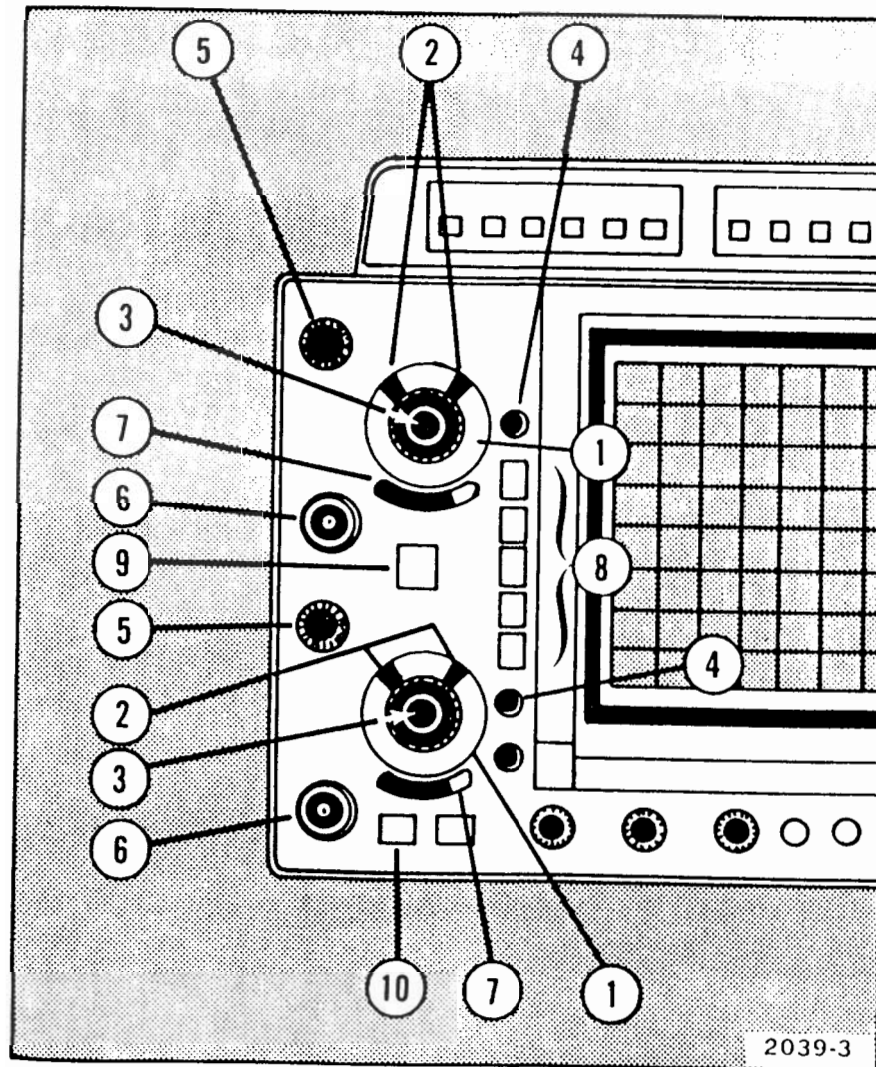
Fig. 2. Vertical controls, connectors, and indicators.
