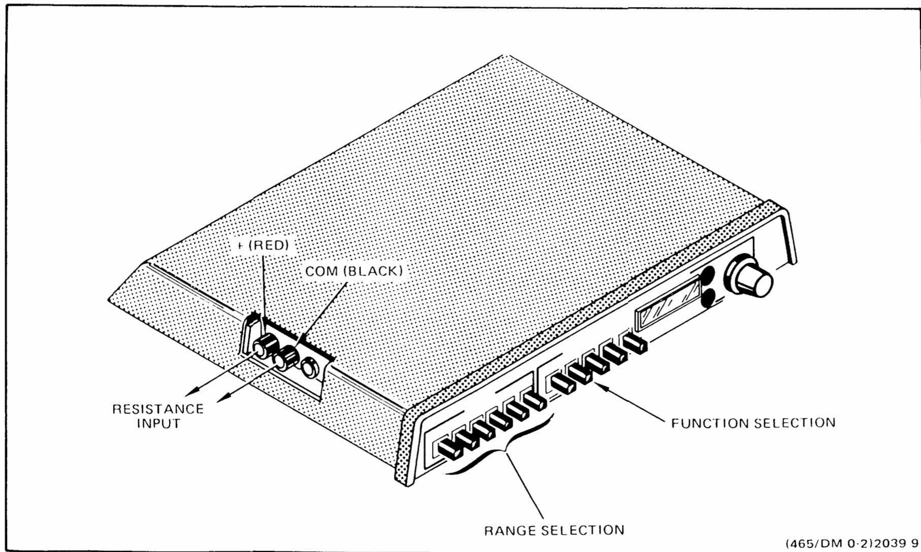
Fig. 8. Resistance.
