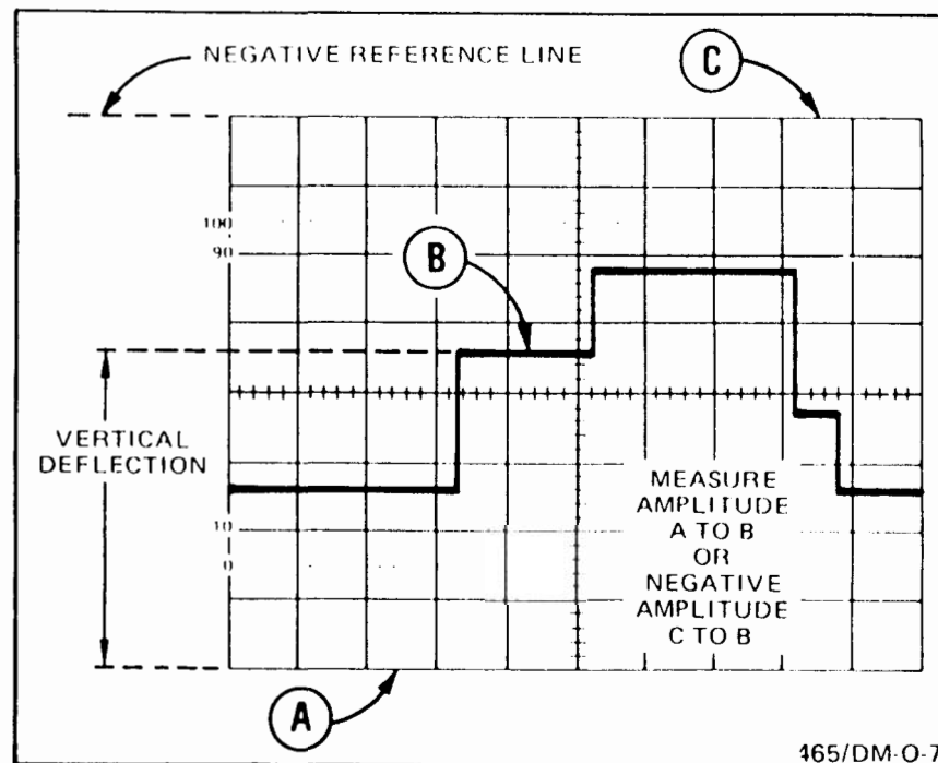
Fig. 15. Instantaneous voltage measurement.
