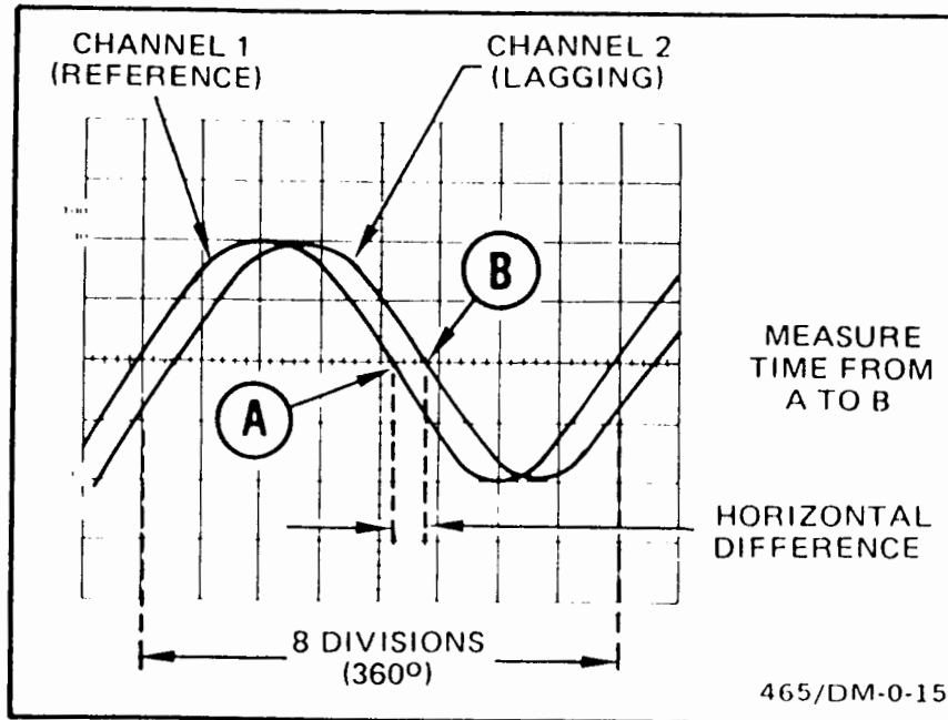
Fig. 21. Phase difference.
