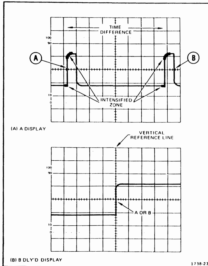
Fig. 25. Time difference between repetitive pulses.
