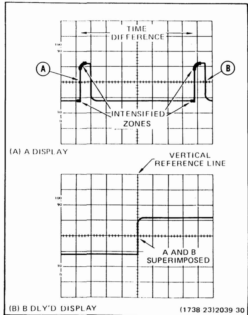
Fig. 29. Time difference between repetitive pulses.
