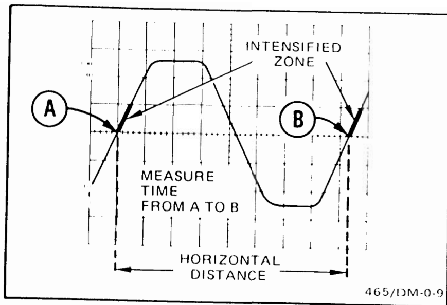
Fig. 26. Time duration.
