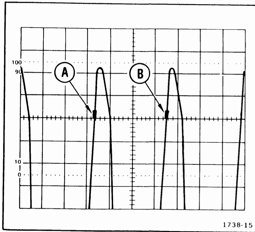
Fig. 13. DM44 timing check.
