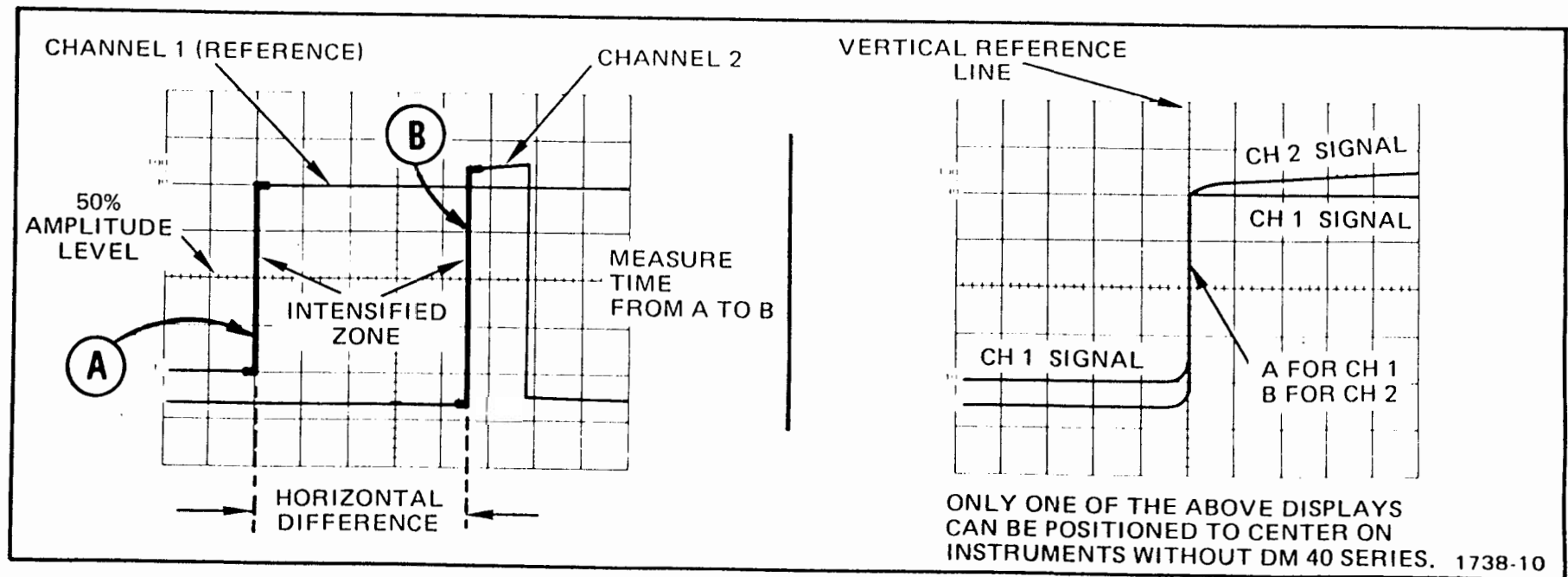
Fig. 27. Time difference between two pulses from different sources.
