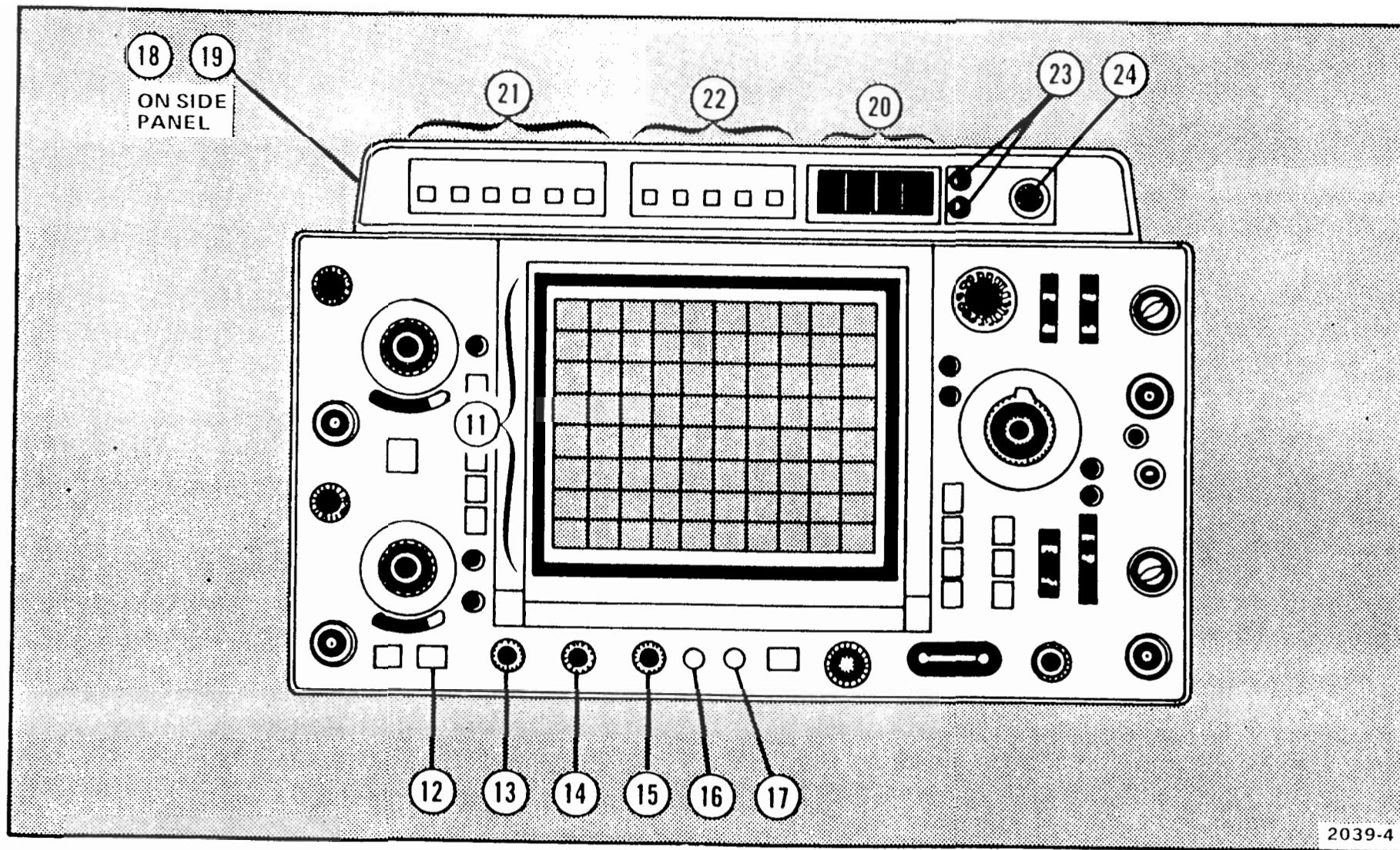
Fig. 3. Display and DM44 controls, connectors, and indicators.
