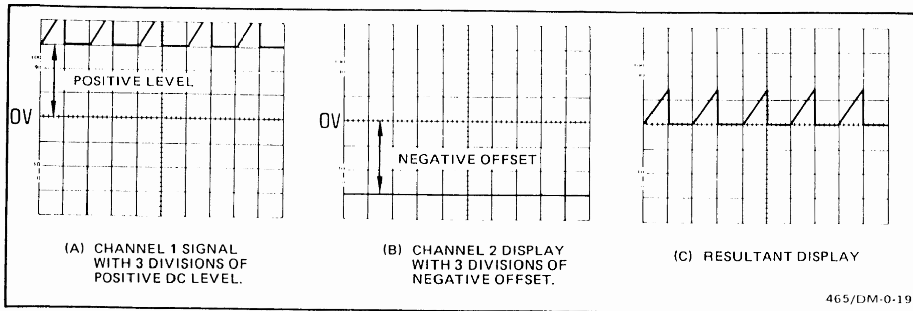
Fig. 16. Algebraic addition.
