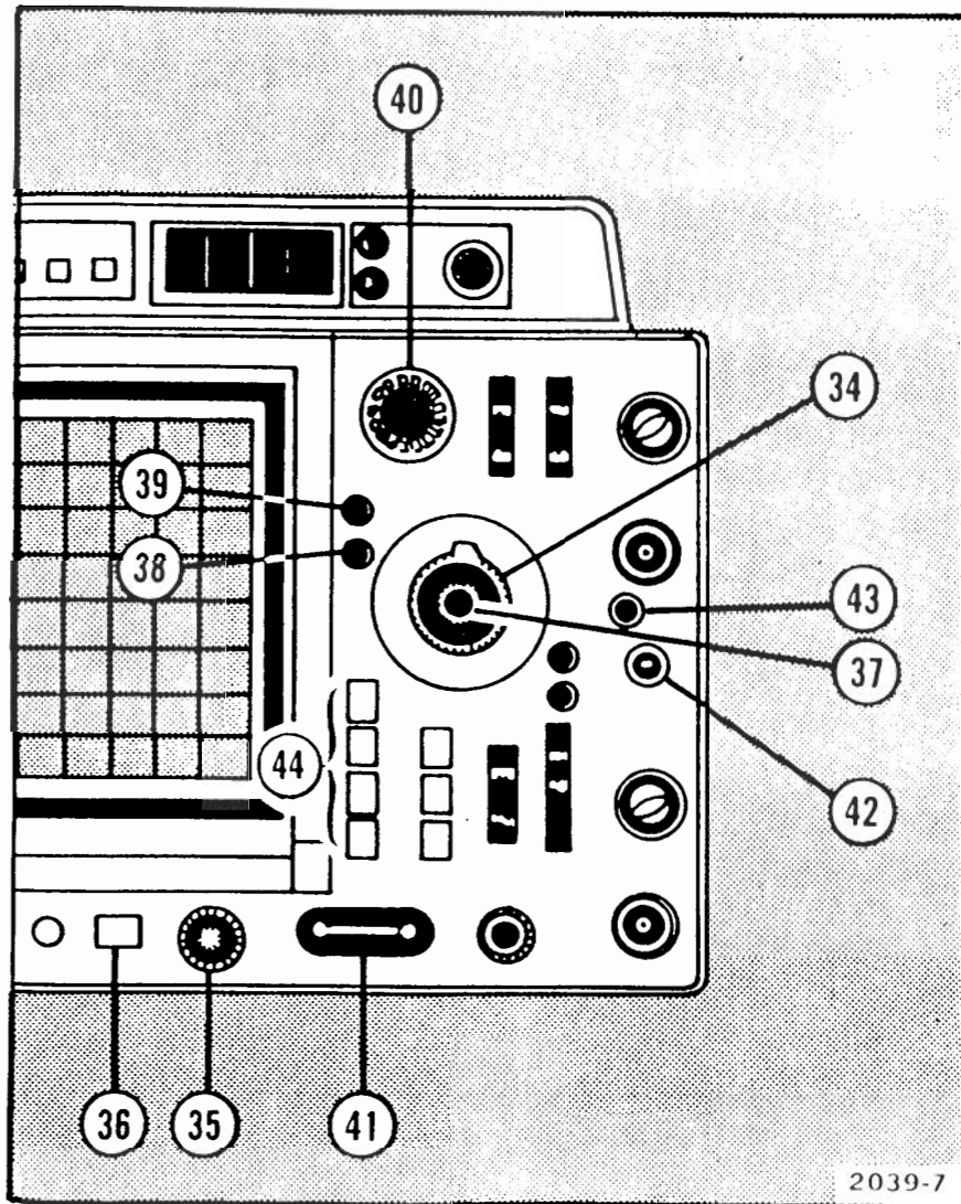
Fig. 6. Horizontal, calibrator, and power controls, connectors, and indicators.
