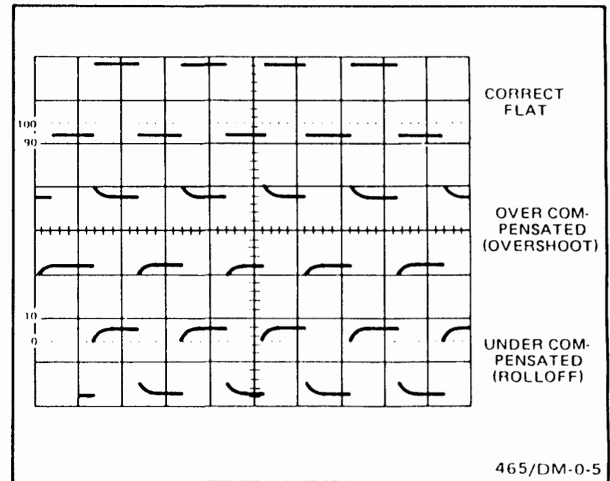
Fig. 11. Probe compensation.
