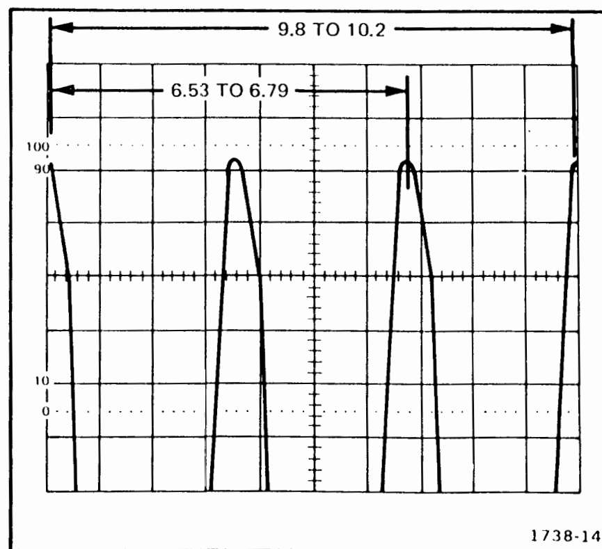
Fig. 12. Basic 475A timing check.
