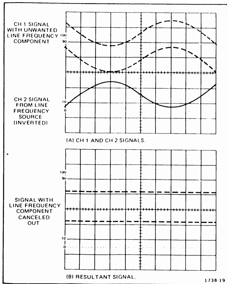
Fig. 17. Common-mode rejection.
