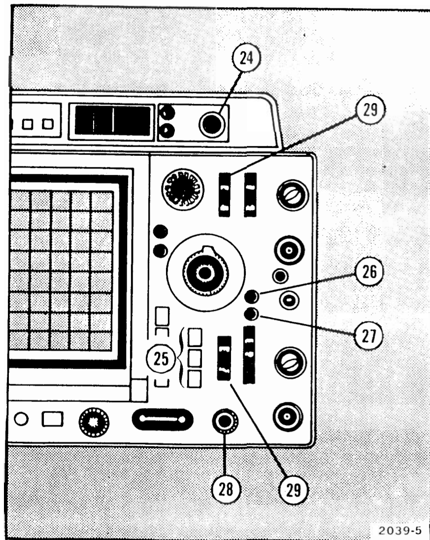
Fig. 4. Trigger controls, connectors, and indicators.
