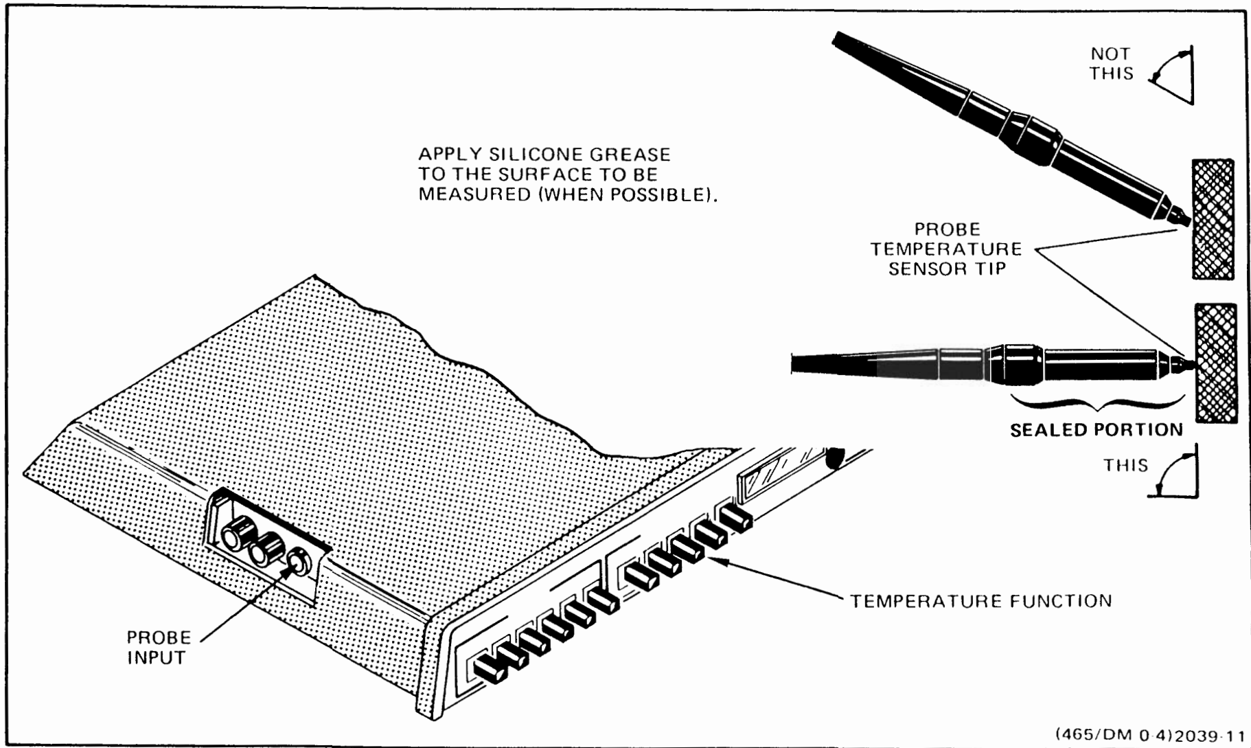
Fig. 10. Temperature.
