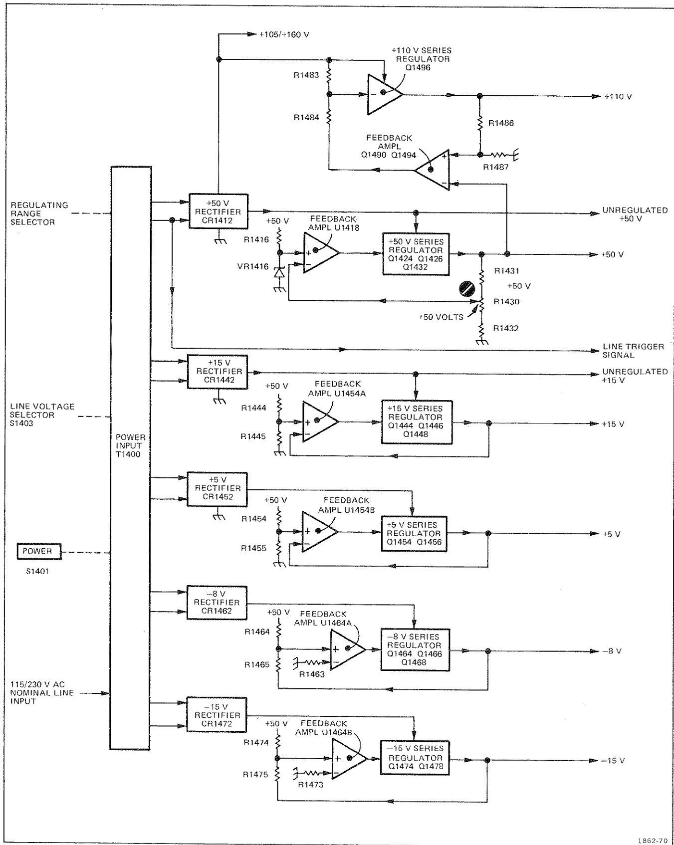
Fig. 3-9. Detailed block diagram of the Power Supply circuit.
