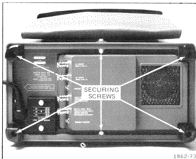
Fig. 4-1. Removing the standard cabinet.
