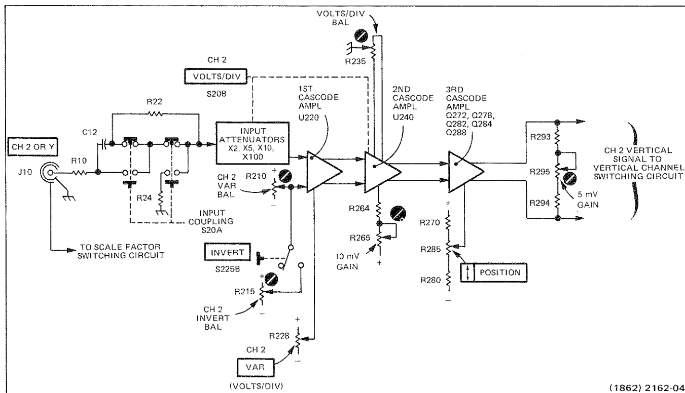
Fig. 3-3. Detailed block diagram of the Channel 2 Vertical Preamplifier circuit.
