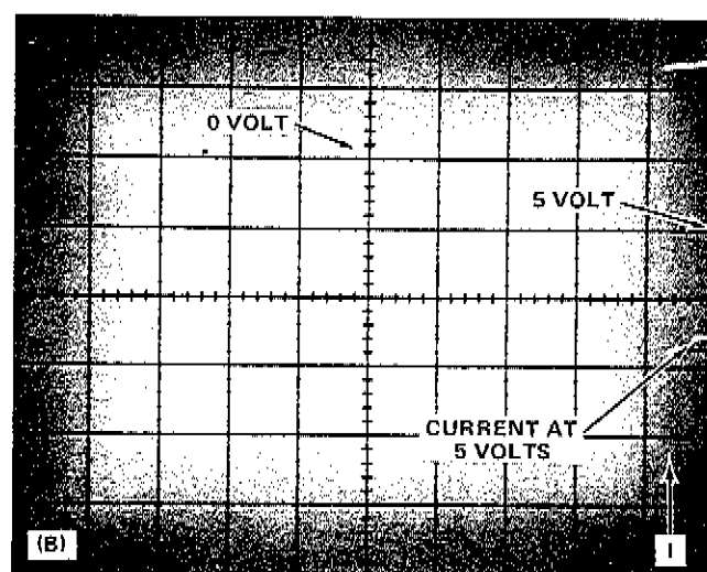
Fig. 5-3. Typical displays of Step Generator current at maximum voltage. (A) Illustrating step k and (B) illustrating step m.
