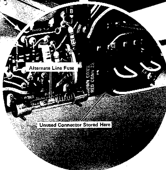
Fig. 4-1. Power transformer line-voltage taps.
