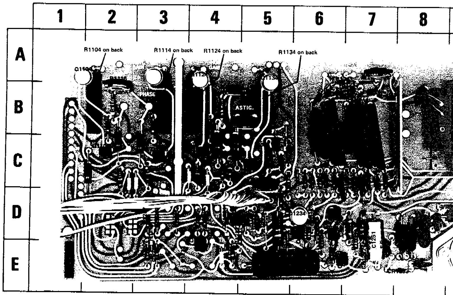
Fig. 7-17. A5 Deflection Amplifier/High Voltage circuit board.
