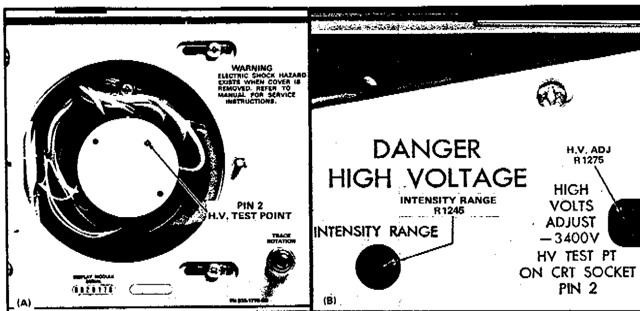
Fig. 7-2. Location of (A) CRT socket access and (B) R1275, H V Adj R1245, Intensity Range.
