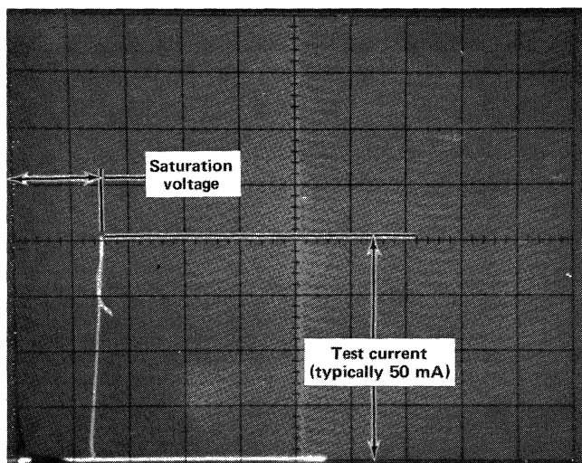
Fig. 22. Typical display of Emitter Saturation Voltage V_{EB_1(SAT)} .
