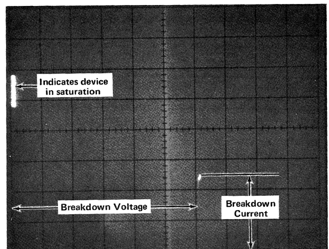
Fig. 17. Typical display of V_{(BR)CEO} for current values in excess of 1 mA.
