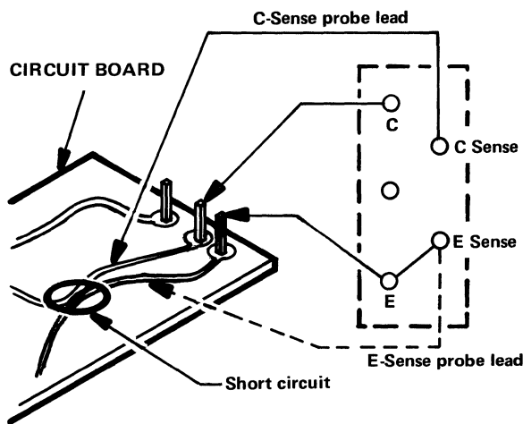
Fig. 43. Connecting the C-sense lead for short-circuit location.
