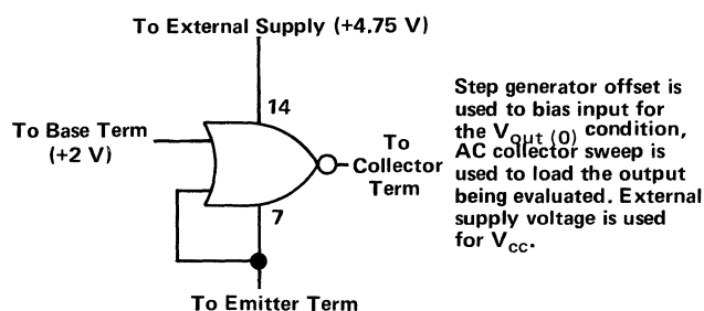
Fig. 53. TTL evaluation, V_{out}(0) condition.
