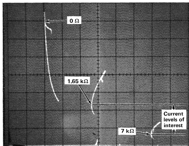
Fig. 24. Stored display of the effect of resistance in series with the unijunction emitter.
