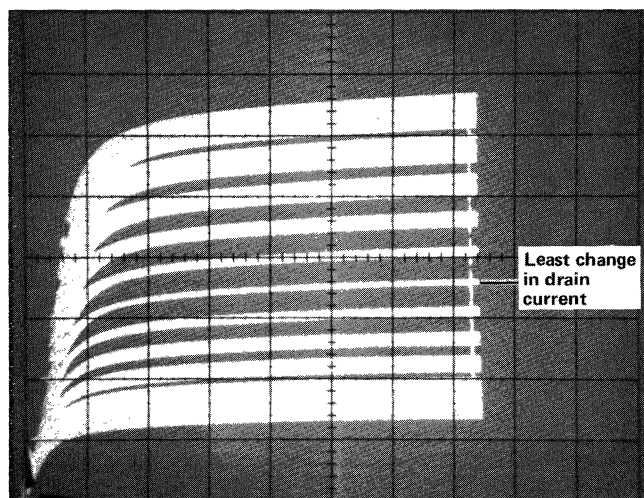
Fig. 21. Display of changes in drain current characteristics with temperature changes. Stored display clearly shows level of least change in drain current.
