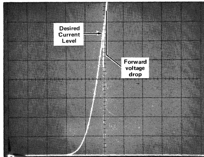
Fig. 26. SCR Forward voltage drop.
