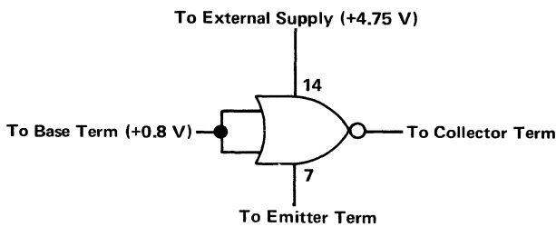
Fig. 55. TTL evaluation, Short-Circuit Output Current I_{OS} .
