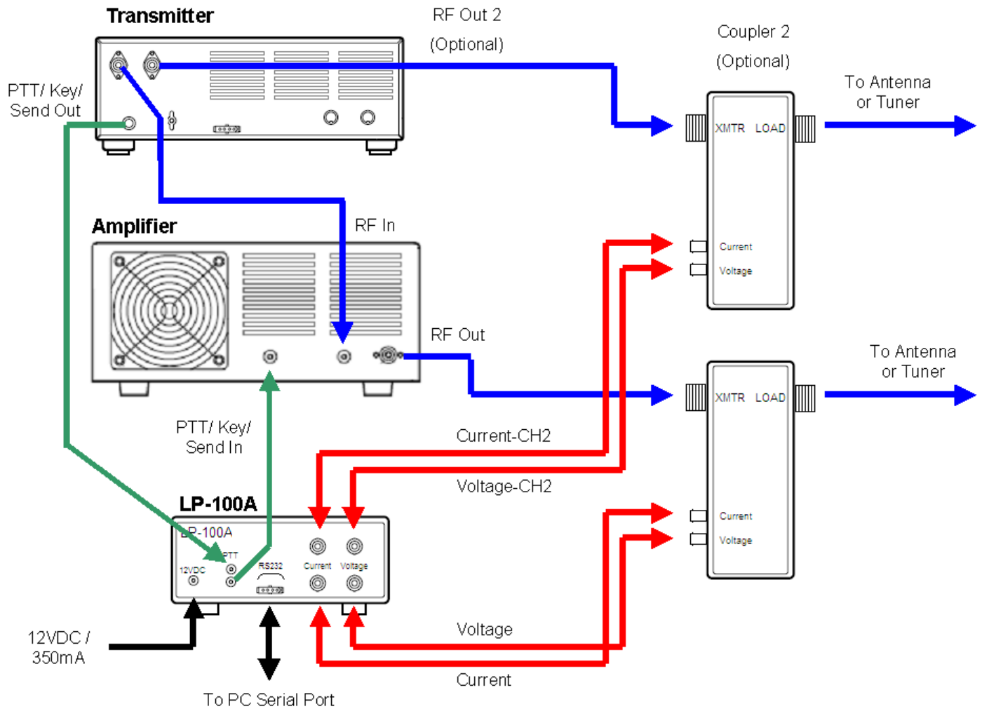
Fig.1. Shows installation with dual coupler option installed and transmitter with two ANT jacks. Ignore 2 nd coupler and its connections for a standard single coupler installation. Current cables are marked with red band (2 red bands for 2 nd coupler).
