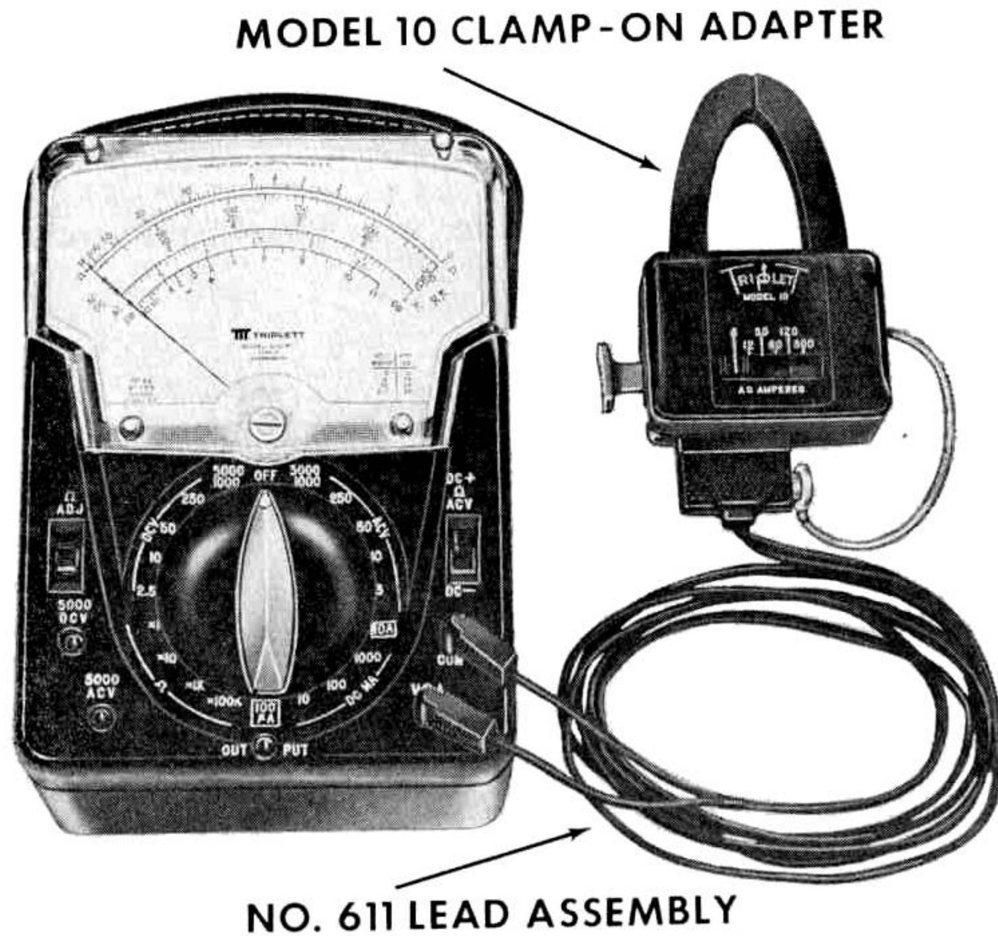
Fig. 8. Model 10 Clamp-On-Adapter.
