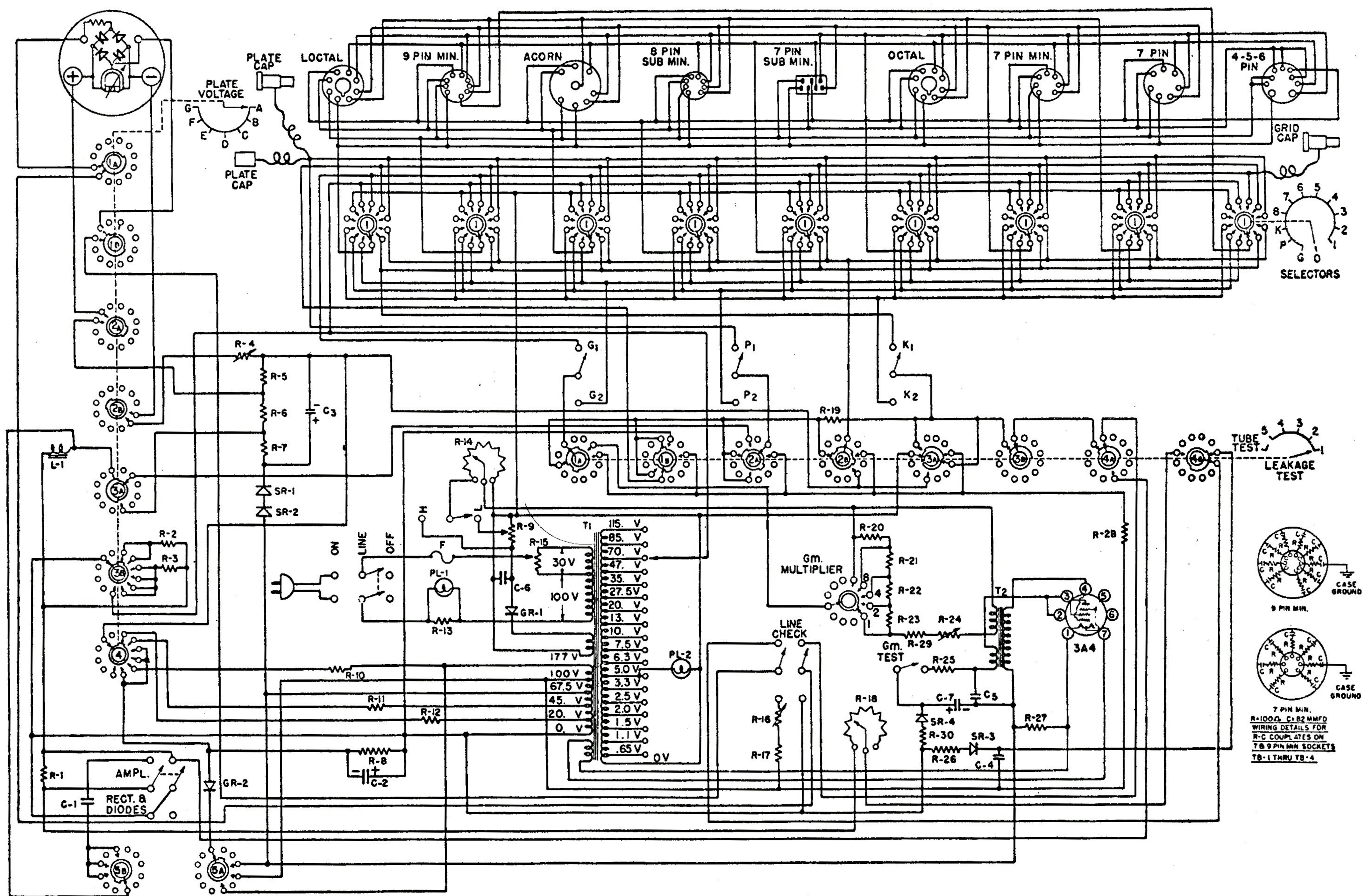
Schematic Wiring Diagram — Model 981 Type 3
