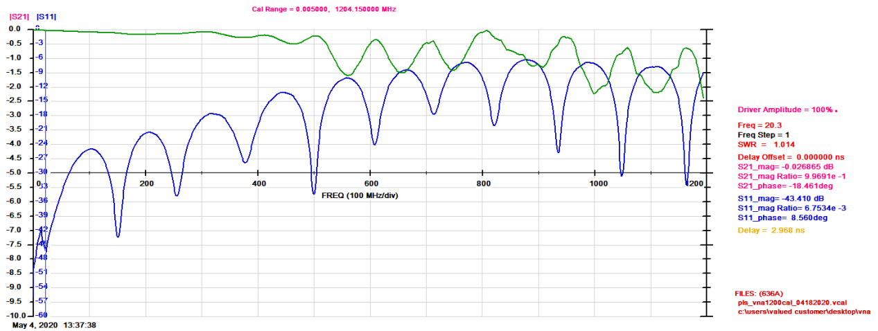
Figure 7: Baseline data for Splice test (cable 3)
