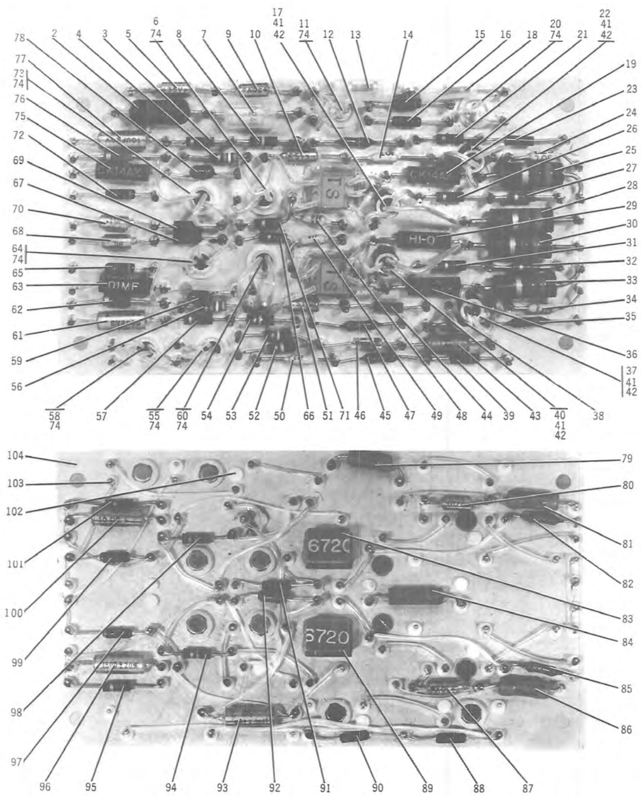
Figure 6-6. Electronic Components Assembly.
