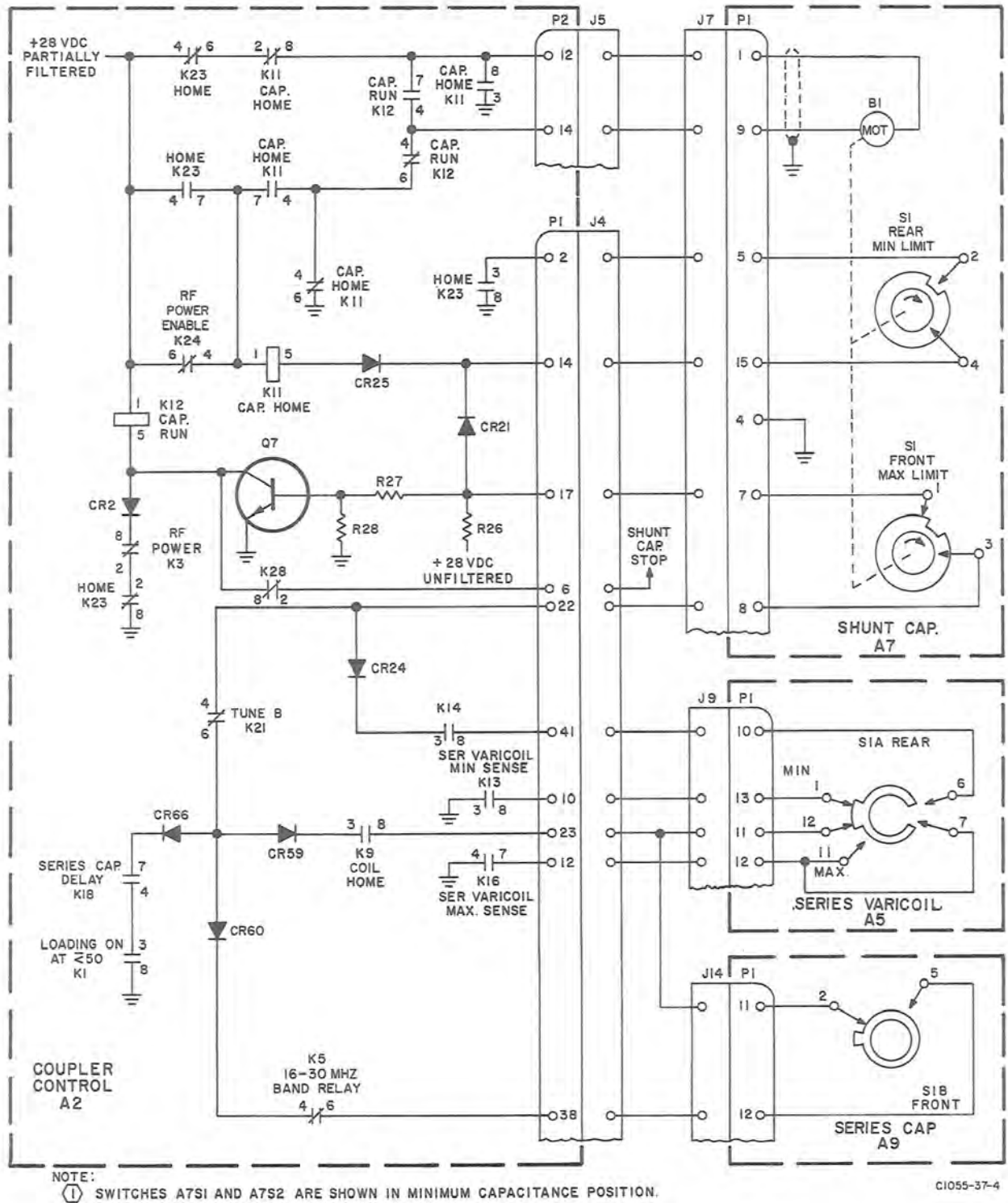
Figure 4-5. Shunt Capacitor Motor Circuit, Simplified Schematic Diagram.
