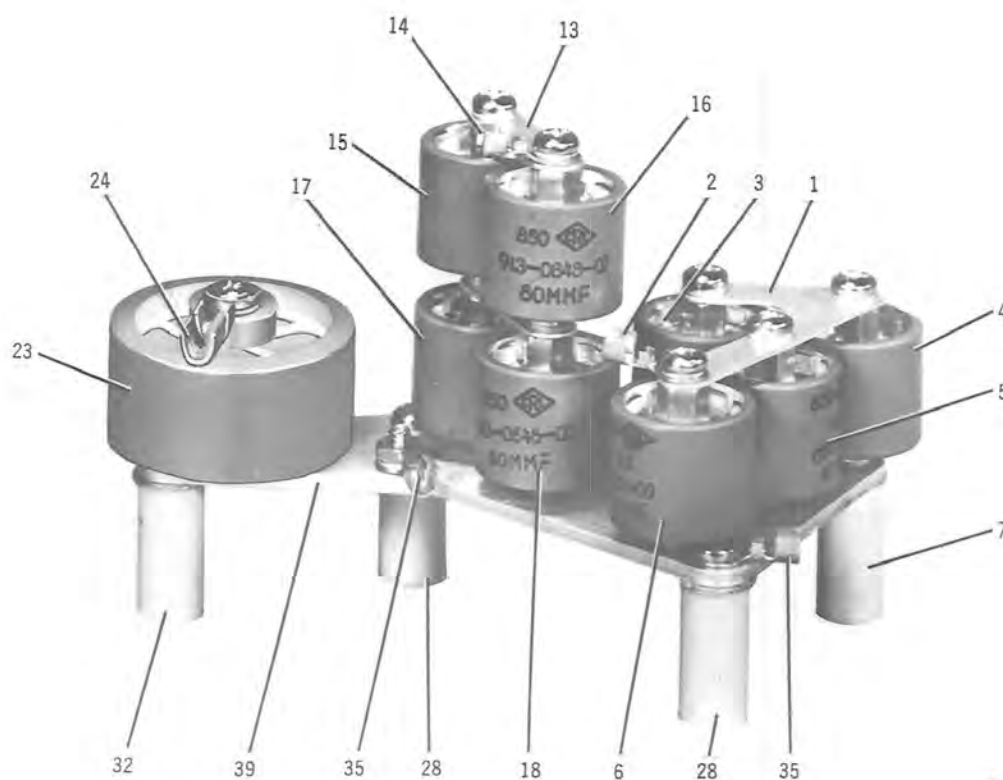
Figure 6-13. Capacitor Assembly.
