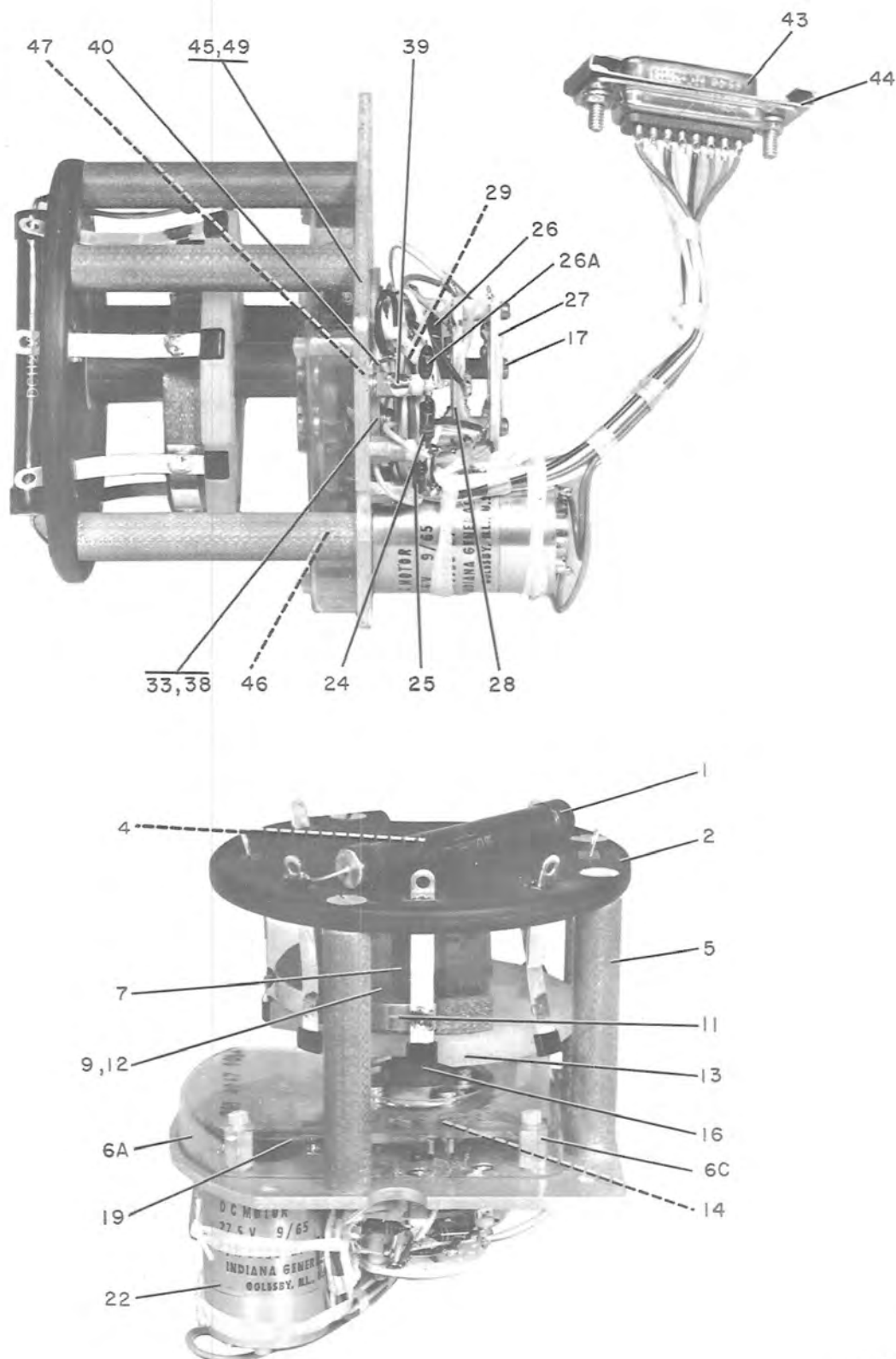
Figure 6-14. Rotary Switch.
