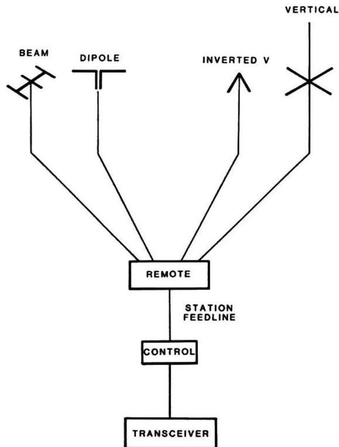
BLOCK DIAGRAM
