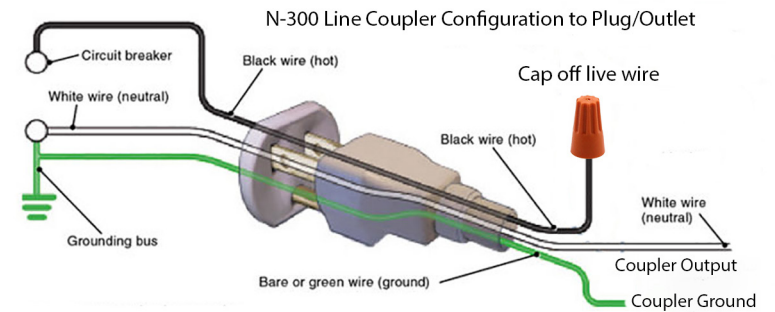
Line Coupler Configuration
