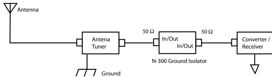
Ground Isolator Configuration
