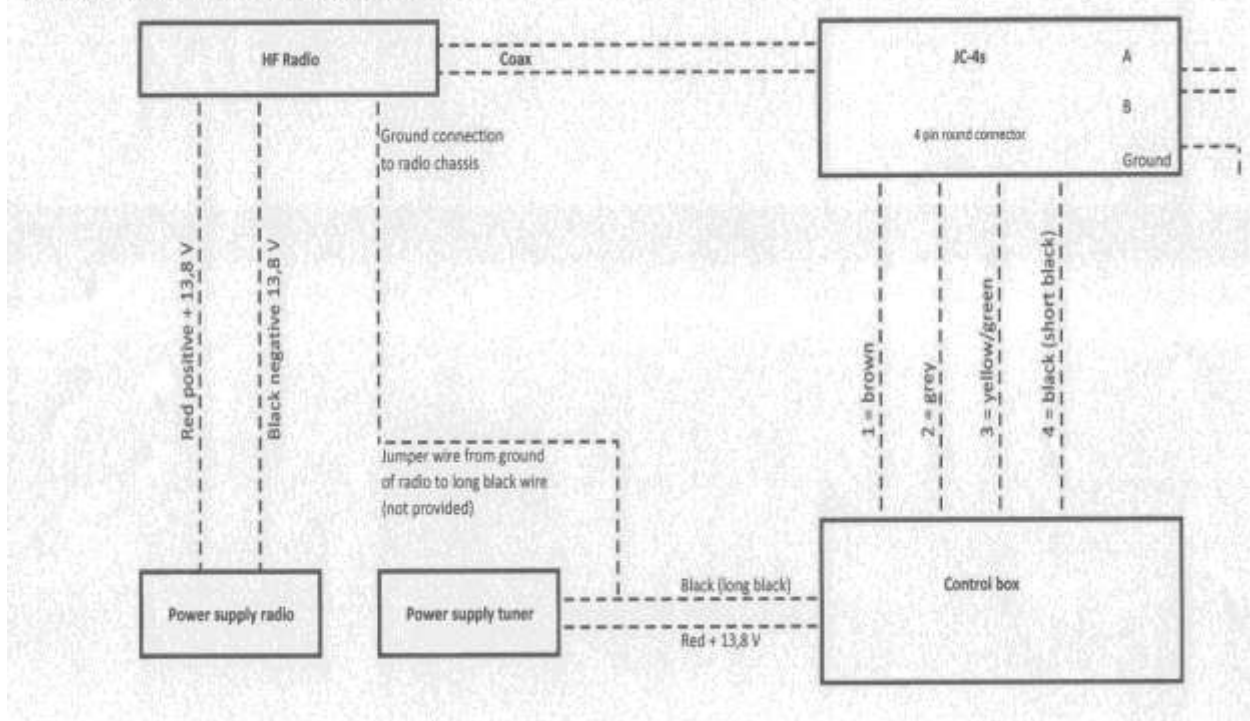
Wiring diagram control box with 2 separately power supplies
