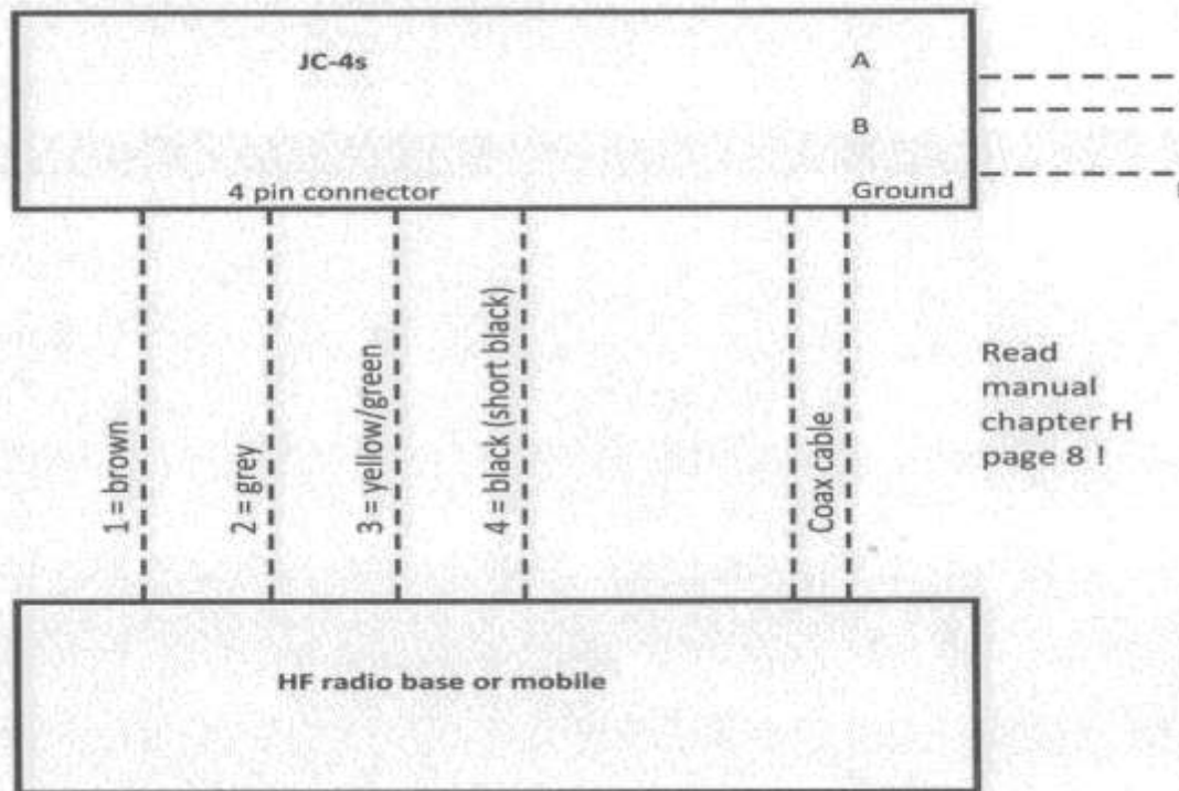
Wiring diagram Radio to JC-4 without control box
