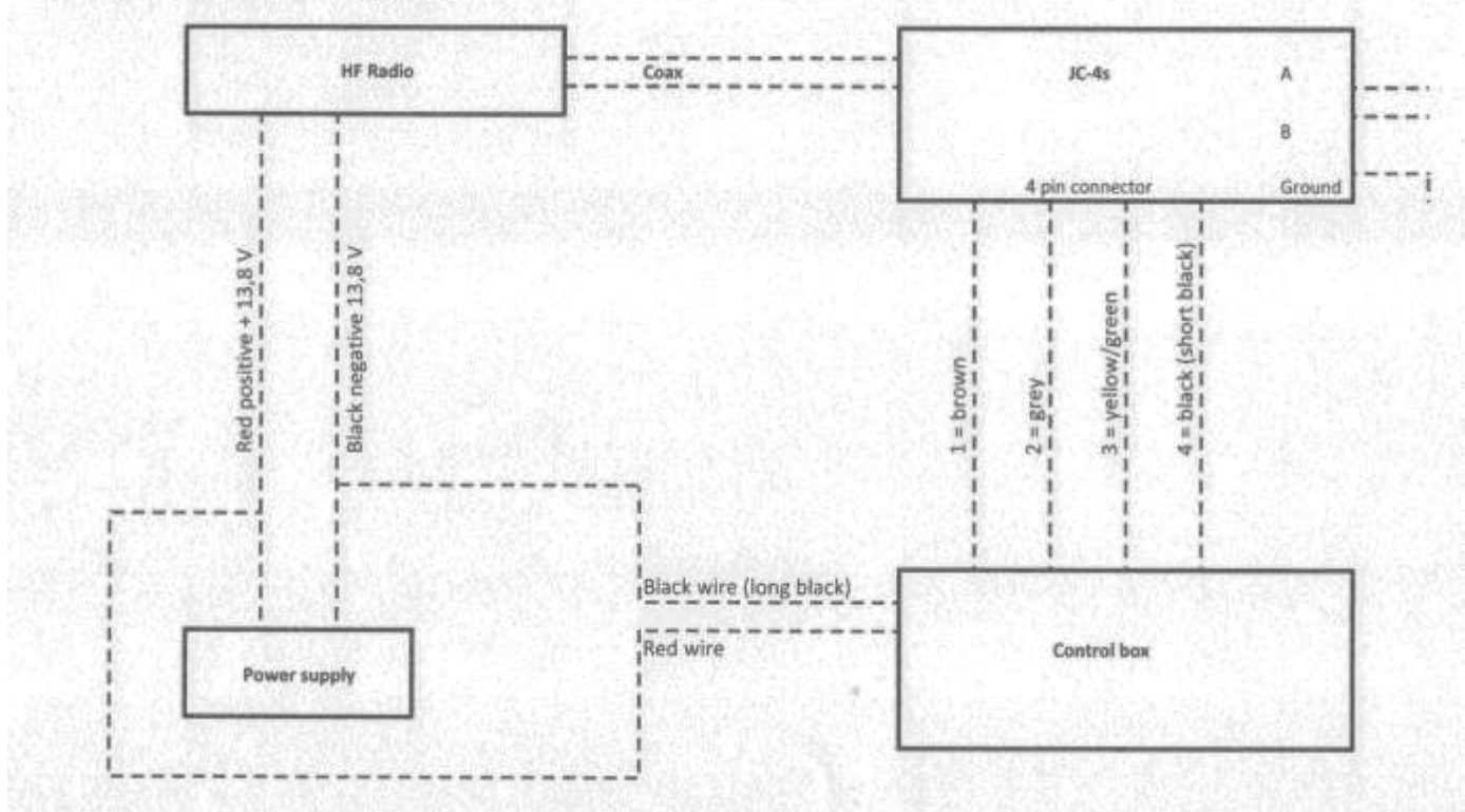
Wiring diagram control box with 1 power supply
