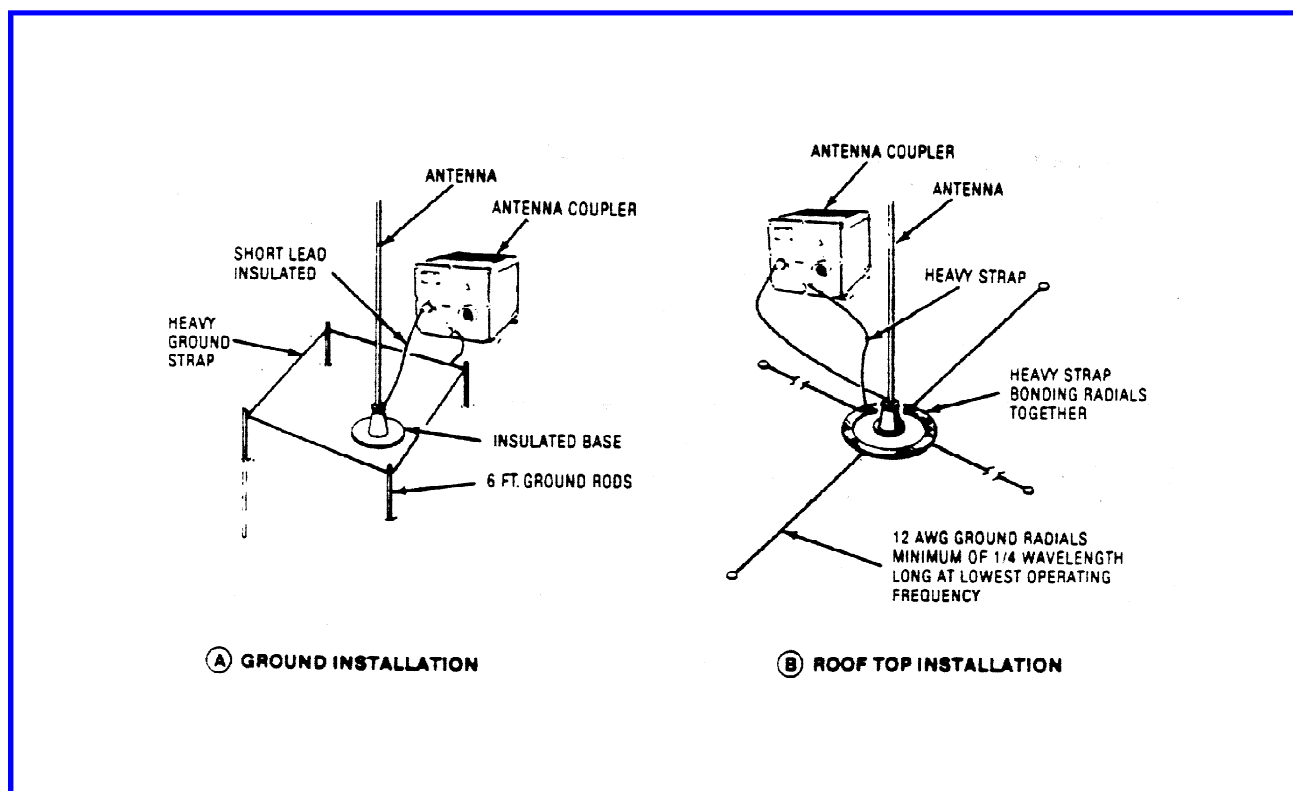
Figure 2.6 Whip Antenna.
