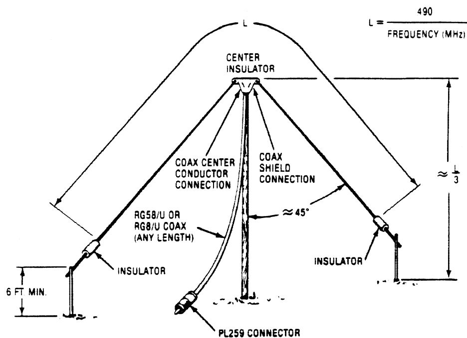
Figure 2.7 Inverted 'V' Antenna.
