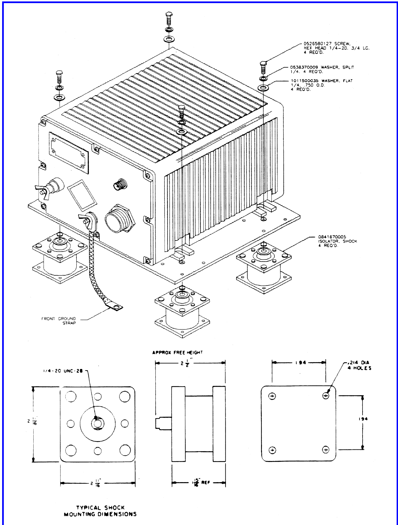
Figure 2.2 Shockmount Installation.
