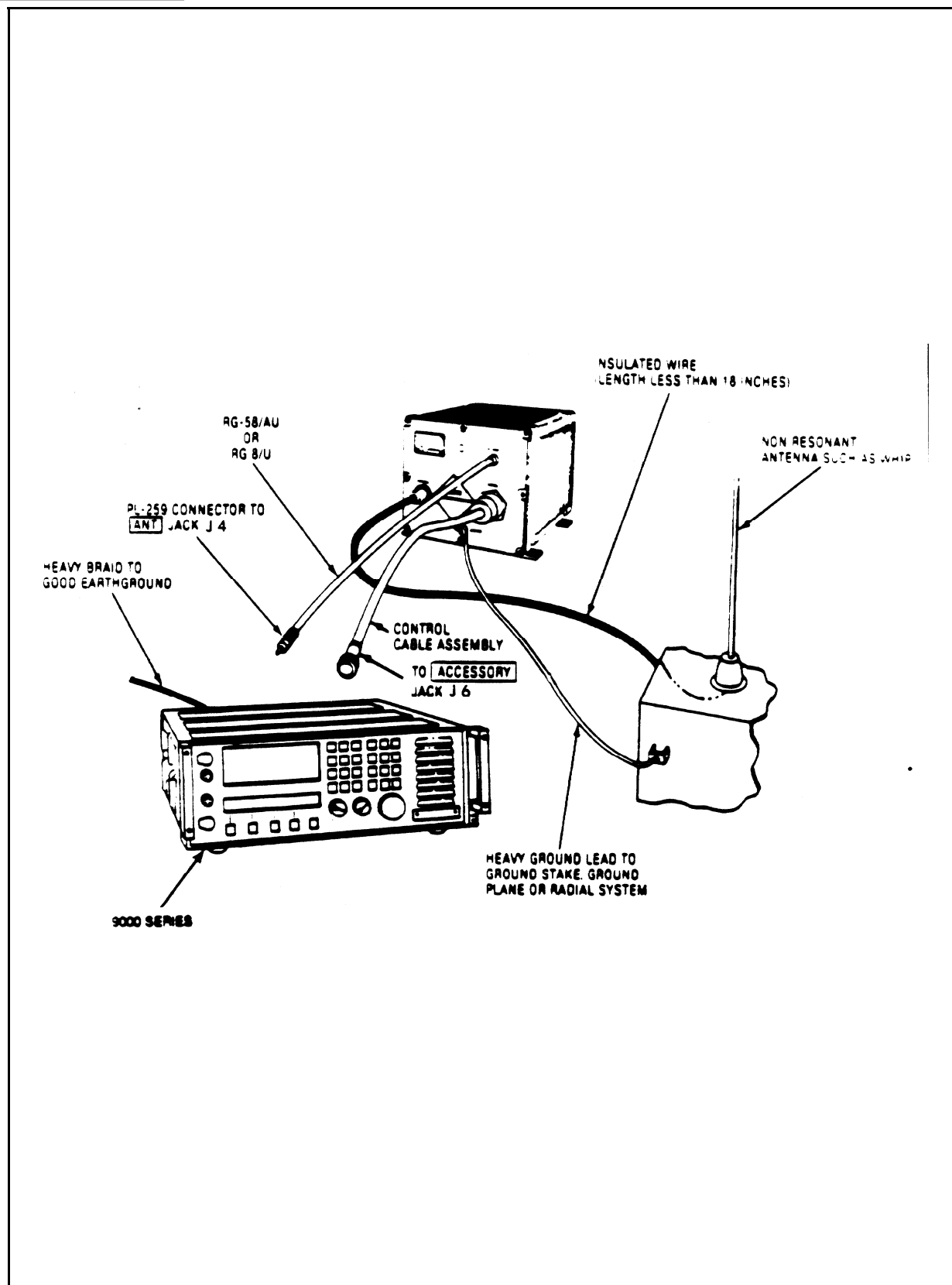
Figure 2.3 Typical Base Station Installation Using Non-Resonant Antennas.
