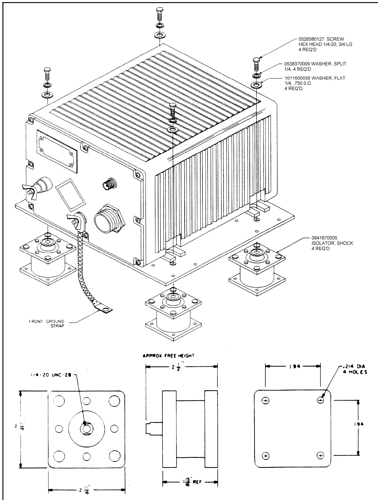
Figure 2.2 Shockmount Installation.
