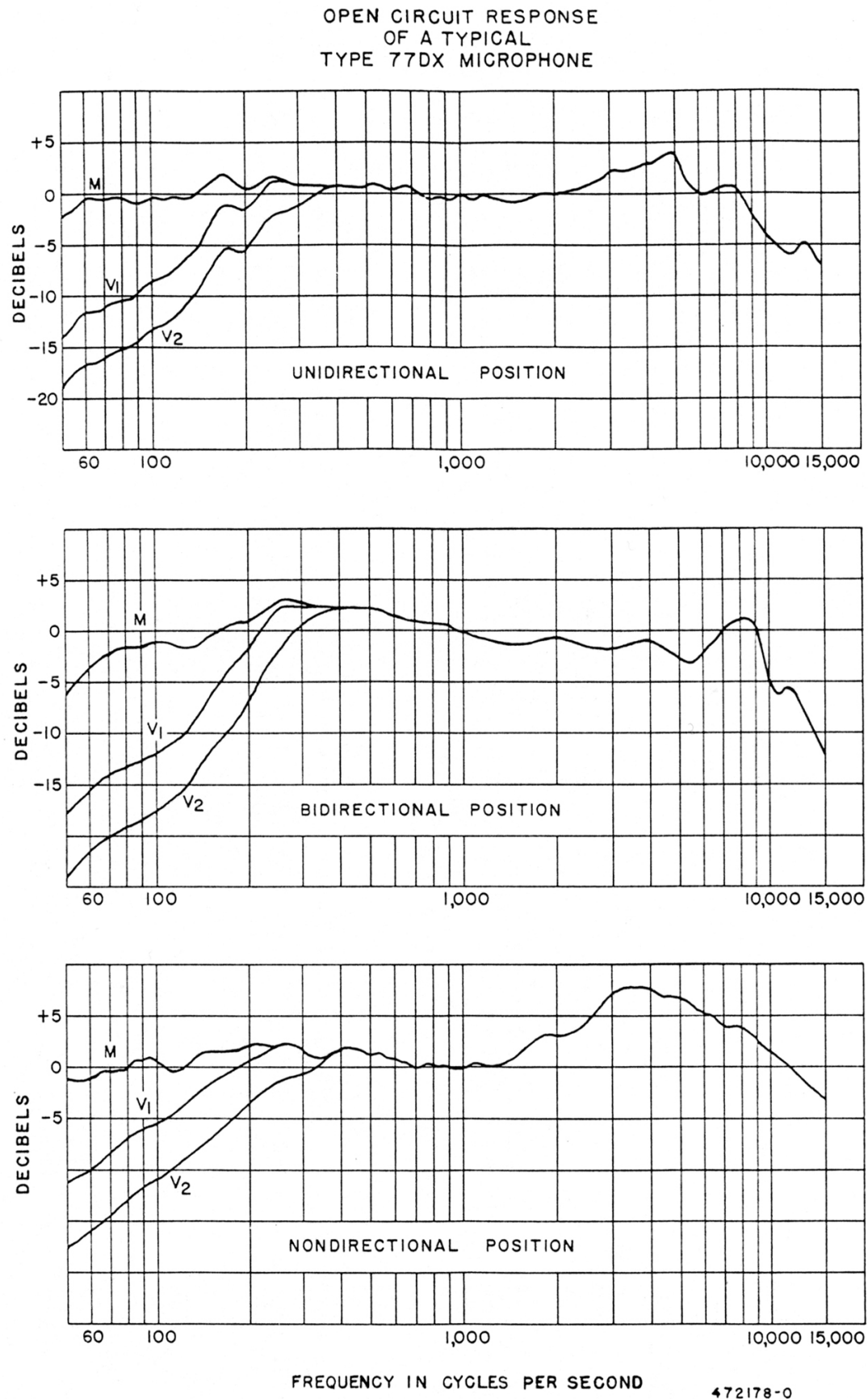
Figure 5 - Frequency Response Curves
