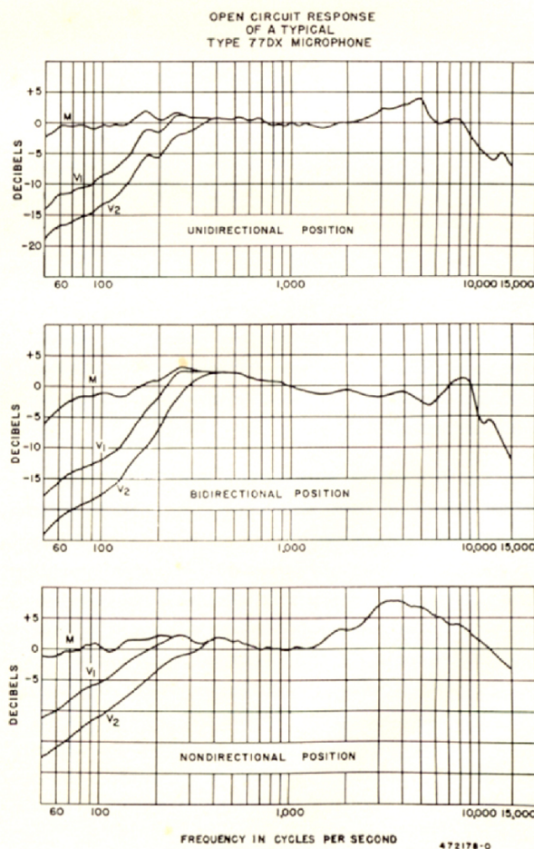
Typical Directional Patterns and Frequency Response Curves of 77-DX Polydirectional Microphone
