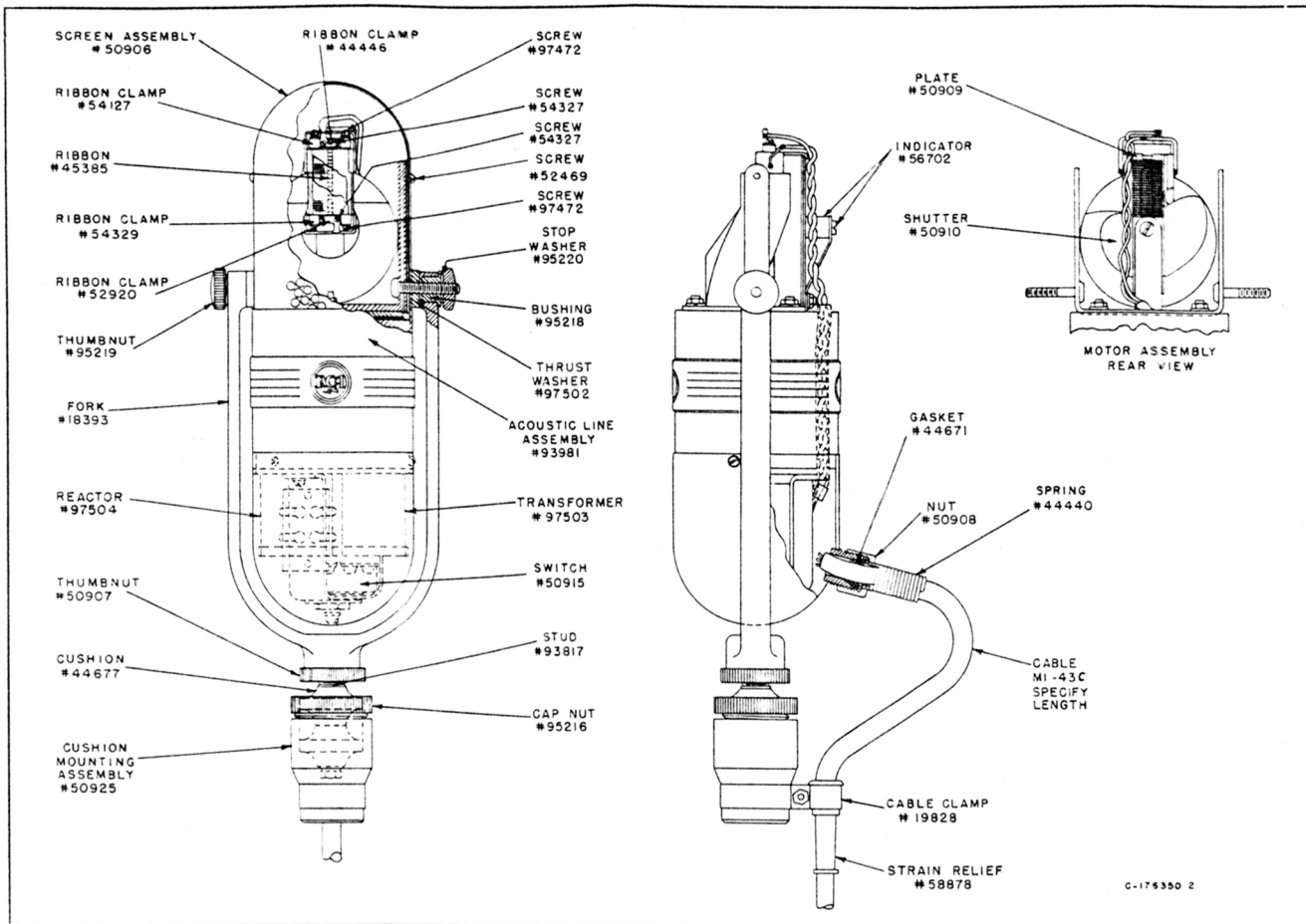
Figure 6 - Parts Location Diagram of MI-4045-F
