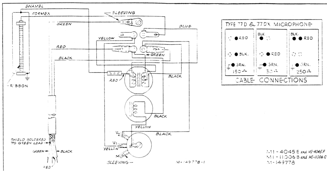
Figure 3 - Schematic and Connection Diagram
